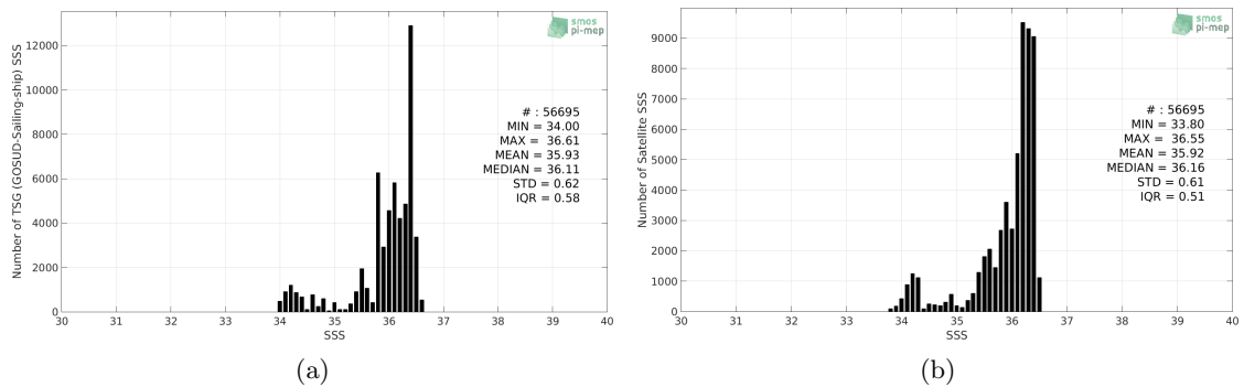
Figure 2: Histograms of SSS from TSG (GOSUD-Sailing-ship) (a) and CCI SSS L4 Merged-OI v3.2 - 7-day running (ESA) (b) considering all match-up pairs per bins of 0.1 over the OTT zone Pi-MEP region and for the full satellite product period.
