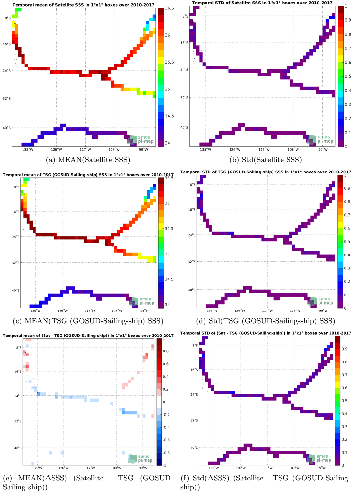
Figure 6: Temporal mean (left) and Std (right) of SSS from CCI SSS L4 Merged-OI v3.2 - 7-day running (ESA) (top), TSG (GOSUD-Sailing-ship) (middle), and of \Delta SSS (Satellite - TSG (GOSUD-Sailing-ship)). Only match-up pairs are used to generate these maps.
