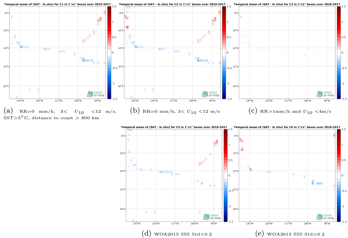
Figure 12: Temporal mean gridded over spatial boxes of size 1^\circ \times 1^\circ of \Delta\text{SSS} (CCI SSS L4 Merged-OI v3.2 - 7-day running (ESA) - TSG (GOSUD-Sailing-ship)) for 5 different subdatasets corresponding to:RR=0 mm/h, 3 < U_{10} < 12 m/s, SST>5°C, distance to coast > 800 km (a), RR=0 mm/h, 3 < U_{10} < 12 m/s (b), RR>1mm/h and U_{10} < 4 m/s (c), WOA2013 SSS Std<0.2 (d), WOA2013 SSS Std>0.2 (e).
