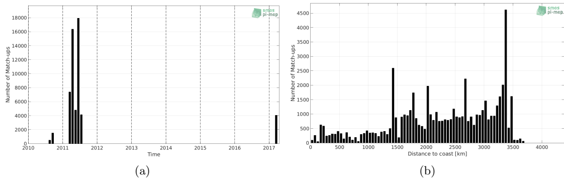
Figure 1: Number of match-ups between TSG (GOSUD-Sailing-ship) and CCI SSS L4 Merged-OI v3.2 - 7-day running (ESA) SSS as a function of time (a) and as function of the distance to coast (b) over the OTT zone Pi-MEP region and for the full satellite product period.
