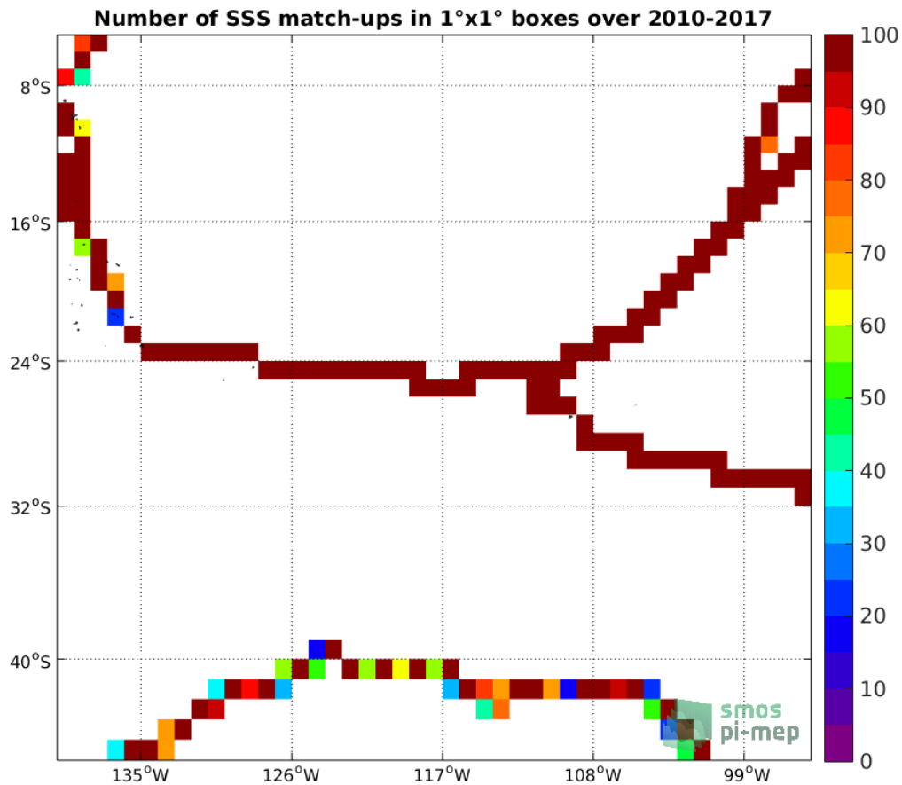
Figure 4: Number of SSS match-ups between TSG (GOSUD-Sailing-ship) SSS and the CCI SSS L4 Merged-OI v3.2 - 7-day running (ESA) SSS product for the OTT zone Pi-MEP region over 1°x1° boxes and for the full satellite product period.
