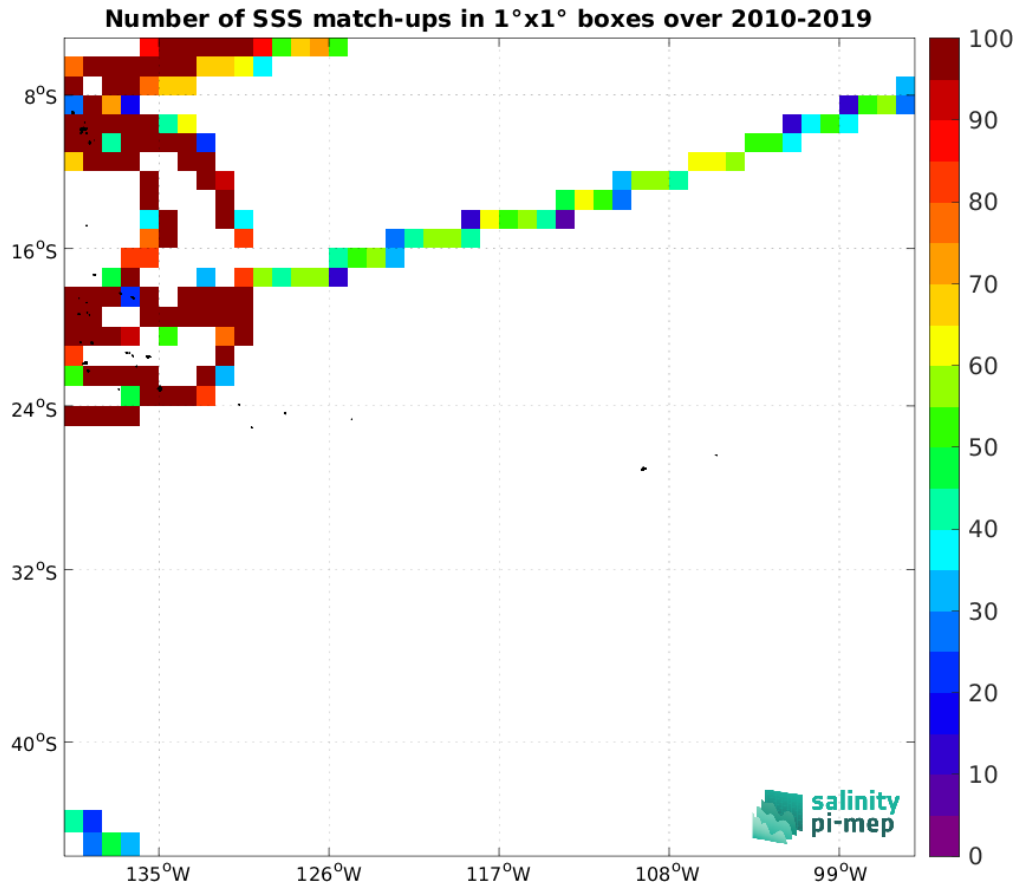
Figure 4: Number of SSS match-ups between TSG (GOSUD-Research-vessel) SSS and the CCI SSS L4 Merged-OI v3.2 - 7-day running (ESA) SSS product for the OTT zone Pi-MEP region over 1^\circ \times 1^\circ boxes and for the full satellite product period.
