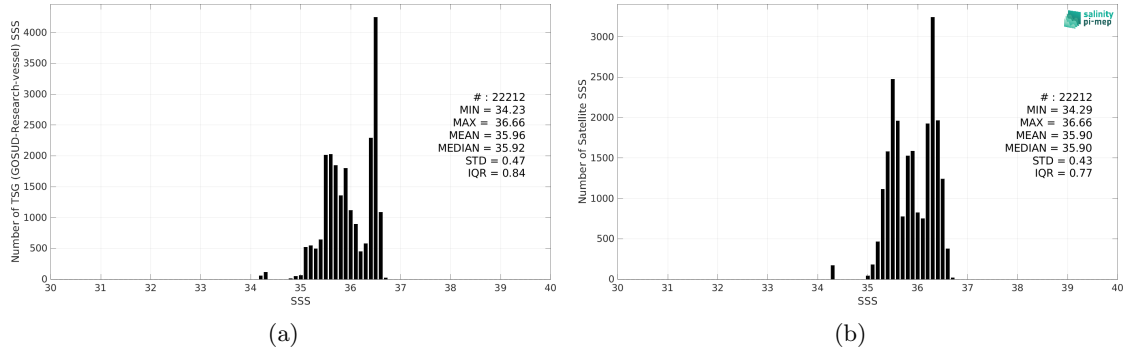
Figure 2: Histograms of SSS from TSG (GOSUD-Research-vessel) (a) and CCI SSS L4 Merged-OI v3.2 - 7-day running (ESA) (b) considering all match-up pairs per bins of 0.1 over the OTT zone Pi-MEP region and for the full satellite product period.
