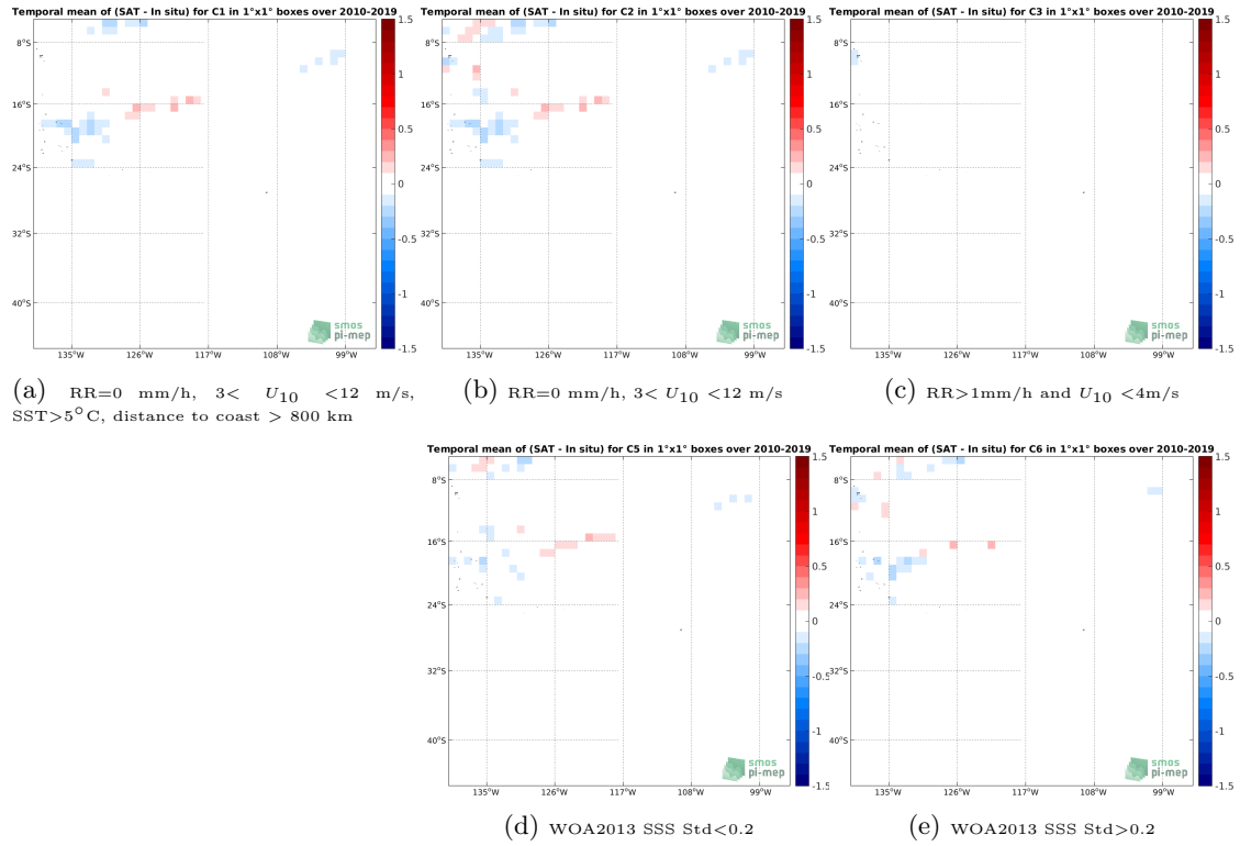
Figure 12: Temporal mean gridded over spatial boxes of size 1^\circ \times 1^\circ of \Delta SSS (CCI SSS L4 Merged-OI v3.2 - 7-day running (ESA) - TSG (GOSUD-Research-vessel)) for 5 different subdatasets corresponding to: RR=0 mm/h, 3 < U_{10} < 12 m/s, SST > 5^\circ C , distance to coast > 800 km (a), RR=0 mm/h, 3 < U_{10} < 12 m/s (b), RR > 1 mm/h and U_{10} < 4 m/s (c), WOA2013 SSS Std < 0.2 (d), WOA2013 SSS Std > 0.2 (e).
