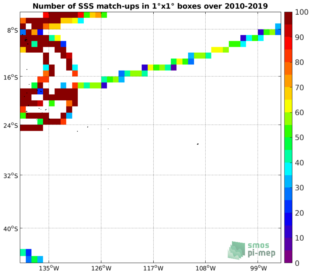
Figure 4: Number of SSS match-ups between TSG (GOSUD-Research-vessel) SSS and the CCI SSS L4 Merged-OI v3.2 - 7-day running (ESA) SSS product for the OTT zone Pi-MEP region over 1°x1° boxes and for the full satellite product period.
