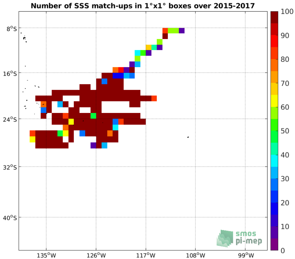
Figure 3: Number of SSS match-ups between Surface drifters SSS and the CCI SSS L4 Merged-OI v3.2 - 7-day running (ESA) SSS product for the OTT zone Pi-MEP region over 1^{\circ} \times 1^{\circ} boxes and for the full satellite product period.
