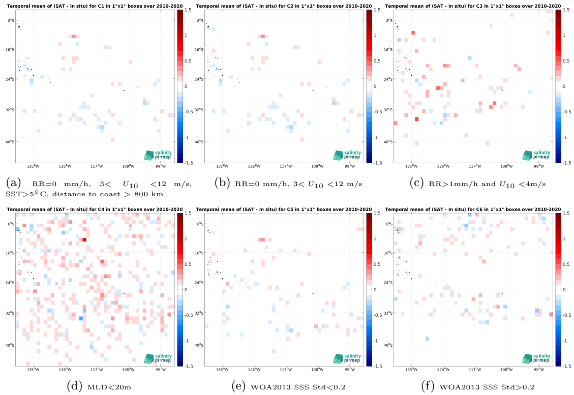
Figure 12: Temporal mean gridded over spatial boxes of size 1^\circ \times 1^\circ of \Delta SSS (CCI SSS L4 Merged-OI v3.2 - 7-day running (ESA) - Argo) for 6 different subdatasets corresponding to:RR=0 mm/h, 3 < U_{10} < 12 m/s, SST >5^\circ C, distance to coast > 800 km (a), RR=0 mm/h, 3 < U_{10} < 12 m/s (b), RR >1 mm/h and U_{10} < 4 m/s (c),MLD <20 m (d),WOA2013 SSS Std <0.2 (e),WOA2013 SSS Std >0.2 (f).
