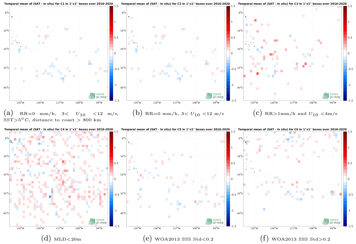
Figure 12: Temporal mean gridded over spatial boxes of size 1^\circ \times 1^\circ of \Delta SSS (CCI SSS L4 Merged-OI v3.2 - 7-day running (ESA) - Argo) for 6 different subdatasets corresponding to:RR=0 mm/h, 3 < U_{10} < 12 m/s, SST > 5^\circ\text{C} , distance to coast > 800 km (a), RR=0 mm/h, 3 < U_{10} < 12 m/s (b), RR > 1 mm/h and U_{10} < 4 m/s (c),MLD < 20 m (d),WOA2013 SSS Std < 0.2 (e),WOA2013 SSS Std > 0.2 (f).
