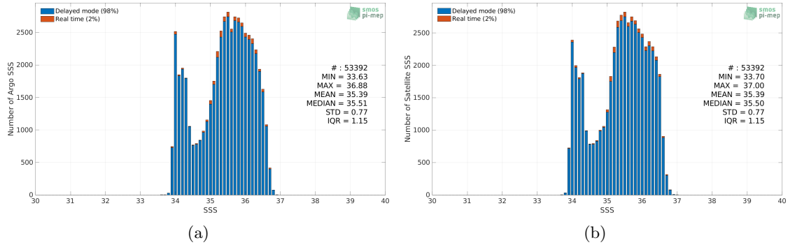
Figure 2: Histograms of SSS from Argo (a) and CCI SSS L4 Merged-OI v3.2 - 7-day running (ESA) (b) considering all match-up pairs per bins of 0.1 over the OTT zone Pi-MEP region and for the full satellite product period.
