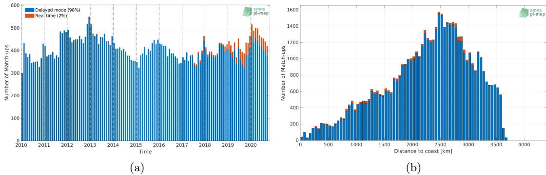
Figure 1: Number of match-ups between Argo and CCI SSS L4 Merged-OI v3.2 - 7-day running (ESA) SSS as a function of time (a) and as function of the distance to coast (b) over the OTT zone Pi-MEP region and for the full satellite product period.
