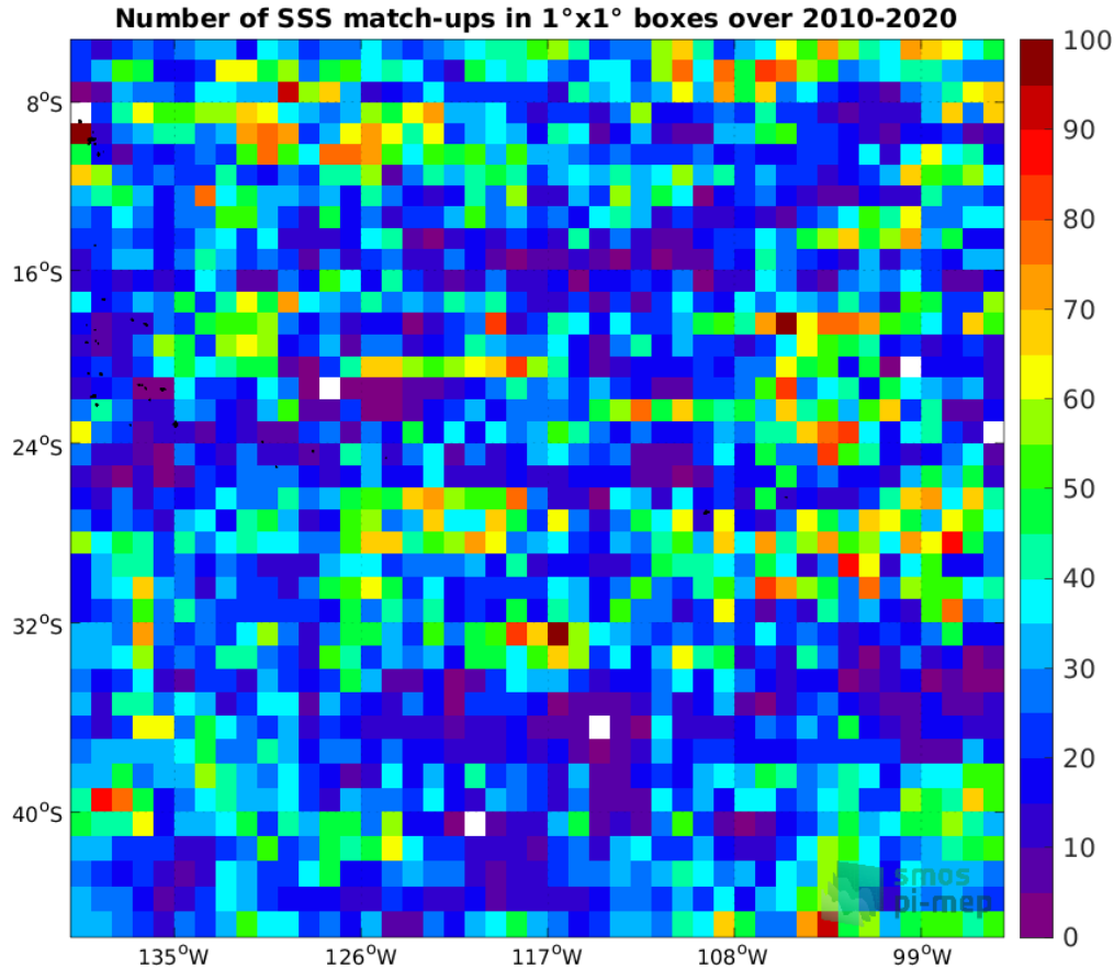
Figure 4: Number of SSS match-ups between Argo SSS and the CCI SSS L4 Merged-OI v3.2 - 7-day running (ESA) SSS product for the OTT zone Pi-MEP region over 1^\circ \times 1^\circ boxes and for the full satellite product period.
