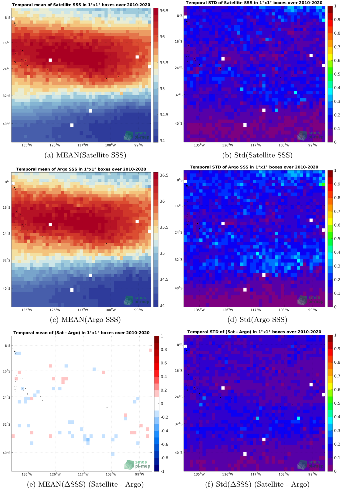
Figure 6: Temporal mean (left) and Std (right) of SSS from CCI SSS L4 Merged-OI v3.2 - 7-day running (ESA) (top), Argo (middle), and of \Delta SSS (Satellite - Argo). Only match-up pairs are used to generate these maps.
