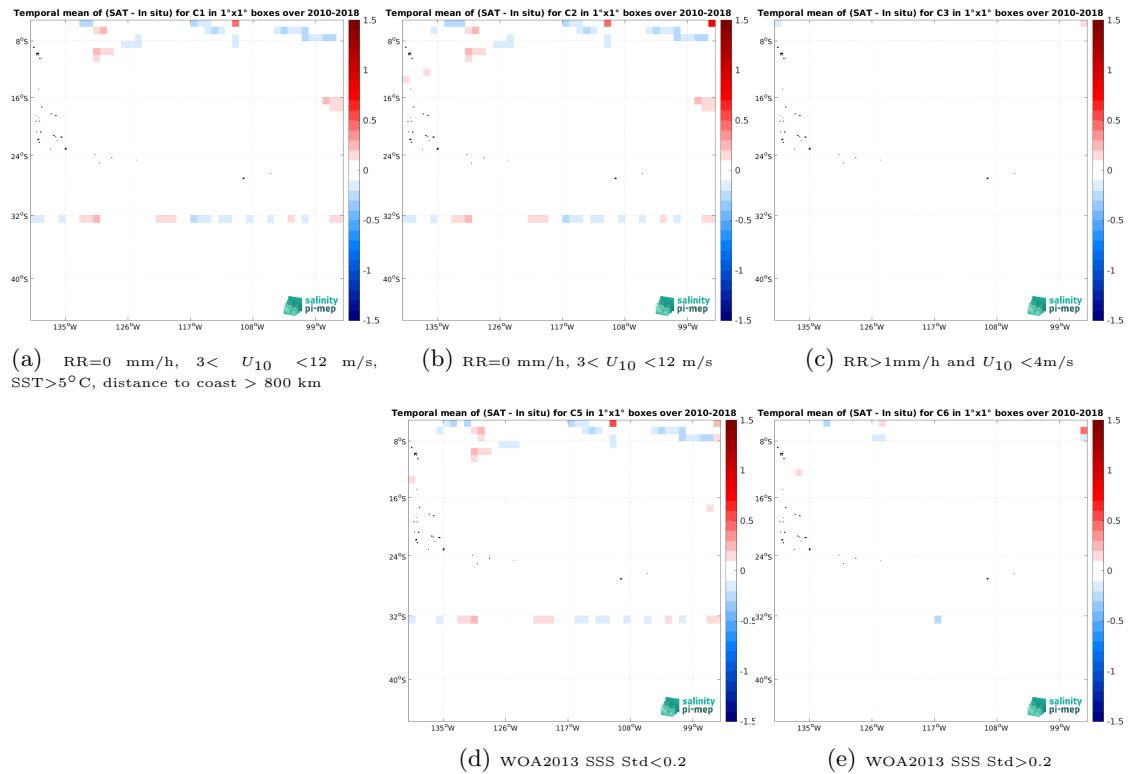
Figure 12: Temporal mean gridded over spatial boxes of size 1^\circ \times 1^\circ of \Delta\text{SSS} (CCI SSS L4 Merged-OI v3.2 - 30-day running (ESA) - TSG (SAMOS)) for 5 different subdatasets corresponding to: \text{RR}=0 mm/h, 3 < U_{10} < 12 m/s, \text{SST} > 5^\circ\text{C} , distance to coast > 800 km (a), \text{RR}=0 mm/h, 3 < U_{10} < 12 m/s (b), \text{RR} > 1\text{mm/h} and U_{10} < 4\text{m/s} (c), WOA2013 SSS Std < 0.2 (d), WOA2013 SSS Std > 0.2 (e).
