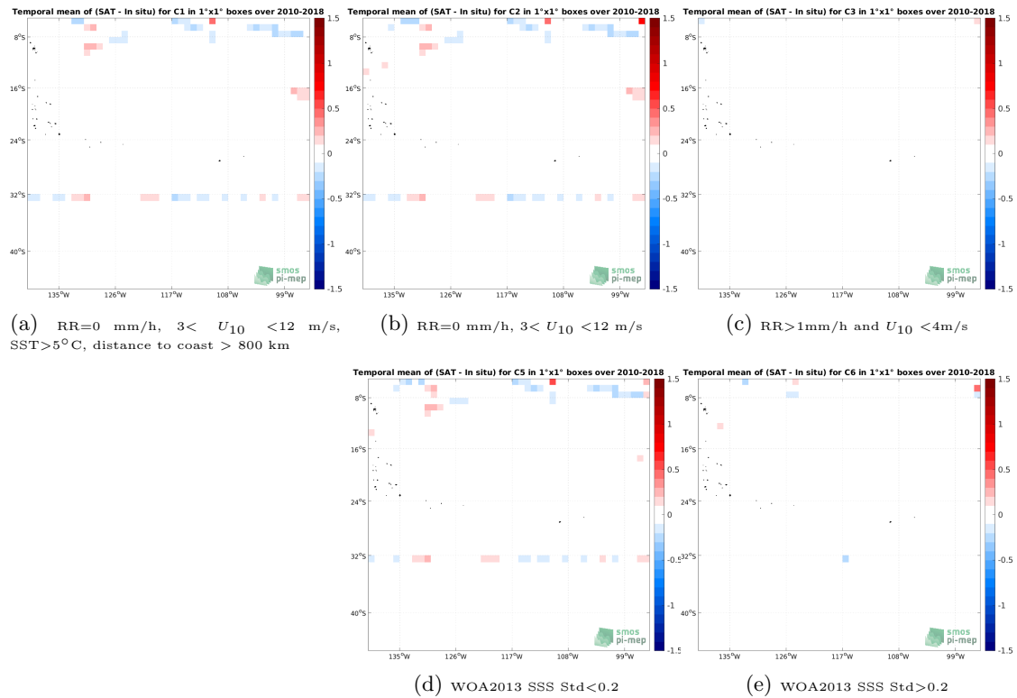
Figure 12: Temporal mean gridded over spatial boxes of size 1^\circ \times 1^\circ of \Delta SSS (CCI SSS L4 Merged-OI v3.2 - 30-day running (ESA) - TSG (SAMOS)) for 5 different subdatasets corresponding to:RR=0 mm/h, 3 < U_{10} < 12 m/s, SST >5^\circ C, distance to coast > 800 km (a), RR=0 mm/h, 3 < U_{10} < 12 m/s (b), RR >1 mm/h and U_{10} < 4 m/s (c), WOA2013 SSS Std <0.2 (d), WOA2013 SSS Std >0.2 (e).
