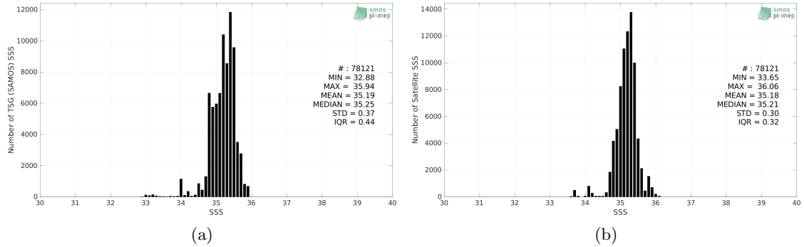
Figure 2: Histograms of SSS from TSG (SAMOS) (a) and CCI SSS L4 Merged-OI v3.2 - 30-day running (ESA) (b) considering all match-up pairs per bins of 0.1 over the OTT zone Pi-MEP region and for the full satellite product period.
