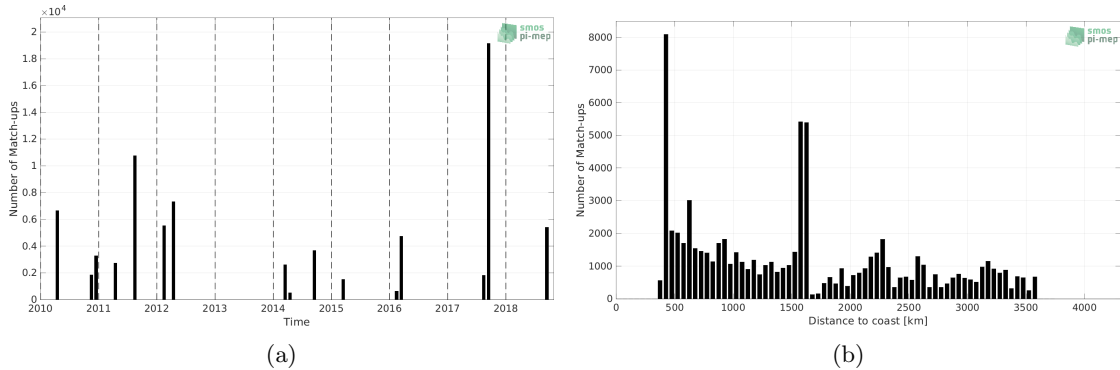
Figure 1: Number of match-ups between TSG (SAMOS) and CCI SSS L4 Merged-OI v3.2 - 30-day running (ESA) SSS as a function of time (a) and as function of the distance to coast (b) over the OTT zone Pi-MEP region and for the full satellite product period.
