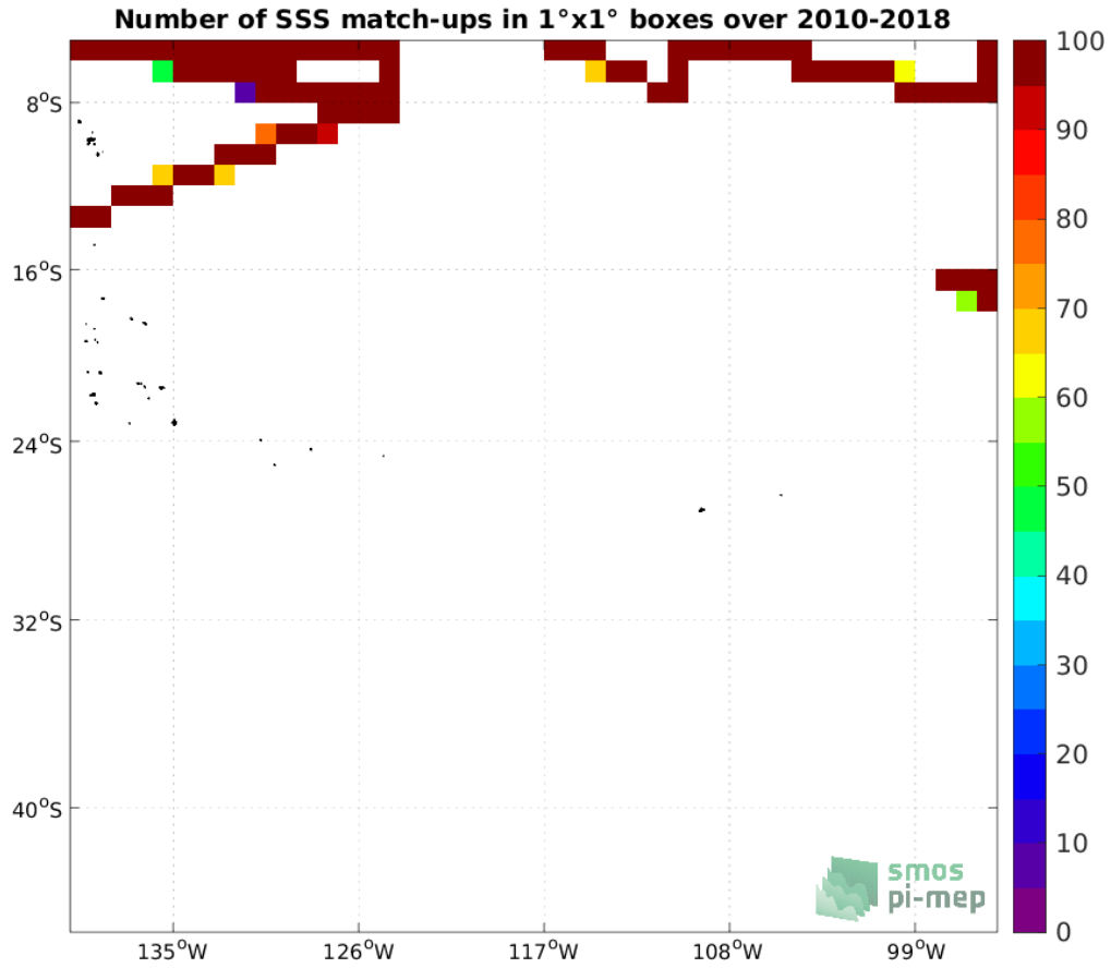
Figure 4: Number of SSS match-ups between TSG (SAMOS) SSS and the CCI SSS L4 Merged-OI v3.2 - 30-day running (ESA) SSS product for the OTT zone Pi-MEP region over 1^\circ \times 1^\circ boxes and for the full satellite product period.
