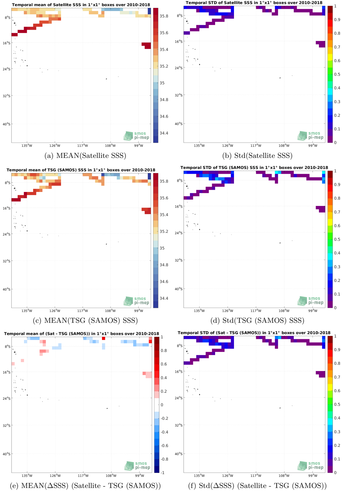
Figure 6: Temporal mean (left) and Std (right) of SSS from CCI SSS L4 Merged-OI v3.2 - 30-day running (ESA) (top), TSG (SAMOS) (middle), and of \Delta SSS (Satellite - TSG (SAMOS)). Only match-up pairs are used to generate these maps.
