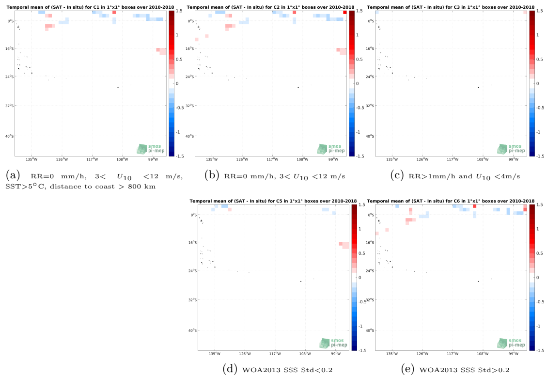
Figure 12: Temporal mean gridded over spatial boxes of size 1^\circ \times 1^\circ of \Delta SSS (CCI SSS L4 Merged-OI v3.2 - 30-day running (ESA) - TSG (SAMOS)) for 5 different subdatasets corresponding to:RR=0 mm/h, 3 < U_{10} < 12 m/s, SST >5^\circ C, distance to coast > 800 km (a), RR=0 mm/h, 3 < U_{10} < 12 m/s (b), RR >1 mm/h and U_{10} < 4 m/s (c), WOA2013 SSS Std <0.2 (d), WOA2013 SSS Std >0.2 (e).
