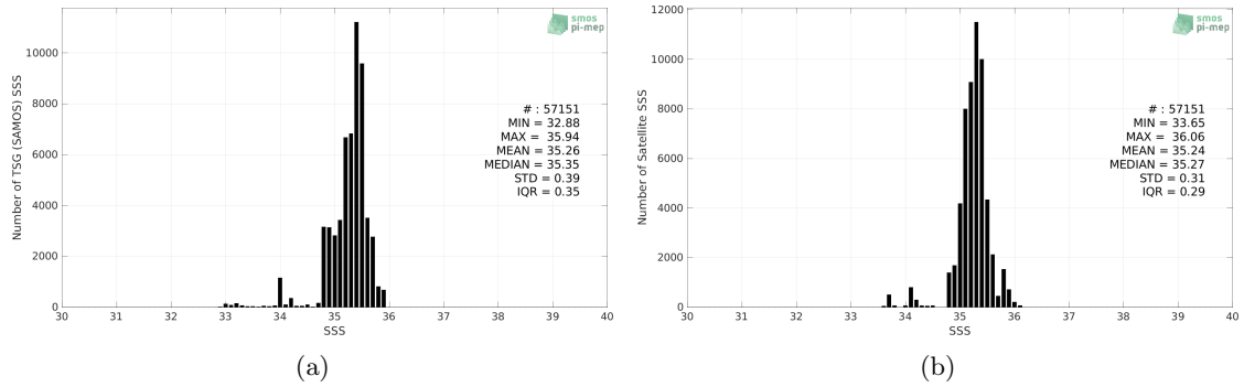
Figure 2: Histograms of SSS from TSG (SAMOS) (a) and CCI SSS L4 Merged-OI v3.2 - 30-day running (ESA) (b) considering all match-up pairs per bins of 0.1 over the OTT zone Pi-MEP region and for the full satellite product period.
