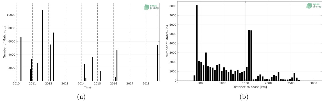
Figure 1: Number of match-ups between TSG (SAMOS) and CCI SSS L4 Merged-OI v3.2 - 30-day running (ESA) SSS as a function of time (a) and as function of the distance to coast (b) over the OTT zone Pi-MEP region and for the full satellite product period.
