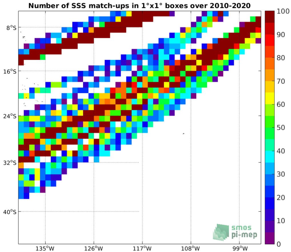
Figure 4: Number of SSS match-ups between TSG (LEGOS-DM) SSS and the CCI SSS L4 Merged-OI v3.2 - 30-day running (ESA) SSS product for the OTT zone Pi-MEP region over 1^\circ \times 1^\circ boxes and for the full satellite product period.
