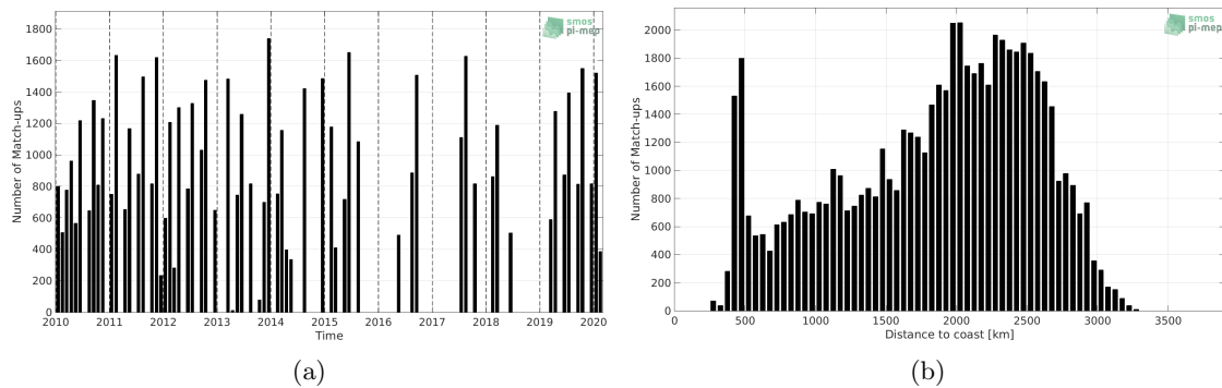
Figure 1: Number of match-ups between TSG (LEGOS-DM) and CCI SSS L4 Merged-OI v3.2 - 30-day running (ESA) SSS as a function of time (a) and as function of the distance to coast (b) over the OTT zone Pi-MEP region and for the full satellite product period.
