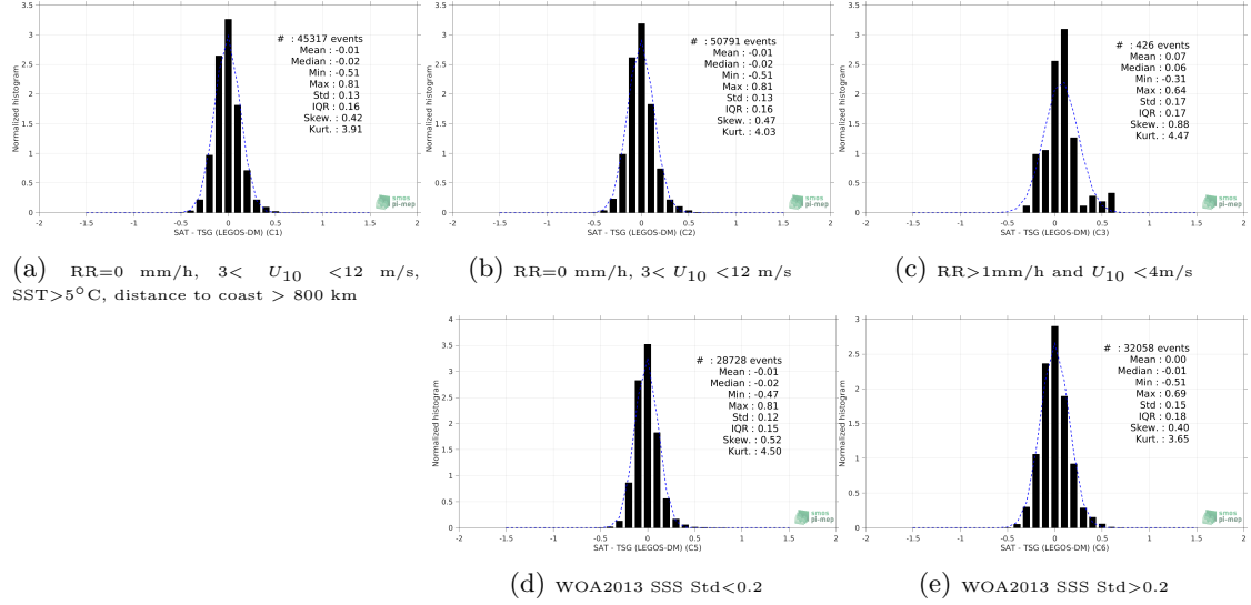
Figure 13: Normalized histogram of \Delta SSS (CCI SSS L4 Merged-OI v3.2 - 30-day running (ESA) - TSG (LEGOS-DM)) for 5 different subdatasets corresponding to: RR=0 mm/h, 3 < U_{10} < 12 m/s, SST>5°C, distance to coast > 800 km (a), RR=0 mm/h, 3 < U_{10} < 12 m/s (b), RR>1mm/h and U_{10} < 4 m/s (c), WOA2013 SSS Std<0.2 (d), WOA2013 SSS Std>0.2 (e).
