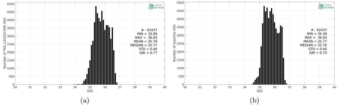
Figure 2: Histograms of SSS from TSG (LEGOS-DM) (a) and CCI SSS L4 Merged-OI v3.2 - 30-day running (ESA) (b) considering all match-up pairs per bins of 0.1 over the OTT zone Pi-MEP region and for the full satellite product period.
