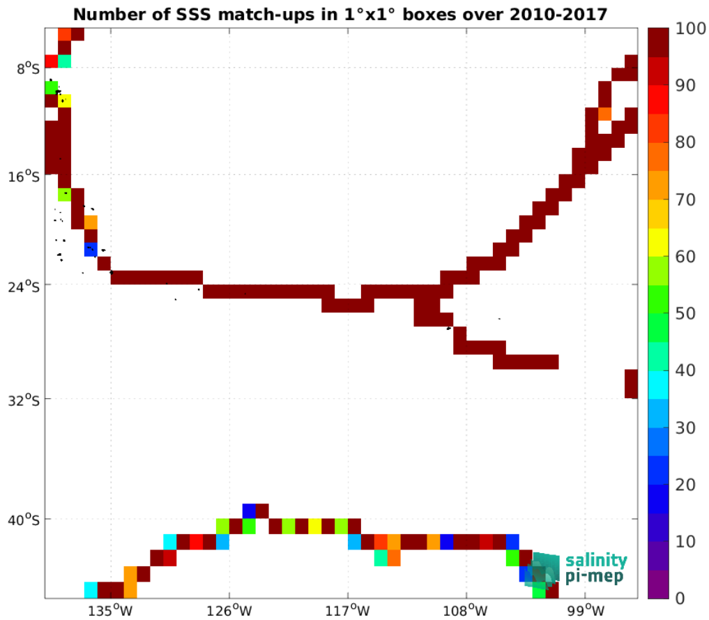
Figure 4: Number of SSS match-ups between TSG (GOSUD-Sailing-ship) SSS and the CCI SSS L4 Merged-OI v3.2 - 30-day running (ESA) SSS product for the OTT zone Pi-MEP region over 1^\circ \times 1^\circ boxes and for the full satellite product period.
