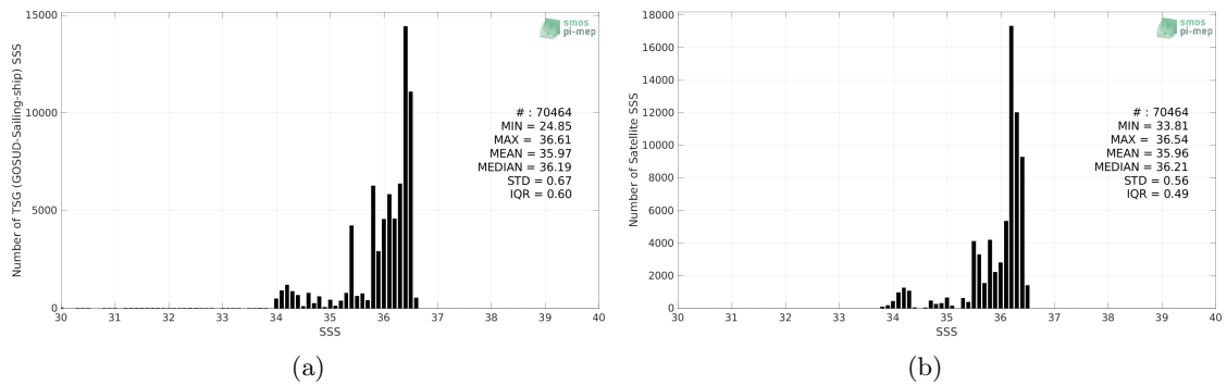
Figure 2: Histograms of SSS from TSG (GOSUD-Sailing-ship) (a) and CCI SSS L4 Merged-OI v3.2 - 30-day running (ESA) (b) considering all match-up pairs per bins of 0.1 over the OTT zone Pi-MEP region and for the full satellite product period.
