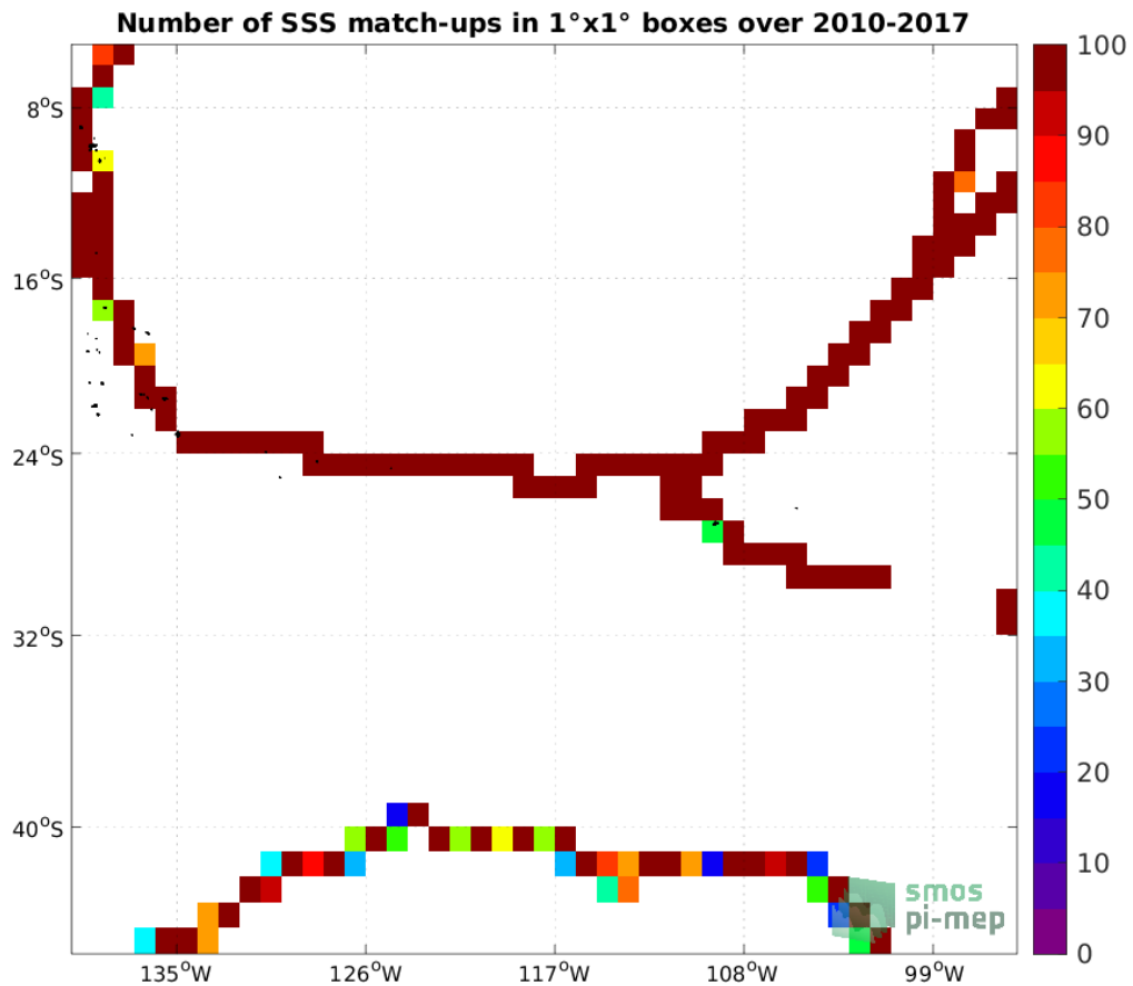
Figure 4: Number of SSS match-ups between TSG (GOSUD-Sailing-ship) SSS and the CCI SSS L4 Merged-OI v3.2 - 30-day running (ESA) SSS product for the OTT zone Pi-MEP region over 1°x1° boxes and for the full satellite product period.
