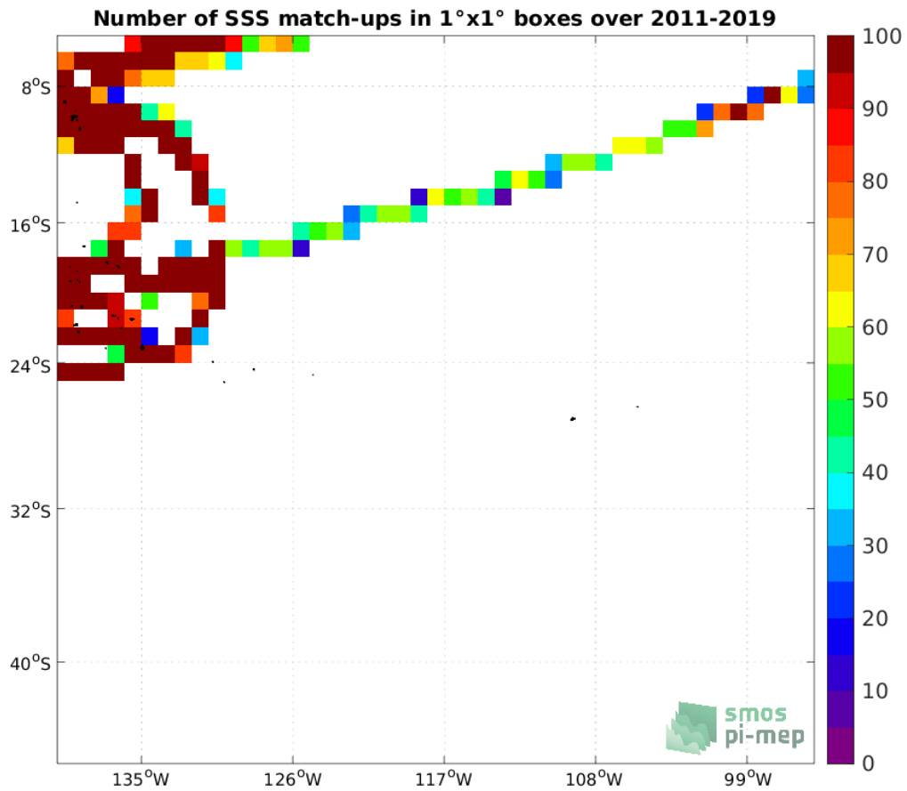
Figure 4: Number of SSS match-ups between TSG (GOSUD-Research-vessel) SSS and the CCI SSS L4 Merged-OI v3.2 - 30-day running (ESA) SSS product for the OTT zone Pi-MEP region over 1°x1° boxes and for the full satellite product period.
