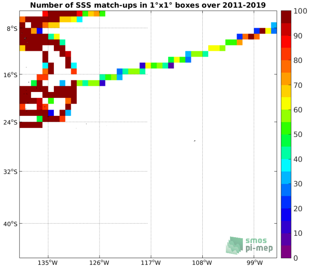
Figure 4: Number of SSS match-ups between TSG (GOSUD-Research-vessel) SSS and the CCI SSS L4 Merged-OI v3.2 - 30-day running (ESA) SSS product for the OTT zone Pi-MEP region over 1^\circ \times 1^\circ boxes and for the full satellite product period.
