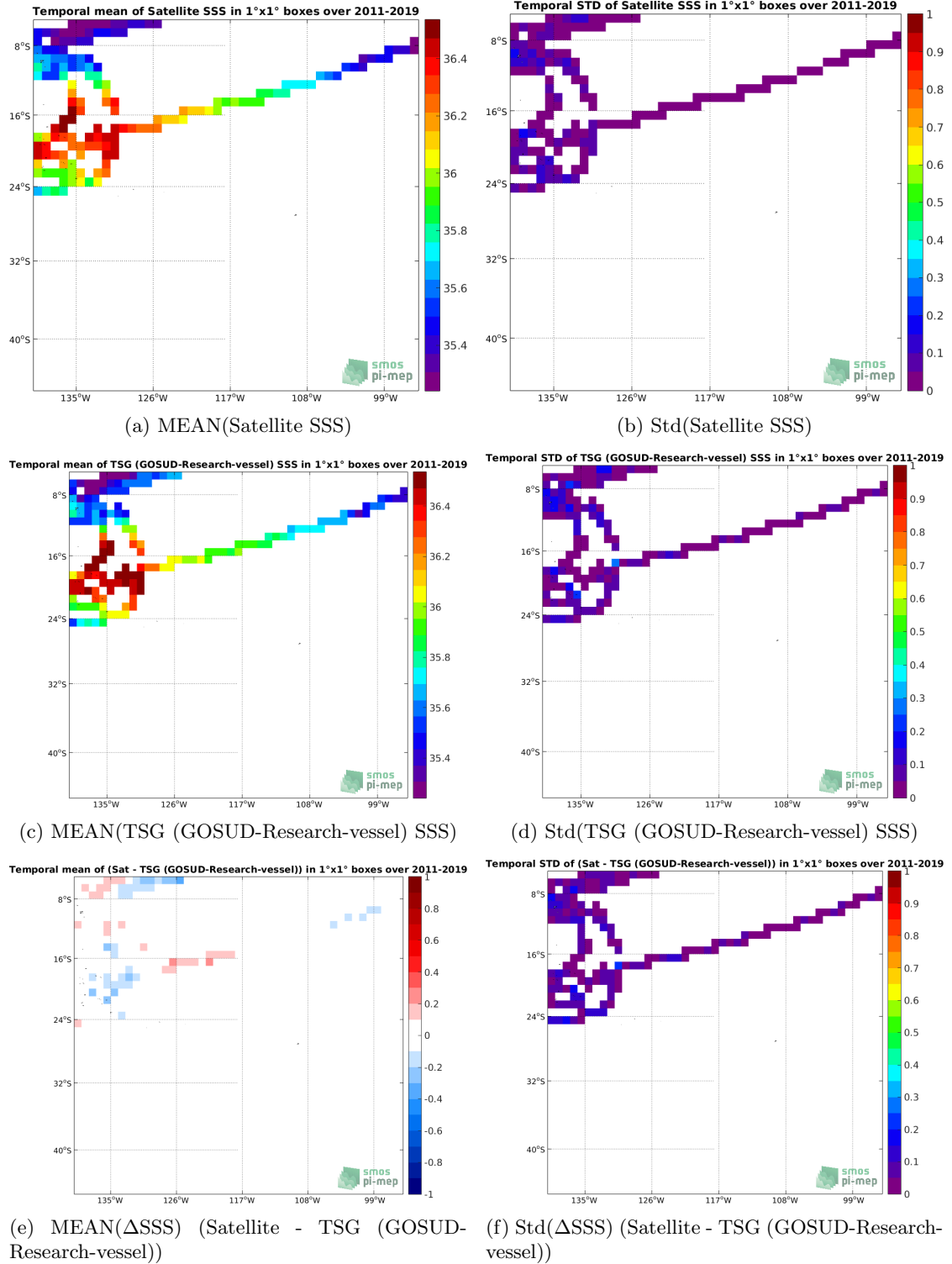
Figure 6: Temporal mean (left) and Std (right) of SSS from CCI SSS L4 Merged-OI v3.2 - 30-day running (ESA) (top), TSG (GOSUD-Research-vessel) (middle), and of \Delta SSS (Satellite - TSG (GOSUD-Research-vessel)). Only match-up pairs are used to generate these maps.
