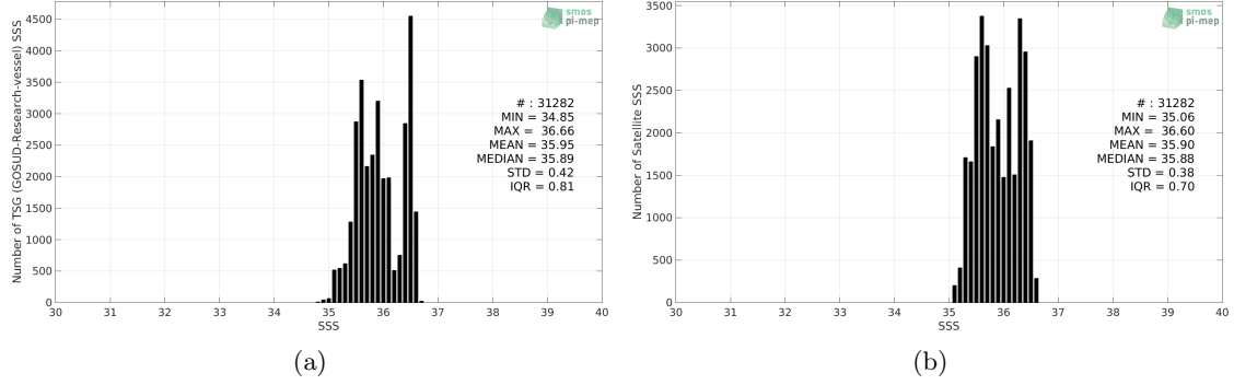
Figure 2: Histograms of SSS from TSG (GOSUD-Research-vessel) (a) and CCI SSS L4 Merged-OI v3.2 - 30-day running (ESA) (b) considering all match-up pairs per bins of 0.1 over the OTT zone Pi-MEP region and for the full satellite product period.
