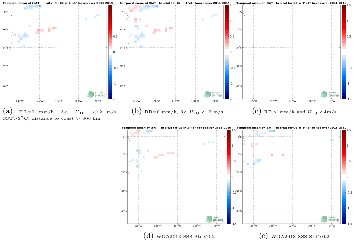
Figure 12: Temporal mean gridded over spatial boxes of size 1^\circ \times 1^\circ of \Delta SSS (CCI SSS L4 Merged-OI v3.2 - 30-day running (ESA) - TSG (GOSUD-Research-vessel)) for 5 different subdatasets corresponding to: RR=0 mm/h, 3 < U_{10} < 12 m/s, SST > 5^\circ\text{C} , distance to coast > 800 km (a), RR=0 mm/h, 3 < U_{10} < 12 m/s (b), RR > 1 mm/h and U_{10} < 4 m/s (c), WOA2013 SSS Std < 0.2 (d), WOA2013 SSS Std > 0.2 (e).
