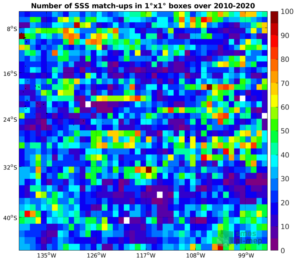
Figure 4: Number of SSS match-ups between Argo SSS and the CCI SSS L4 Merged-OI v3.2 - 30-day running (ESA) SSS product for the OTT zone Pi-MEP region over 1°x1° boxes and for the full satellite product period.
