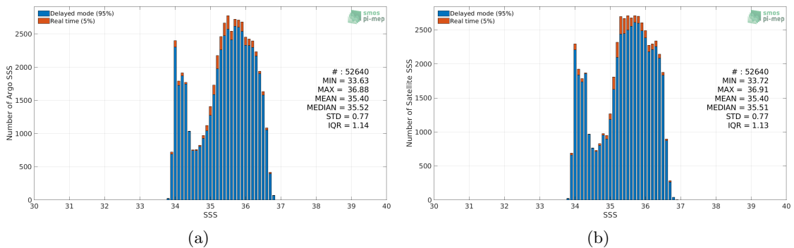
Figure 2: Histograms of SSS from Argo (a) and CCI SSS L4 Merged-OI v3.2 - 30-day running (ESA) (b) considering all match-up pairs per bins of 0.1 over the OTT zone Pi-MEP region and for the full satellite product period.
