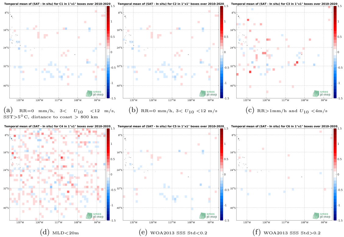
Figure 12: Temporal mean gridded over spatial boxes of size 1^\circ \times 1^\circ of \Delta SSS (CCI SSS L4 Merged-OI v3.2 - 30-day running (ESA) - Argo) for 6 different subdatasets corresponding to:RR=0 mm/h, 3 < U_{10} < 12 m/s, SST > 5^\circ C , distance to coast > 800 km (a), RR=0 mm/h, 3 < U_{10} < 12 m/s (b), RR >1 mm/h and U_{10} < 4 m/s (c),MLD <20 m (d),WOA2013 SSS Std <0.2 (e),WOA2013 SSS Std >0.2 (f).
