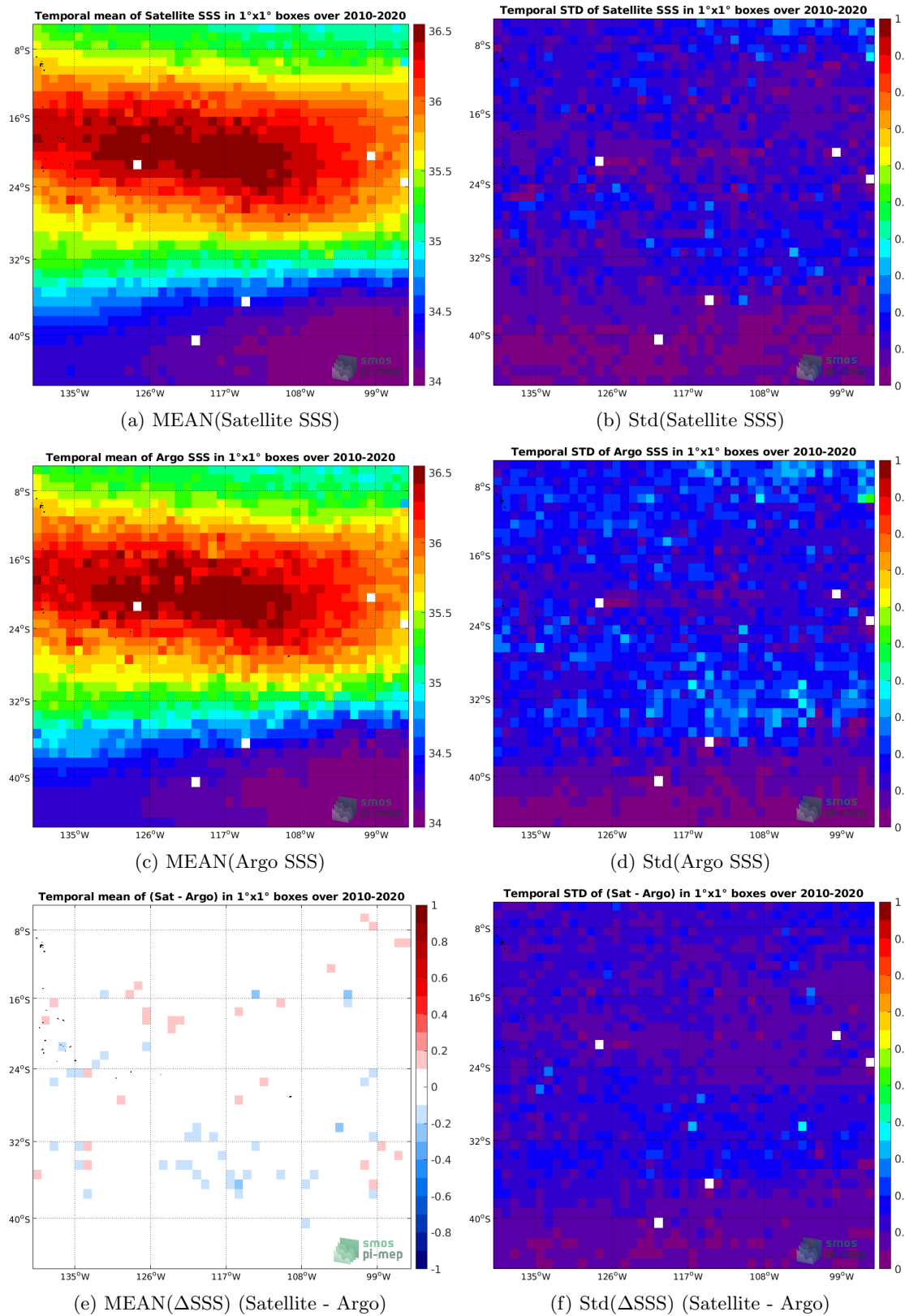
Figure 6: Temporal mean (left) and Std (right) of SSS from CCI SSS L4 Merged-OI v3.2 - 30-day running (ESA) (top), Argo (middle), and of \Delta SSS (Satellite - Argo). Only match-up pairs are used to generate these maps.
