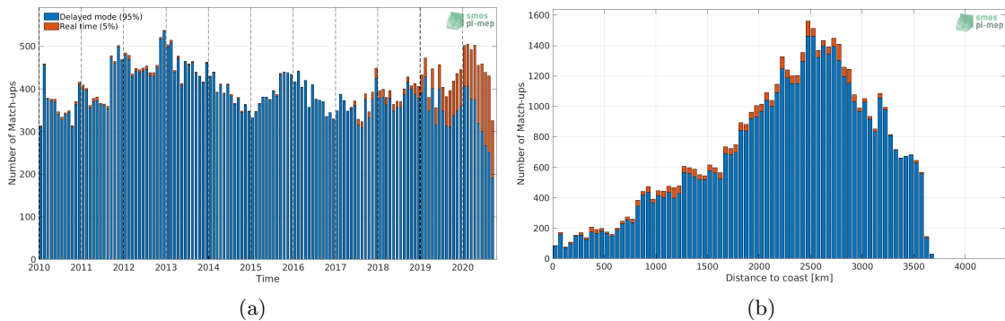
Figure 1: Number of match-ups between Argo and CCI SSS L4 Merged-OI v3.2 - 30-day running (ESA) SSS as a function of time (a) and as function of the distance to coast (b) over the OTT zone Pi-MEP region and for the full satellite product period.
