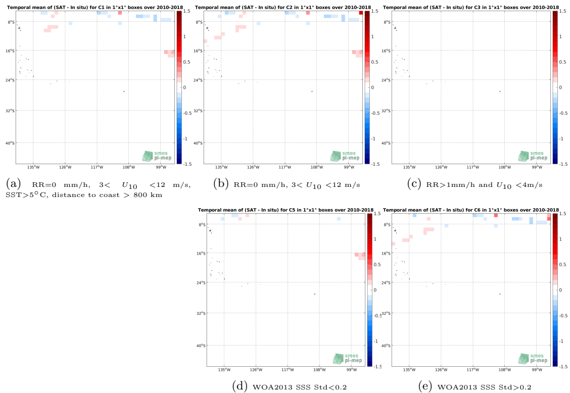
Figure 12: Temporal mean gridded over spatial boxes of size 1^\circ \times 1^\circ of \Delta SSS (CCI SSS L4 Merged-OI v2.31 - 7-day running (ESA) - TSG (SAMOS)) for 5 different subdatasets corresponding to: RR=0 mm/h, 3 < U_{10} < 12 m/s, SST > 5^\circ C , distance to coast > 800 km (a), RR=0 mm/h, 3 < U_{10} < 12 m/s (b), RR > 1 mm/h and U_{10} < 4 m/s (c), WOA2013 SSS Std < 0.2 (d), WOA2013 SSS Std > 0.2 (e).
