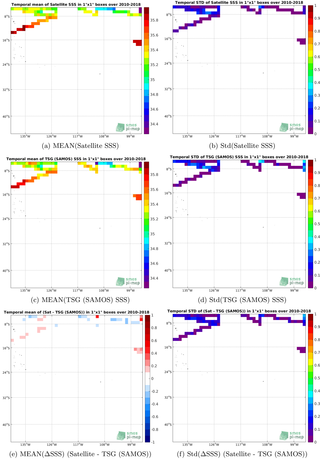
Figure 6: Temporal mean (left) and Std (right) of SSS from CCI L4 Merged-OI v2.31 - 7-day running (ESA) (top), TSG (SAMOS) (middle), and of \Delta SSS (Satellite - TSG (SAMOS)). Only match-up pairs are used to generate these maps.
