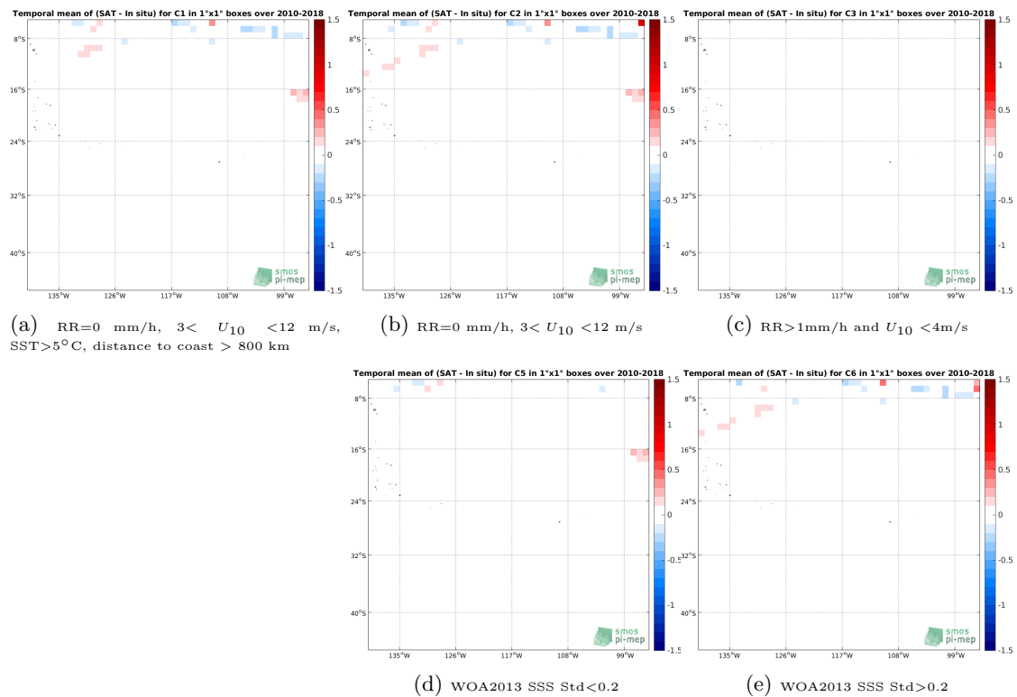
Figure 12: Temporal mean gridded over spatial boxes of size 1^\circ \times 1^\circ of \Delta SSS (CCI L4 Merged-OI v2.31 - 7-day running (ESA) - TSG (SAMOS)) for 5 different subdatasets corresponding to:RR=0 mm/h, 3 < U_{10} < 12 m/s, SST >5^\circ\text{C} , distance to coast > 800 km (a), RR=0 mm/h, 3 < U_{10} < 12 m/s (b), RR >1 mm/h and U_{10} < 4 m/s (c), WOA2013 SSS Std <0.2 (d), WOA2013 SSS Std >0.2 (e).
