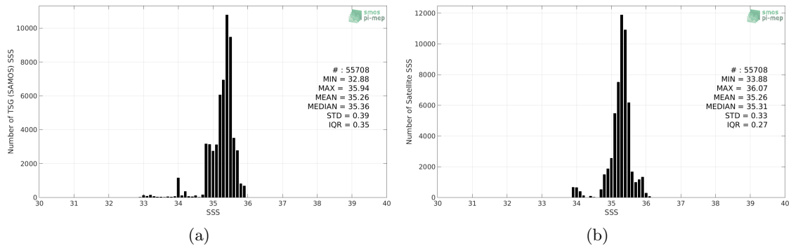
Figure 2: Histograms of SSS from TSG (SAMOS) (a) and CCI L4 Merged-OI v2.31 - 7-day running (ESA) (b) considering all match-up pairs per bins of 0.1 over the OTT zone Pi-MEP region and for the full satellite product period.
