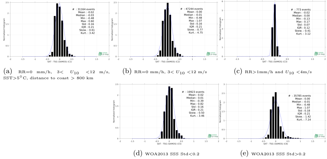
Figure 13: Normalized histogram of \Delta SSS (CCI L4 Merged-OI v2.31 - 7-day running (ESA) - TSG (SAMOS)) for 5 different subdatasets corresponding to: RR=0 mm/h, 3 < U_{10} < 12 m/s, SST > 5°C, distance to coast > 800 km (a), RR=0 mm/h, 3 < U_{10} < 12 m/s (b), RR > 1mm/h and U_{10} < 4 m/s (c), WOA2013 SSS Std < 0.2 (d), WOA2013 SSS Std > 0.2 (e).
