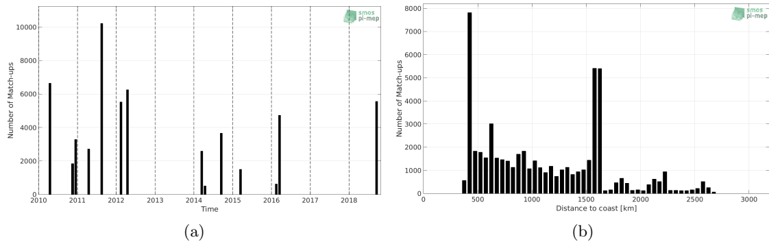
Figure 1: Number of match-ups between TSG (SAMOS) and CCI L4 Merged-OI v2.31 - 7-day running (ESA) SSS as a function of time (a) and as function of the distance to coast (b) over the OTT zone Pi-MEP region and for the full satellite product period.
