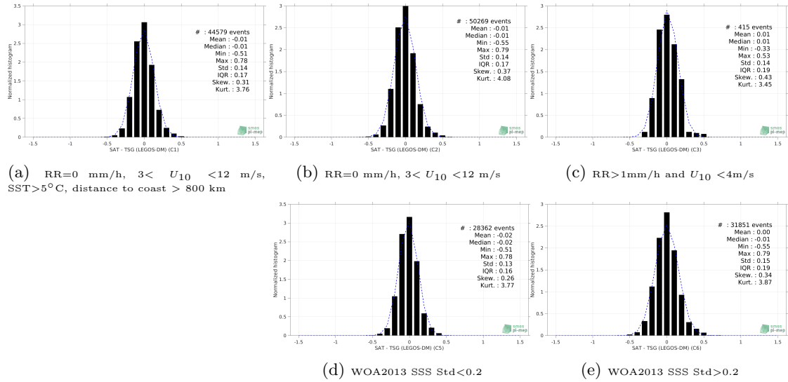
Figure 13: Normalized histogram of \Delta SSS (CCI SSS L4 Merged-OI v2.31 - 7-day running (ESA) - TSG (LEGOS-DM)) for 5 different subdatasets corresponding to: RR=0 mm/h, 3 < U_{10} < 12 m/s, SST > 5°C, distance to coast > 800 km (a), RR=0 mm/h, 3 < U_{10} < 12 m/s (b), RR > 1mm/h and U_{10} < 4 m/s (c), WOA2013 SSS Std < 0.2 (d), WOA2013 SSS Std > 0.2 (e).
