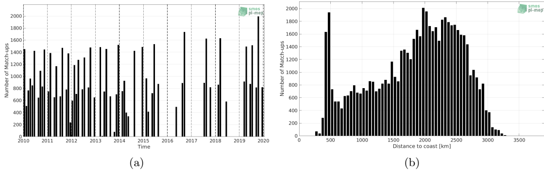
Figure 1: Number of match-ups between TSG (LEGOS-DM) and CCI SSS L4 Merged-OI v2.31 - 7-day running (ESA) SSS as a function of time (a) and as function of the distance to coast (b) over the OTT zone Pi-MEP region and for the full satellite product period.
