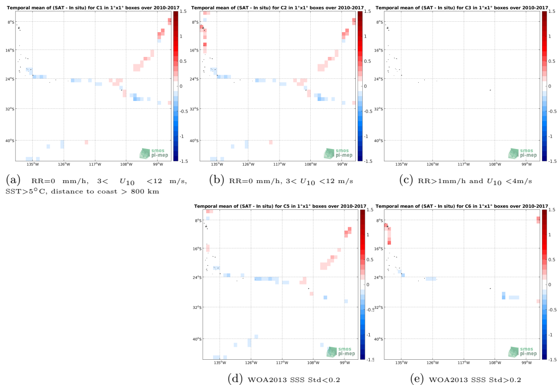
Figure 12: Temporal mean gridded over spatial boxes of size 1^\circ \times 1^\circ of \Delta SSS (CCI SSS L4 Merged-OI v2.31 - 7-day running (ESA) - TSG (GOSUD-Sailing-ship)) for 5 different subdatasets corresponding to: RR=0 mm/h, 3 < U_{10} < 12 m/s, SST > 5^\circ C , distance to coast > 800 km (a), RR=0 mm/h, 3 < U_{10} < 12 m/s (b), RR > 1 mm/h and U_{10} < 4 m/s (c), WOA2013 SSS Std < 0.2 (d), WOA2013 SSS Std > 0.2 (e).
