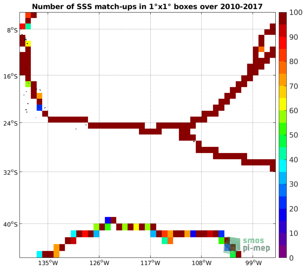
Figure 4: Number of SSS match-ups between TSG (GOSUD-Sailing-ship) SSS and the CCI SSS L4 Merged-OI v2.31 - 7-day running (ESA) SSS product for the OTT zone Pi-MEP region over 1°x1° boxes and for the full satellite product period.
