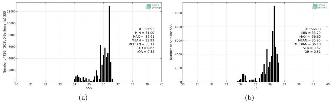
Figure 2: Histograms of SSS from TSG (GOSUD-Sailing-ship) (a) and CCI SSS L4 Merged-OI v2.31 - 7-day running (ESA) (b) considering all match-up pairs per bins of 0.1 over the OTT zone Pi-MEP region and for the full satellite product period.
