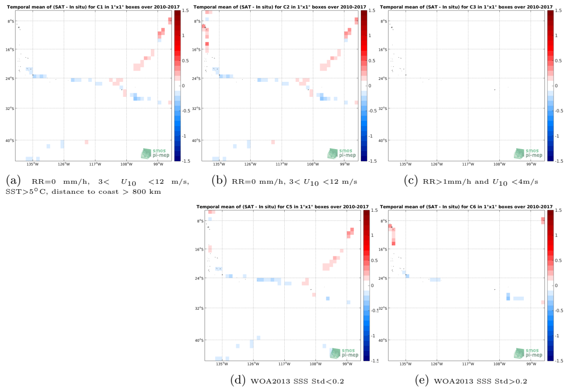
Figure 12: Temporal mean gridded over spatial boxes of size 1^\circ \times 1^\circ of \Delta\text{SSS} (CCI SSS L4 Merged-OI v2.31 - 7-day running (ESA) - TSG (GOSUD-Sailing-ship)) for 5 different subdatasets corresponding to: \text{RR}=0 \text{ mm/h} , 3 < U_{10} < 12 \text{ m/s} , \text{SST} > 5^\circ\text{C} , distance to coast > 800 \text{ km} (a), \text{RR}=0 \text{ mm/h} , 3 < U_{10} < 12 \text{ m/s} (b), \text{RR} > 1 \text{ mm/h} and U_{10} < 4 \text{ m/s} (c), WOA2013 SSS Std < 0.2 (d), WOA2013 SSS Std > 0.2 (e).
