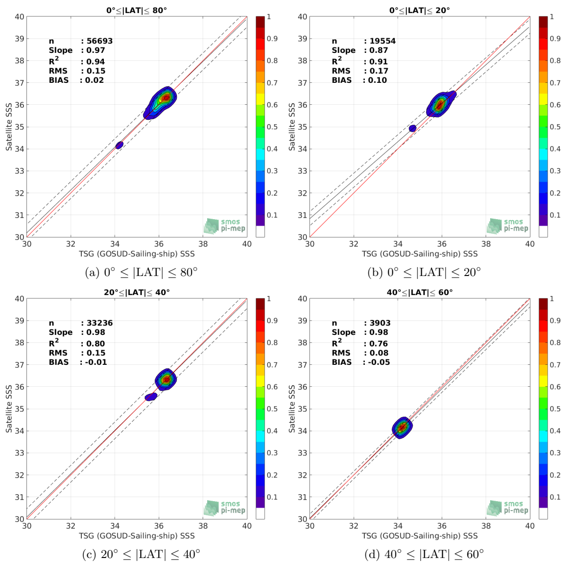
Figure 9: Contour maps of the concentration of CCI SSS L4 Merged-OI v2.31 - 7-day running (ESA) SSS (y-axis) versus TSG (GOSUD-Sailing-ship) SSS (x-axis) at match-up pairs for different latitude bands. For each plot, the red line shows x=y . The black thin and dashed lines indicate a linear fit through the data cloud and the \pm 95\% confidence levels, respectively. The number match-up pairs n , the slope and R^2 coefficient of the linear fit, the root mean square (RMS) and the mean bias between satellite and in situ data are indicated for each latitude band in each plots.
