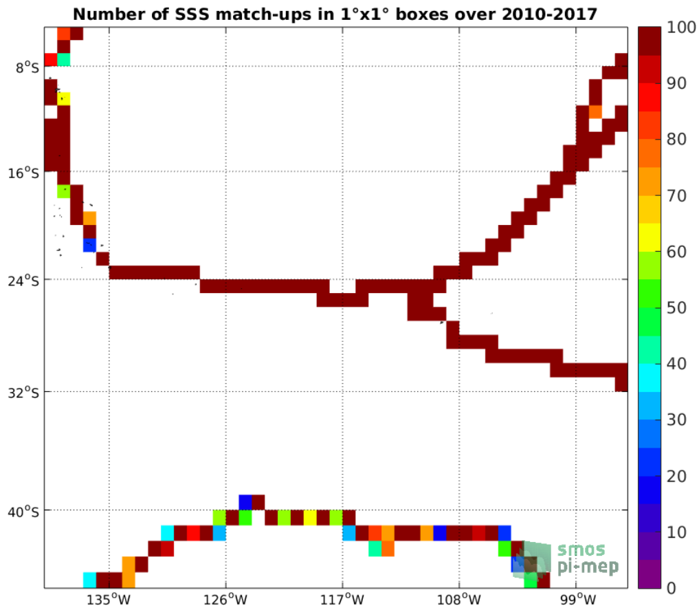
Figure 4: Number of SSS match-ups between TSG (GOSUD-Sailing-ship) SSS and the CCI SSS L4 Merged-OI v2.31 - 7-day running (ESA) SSS product for the OTT zone Pi-MEP region over 1^\circ \times 1^\circ boxes and for the full satellite product period.
