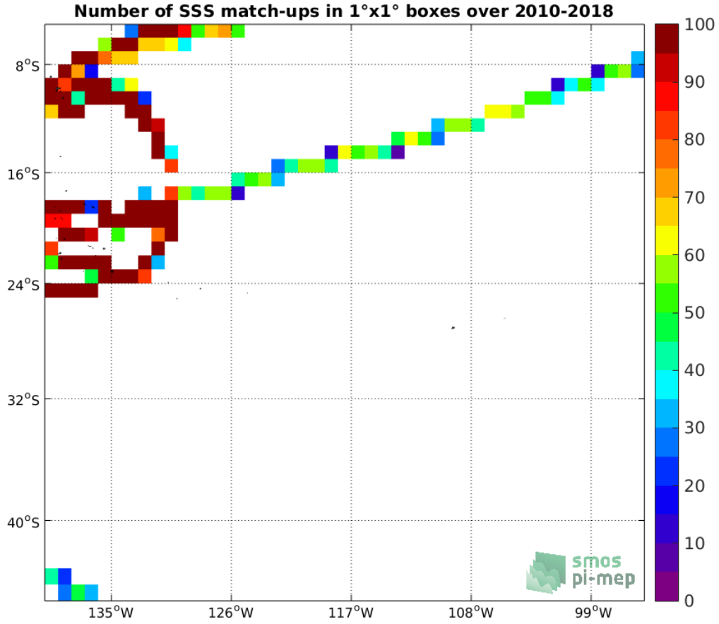
Figure 4: Number of SSS match-ups between TSG (GOSUD-Research-vessel) SSS and the CCI SSS L4 Merged-OI v2.31 - 7-day running (ESA) SSS product for the OTT zone Pi-MEP region over 1°x1° boxes and for the full satellite product period.
