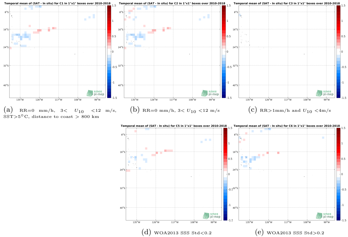
Figure 12: Temporal mean gridded over spatial boxes of size 1^\circ \times 1^\circ of \Delta\text{SSS} (CCI SSS L4 Merged-OI v2.31 - 7-day running (ESA) - TSG (GOSUD-Research-vessel)) for 5 different subdatasets corresponding to: \text{RR}=0 \text{ mm/h} , 3 < U_{10} < 12 \text{ m/s} , \text{SST} > 5^\circ\text{C} , distance to coast > 800 \text{ km} (a), \text{RR}=0 \text{ mm/h} , 3 < U_{10} < 12 \text{ m/s} (b), \text{RR} > 1 \text{ mm/h} and U_{10} < 4 \text{ m/s} (c), WOA2013 SSS Std < 0.2 (d), WOA2013 SSS Std > 0.2 (e).
