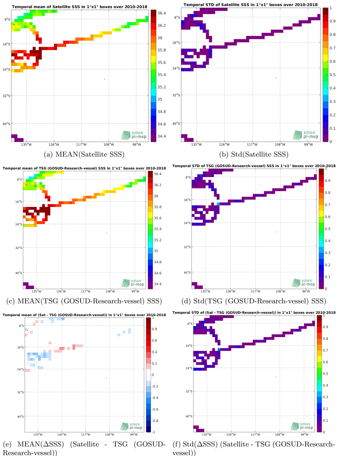
Figure 6: Temporal mean (left) and Std (right) of SSS from CCI SSS L4 Merged-OI v2.31 - 7-day running (ESA) (top), TSG (GOSUD-Research-vessel) (middle), and of \Delta SSS (Satellite - TSG (GOSUD-Research-vessel)). Only match-up pairs are used to generate these maps.
