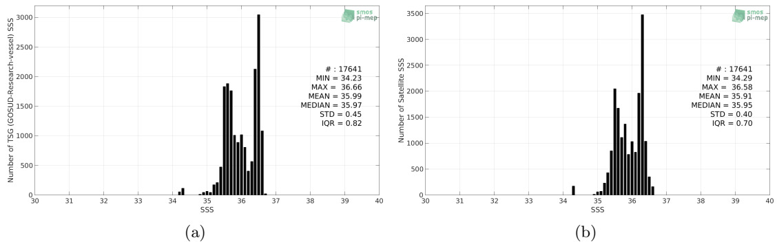
Figure 2: Histograms of SSS from TSG (GOSUD-Research-vessel) (a) and CCI SSS L4 Merged-OI v2.31 - 7-day running (ESA) (b) considering all match-up pairs per bins of 0.1 over the OTT zone Pi-MEP region and for the full satellite product period.
