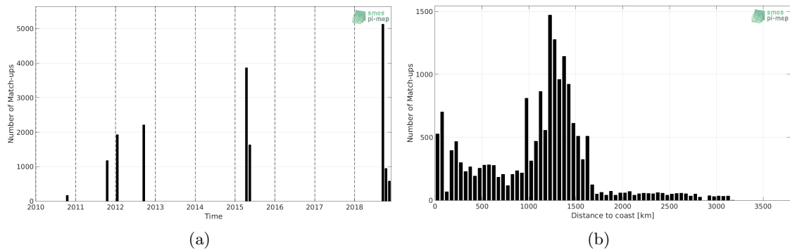
Figure 1: Number of match-ups between TSG (GOSUD-Research-vessel) and CCI L4 Merged-OI v2.31 - 7-day running (ESA) SSS as a function of time (a) and as function of the distance to coast (b) over the OTT zone Pi-MEP region and for the full satellite product period.
