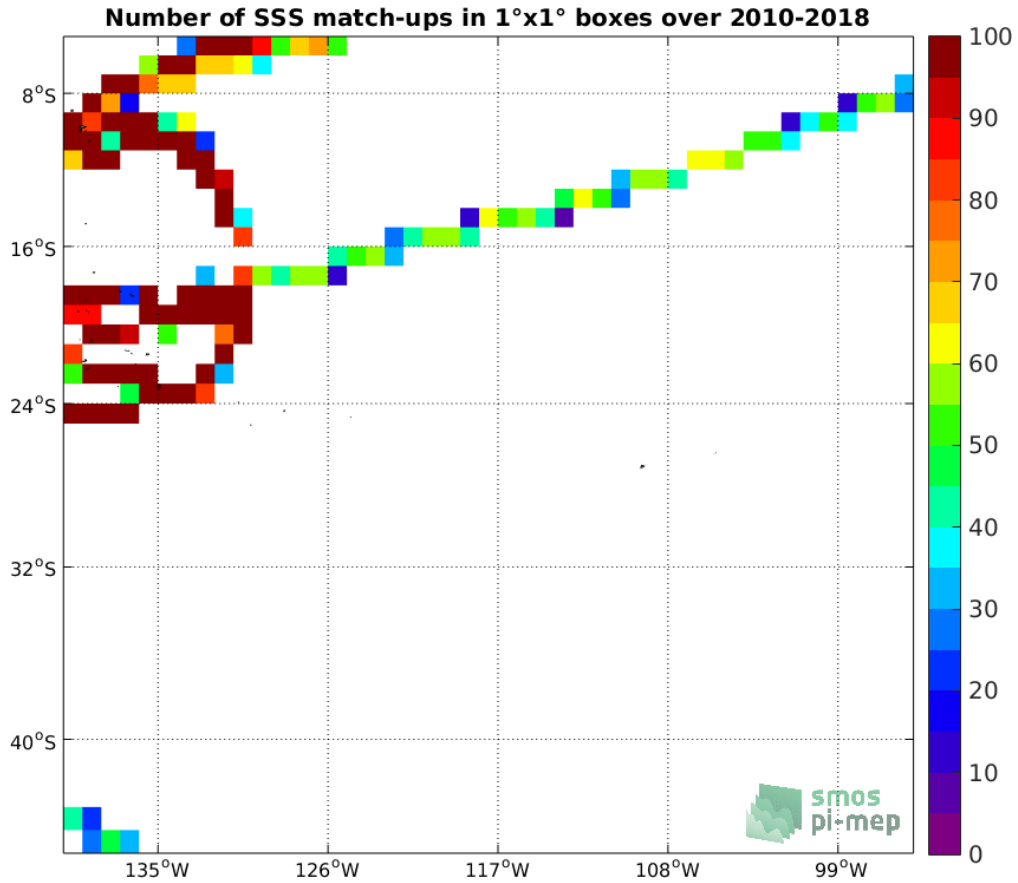
Figure 4: Number of SSS match-ups between TSG (GOSUD-Research-vessel) SSS and the CCI L4 Merged-OI v2.31 - 7-day running (ESA) SSS product for the OTT zone Pi-MEP region over 1^{\circ} \times 1^{\circ} boxes and for the full satellite product period.
