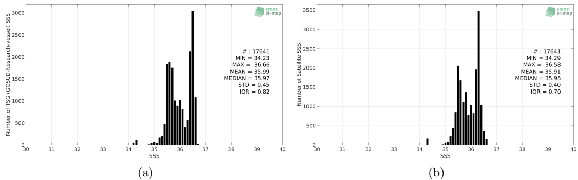
Figure 2: Histograms of SSS from TSG (GOSUD-Research-vessel) (a) and CCI L4 Merged-OI v2.31 - 7-day running (ESA) (b) considering all match-up pairs per bins of 0.1 over the OTT zone Pi-MEP region and for the full satellite product period.
