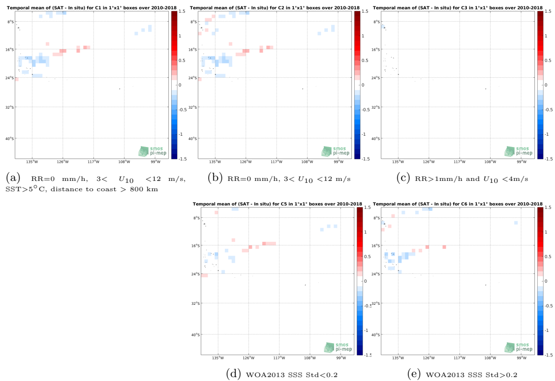
Figure 12: Temporal mean gridded over spatial boxes of size 1^\circ \times 1^\circ of \Delta SSS (CCI L4 Merged-OI v2.31 - 7-day running (ESA) - TSG (GOSUD-Research-vessel)) for 5 different subdatasets corresponding to: RR=0 mm/h, 3 < U_{10} < 12 m/s, SST > 5^\circ C , distance to coast > 800 km (a), RR=0 mm/h, 3 < U_{10} < 12 m/s (b), RR > 1 mm/h and U_{10} < 4 m/s (c), WOA2013 SSS Std < 0.2 (d), WOA2013 SSS Std > 0.2 (e).
