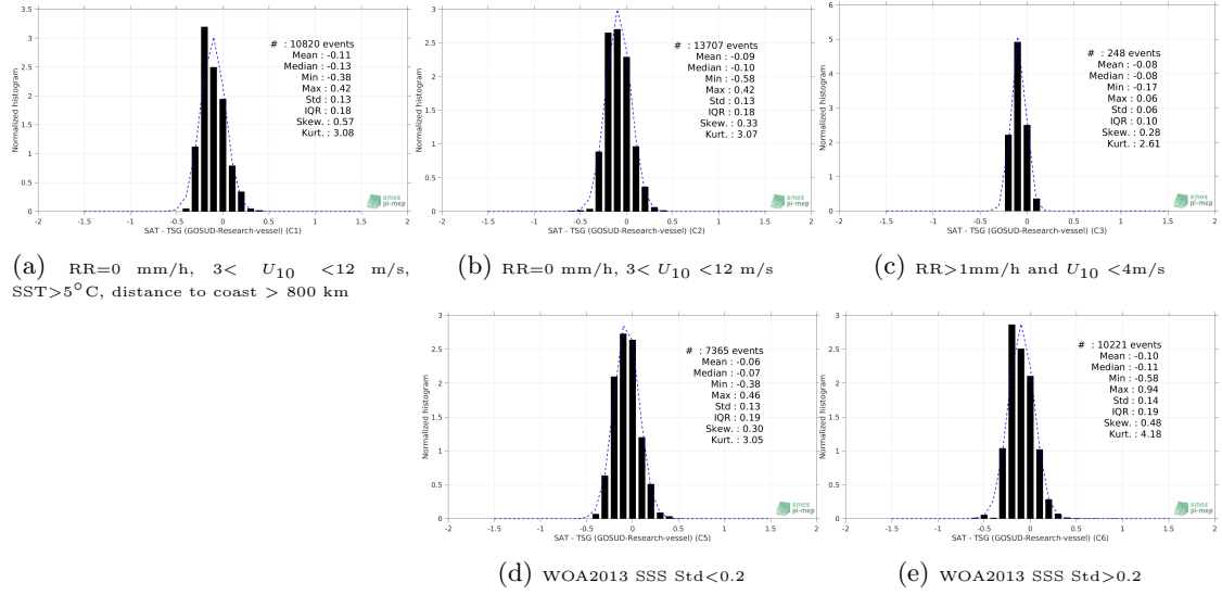
Figure 13: Normalized histogram of \Delta\text{SSS} (CCI L4 Merged-OI v2.31 - 7-day running (ESA) - TSG (GOSUD-Research-vessel)) for 5 different subdatasets corresponding to: RR=0 mm/h, 3 < U_{10} < 12 m/s, SST > 5^\circ\text{C} , distance to coast > 800 km (a), RR=0 mm/h, 3 < U_{10} < 12 m/s (b), RR > 1\text{mm/h} and U_{10} < 4\text{m/s} (c), WOA2013 SSS Std < 0.2 (d), WOA2013 SSS Std > 0.2 (e).
