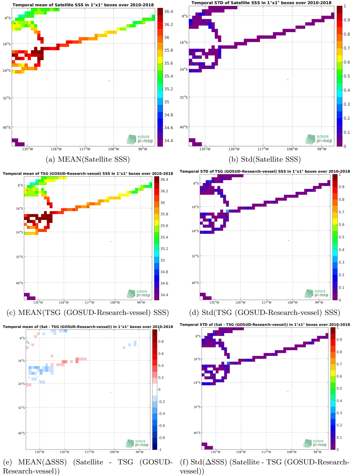
Figure 6: Temporal mean (left) and Std (right) of SSS from CCI L4 Merged-OI v2.31 - 7-day running (ESA) (top), TSG (GOSUD-Research-vessel) (middle), and of \Delta SSS (Satellite - TSG (GOSUD-Research-vessel)). Only match-up pairs are used to generate these maps.
