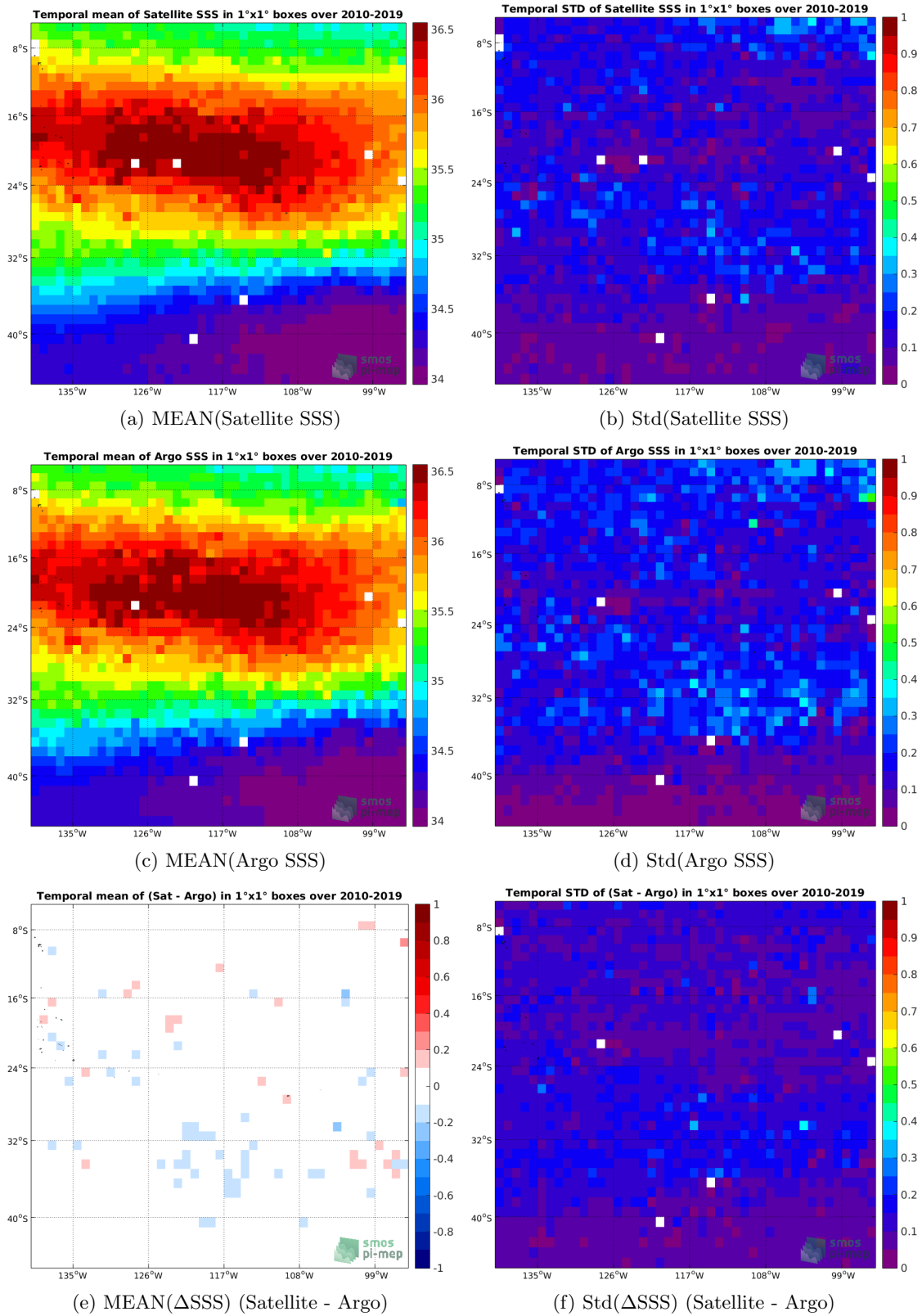
Figure 6: Temporal mean (left) and Std (right) of SSS from CCI SSS L4 Merged-OI v2.31 - 7-day running (ESA) (top), Argo (middle), and of \Delta SSS (Satellite - Argo). Only match-up pairs are used to generate these maps.
