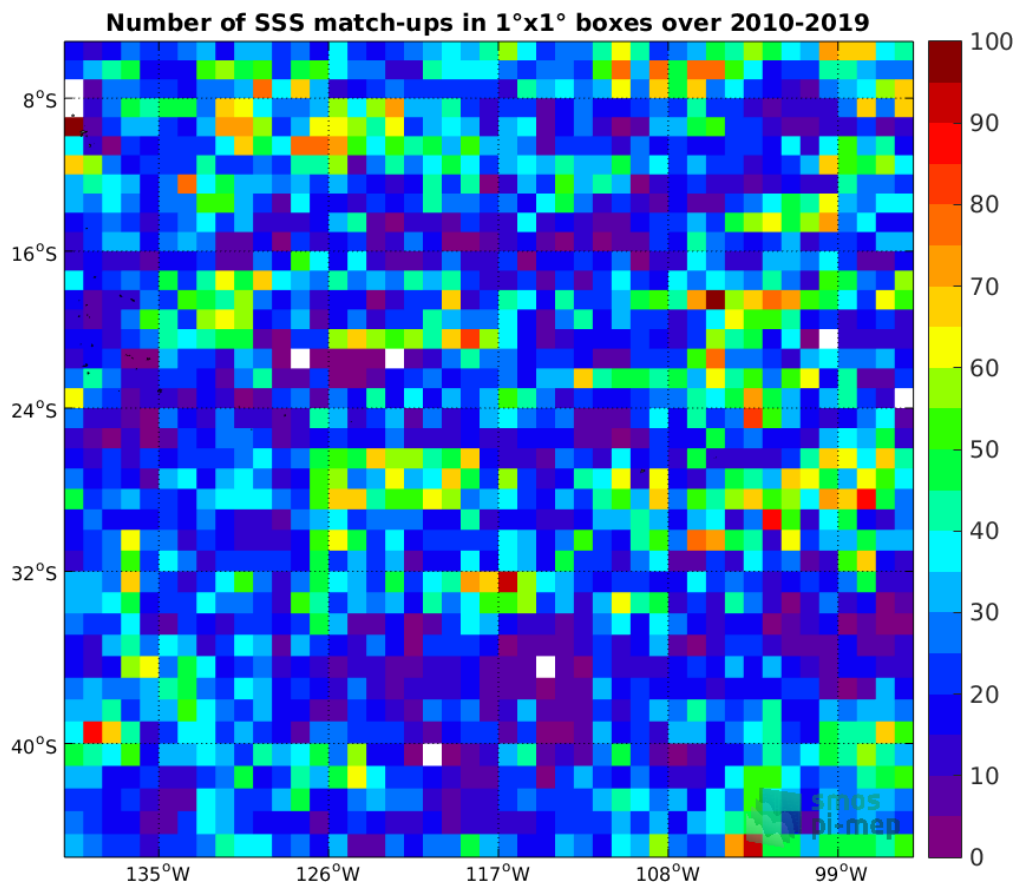
Figure 4: Number of SSS match-ups between Argo SSS and the CCI SSS L4 Merged-OI v2.31 - 7-day running (ESA) SSS product for the OTT zone Pi-MEP region over 1°x1° boxes and for the full satellite product period.
