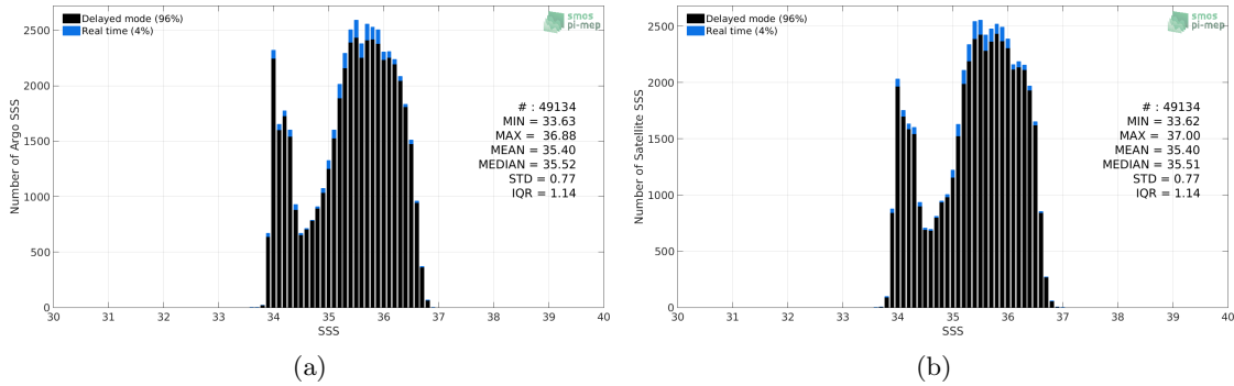
Figure 2: Histograms of SSS from Argo (a) and CCI SSS L4 Merged-OI v2.31 - 7-day running (ESA) (b) considering all match-up pairs per bins of 0.1 over the OTT zone Pi-MEP region and for the full satellite product period.
