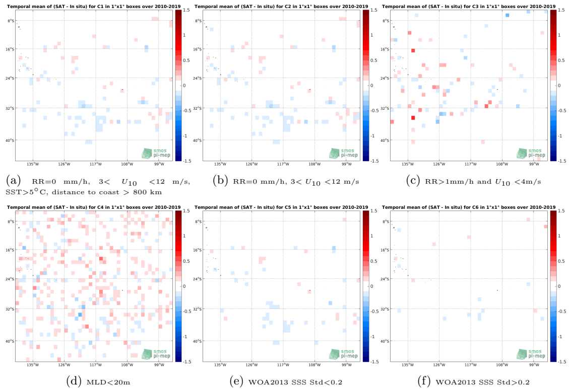
Figure 12: Temporal mean gridded over spatial boxes of size 1^\circ \times 1^\circ of \Delta SSS (CCI SSS L4 Merged-OI v2.31 - 7-day running (ESA) - Argo) for 6 different subdatasets corresponding to:RR=0 mm/h, 3 < U_{10} < 12 m/s, SST >5^\circ\text{C} , distance to coast > 800 km (a), RR=0 mm/h, 3 < U_{10} < 12 m/s (b), RR >1 mm/h and U_{10} < 4 m/s (c),MLD <20 m (d),WOA2013 SSS Std <0.2 (e),WOA2013 SSS Std >0.2 (f).
