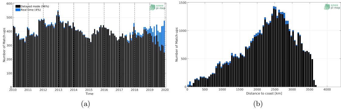
Figure 1: Number of match-ups between Argo and CCI SSS L4 Merged-OI v2.31 - 7-day running (ESA) SSS as a function of time (a) and as function of the distance to coast (b) over the OTT zone Pi-MEP region and for the full satellite product period.
