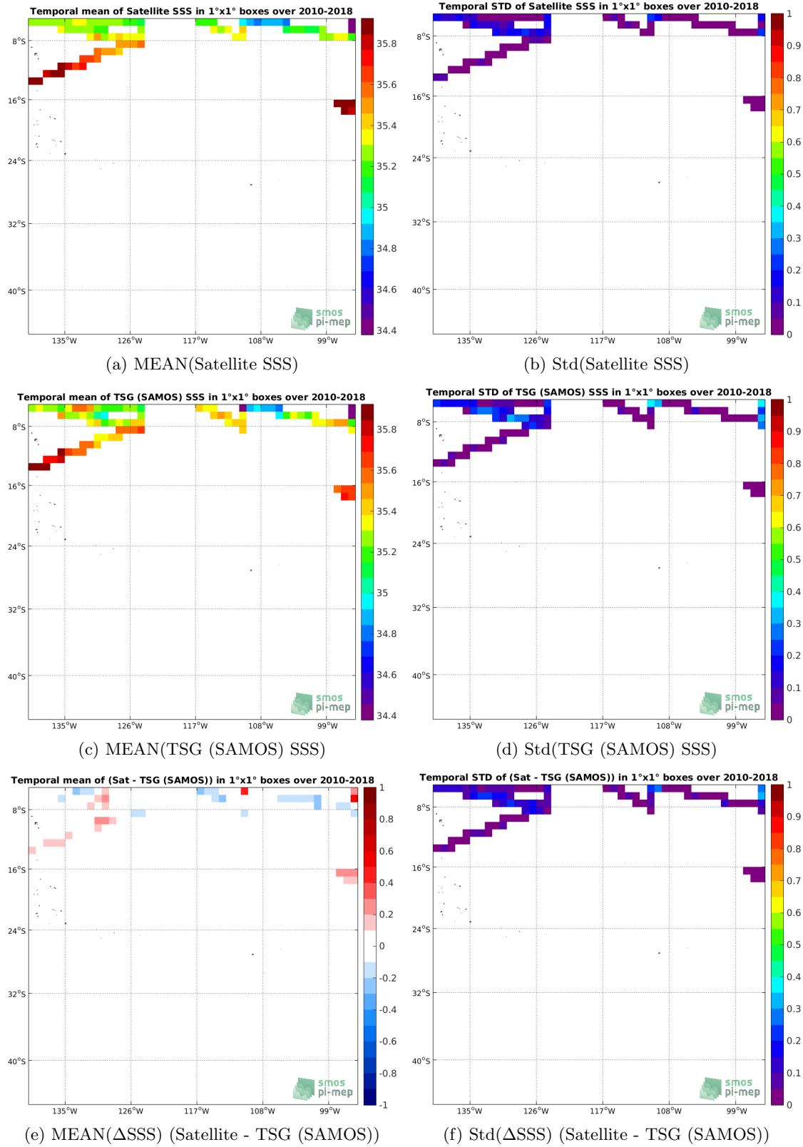
Figure 6: Temporal mean (left) and Std (right) of SSS from CCI SSS L4 Merged-OI v2.31 - 30-day running (ESA) (top), TSG (SAMOS) (middle), and of \Delta SSS (Satellite - TSG (SAMOS)). Only match-up pairs are used to generate these maps.
