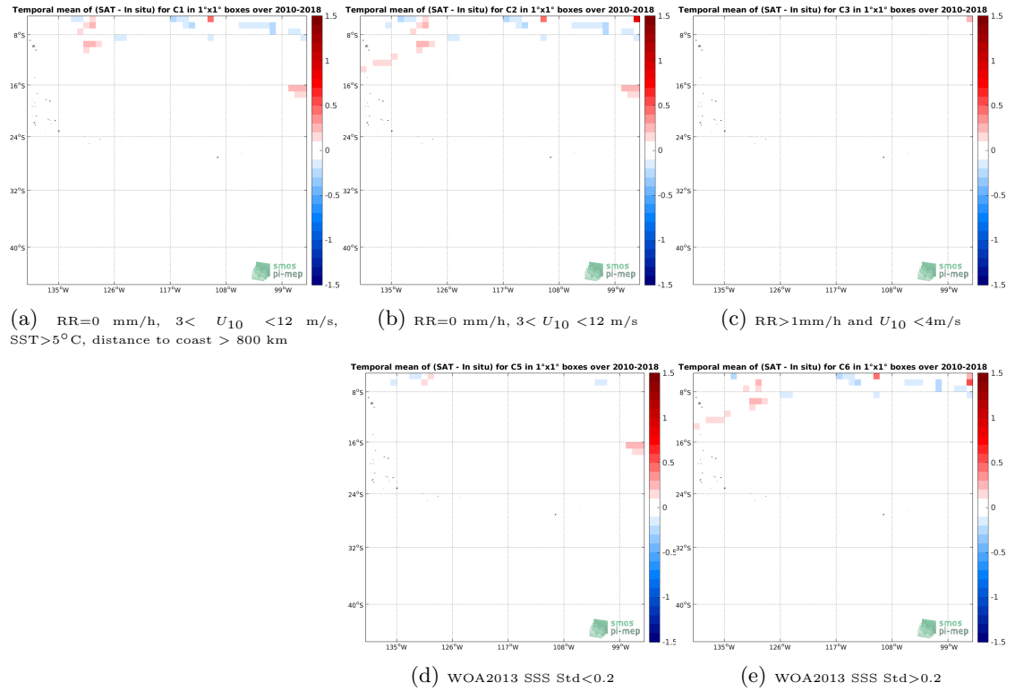
Figure 12: Temporal mean gridded over spatial boxes of size 1^\circ \times 1^\circ of \Delta SSS (CCI L4 Merged-OI v2.31 - 30-day running (ESA) - TSG (SAMOS)) for 5 different subdatasets corresponding to: RR=0 mm/h, 3 < U_{10} < 12 m/s, SST > 5^\circ C , distance to coast > 800 km (a), RR=0 mm/h, 3 < U_{10} < 12 m/s (b), RR > 1 mm/h and U_{10} < 4 m/s (c), WOA2013 SSS Std < 0.2 (d), WOA2013 SSS Std > 0.2 (e).
