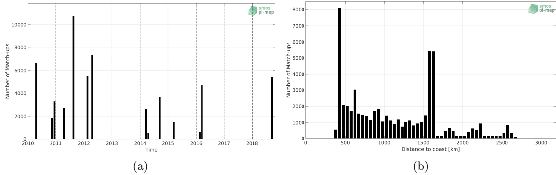
Figure 1: Number of match-ups between TSG (SAMOS) and CCI L4 Merged-OI v2.31 - 30-day running (ESA) SSS as a function of time (a) and as function of the distance to coast (b) over the OTT zone Pi-MEP region and for the full satellite product period.
