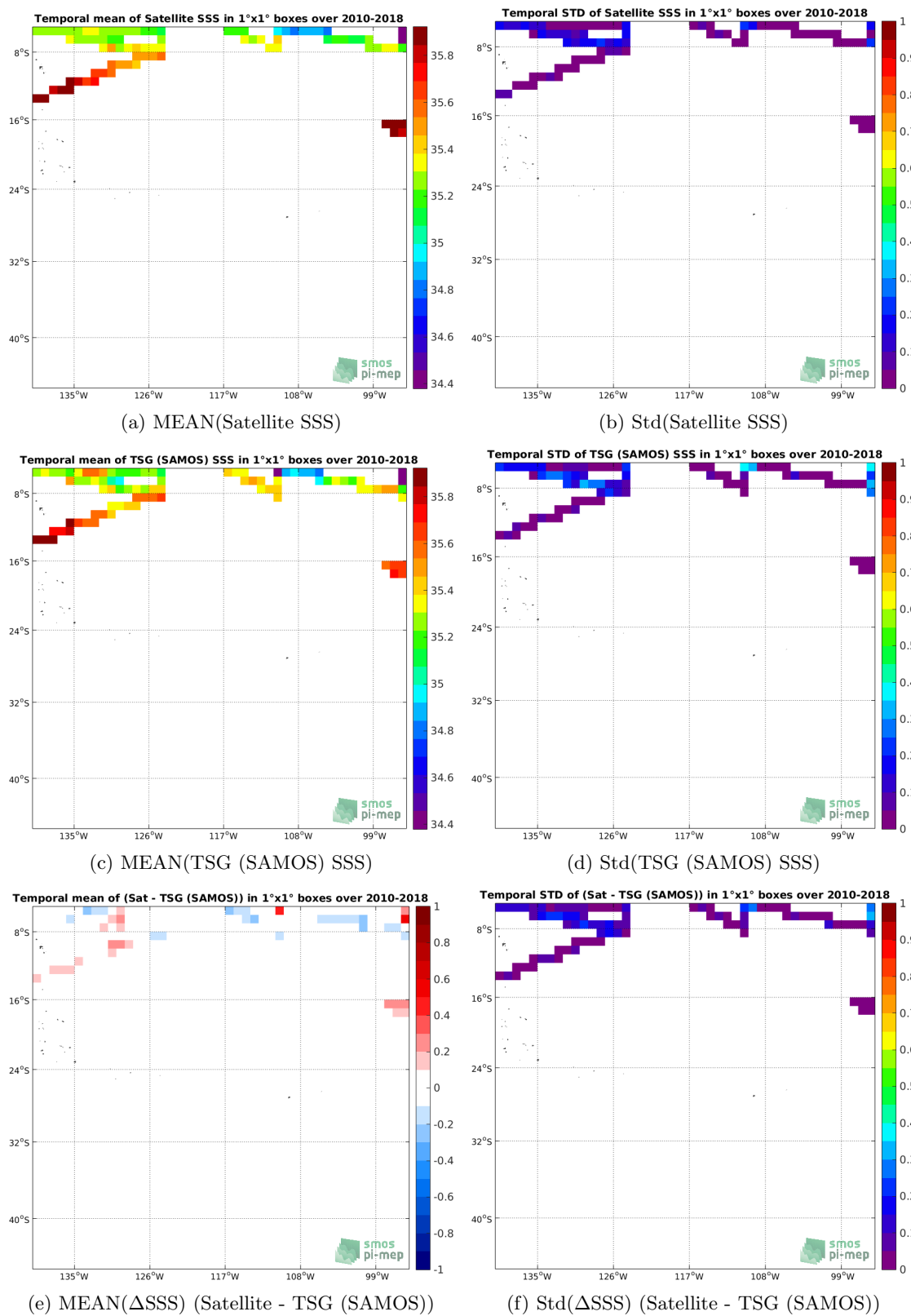
Figure 6: Temporal mean (left) and Std (right) of SSS from CCI L4 Merged-OI v2.31 - 30-day running (ESA) (top), TSG (SAMOS) (middle), and of \Delta SSS (Satellite - TSG (SAMOS)). Only match-up pairs are used to generate these maps.
