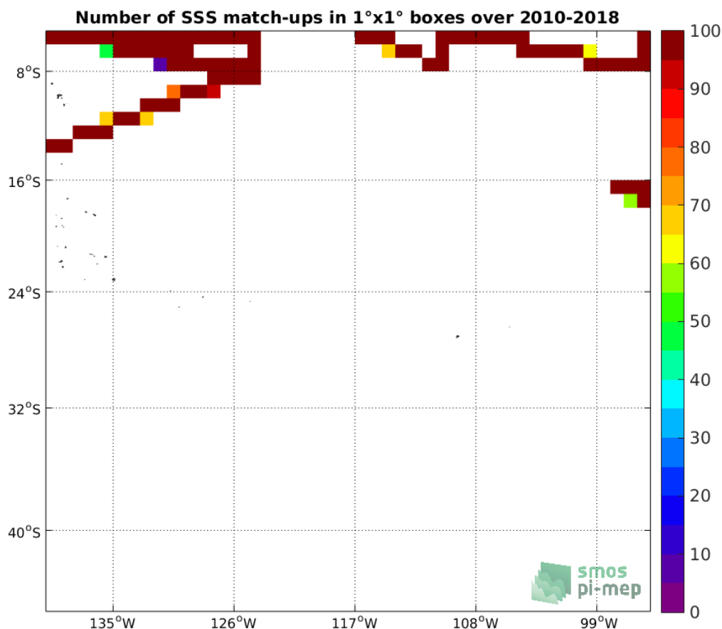
Figure 4: Number of SSS match-ups between TSG (SAMOS) SSS and the CCI L4 Merged-OI v2.31 - 30-day running (ESA) SSS product for the OTT zone Pi-MEP region over 1°x1° boxes and for the full satellite product period.
