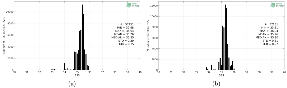
Figure 2: Histograms of SSS from TSG (SAMOS) (a) and CCI L4 Merged-OI v2.31 - 30-day running (ESA) (b) considering all match-up pairs per bins of 0.1 over the OTT zone Pi-MEP region and for the full satellite product period.
