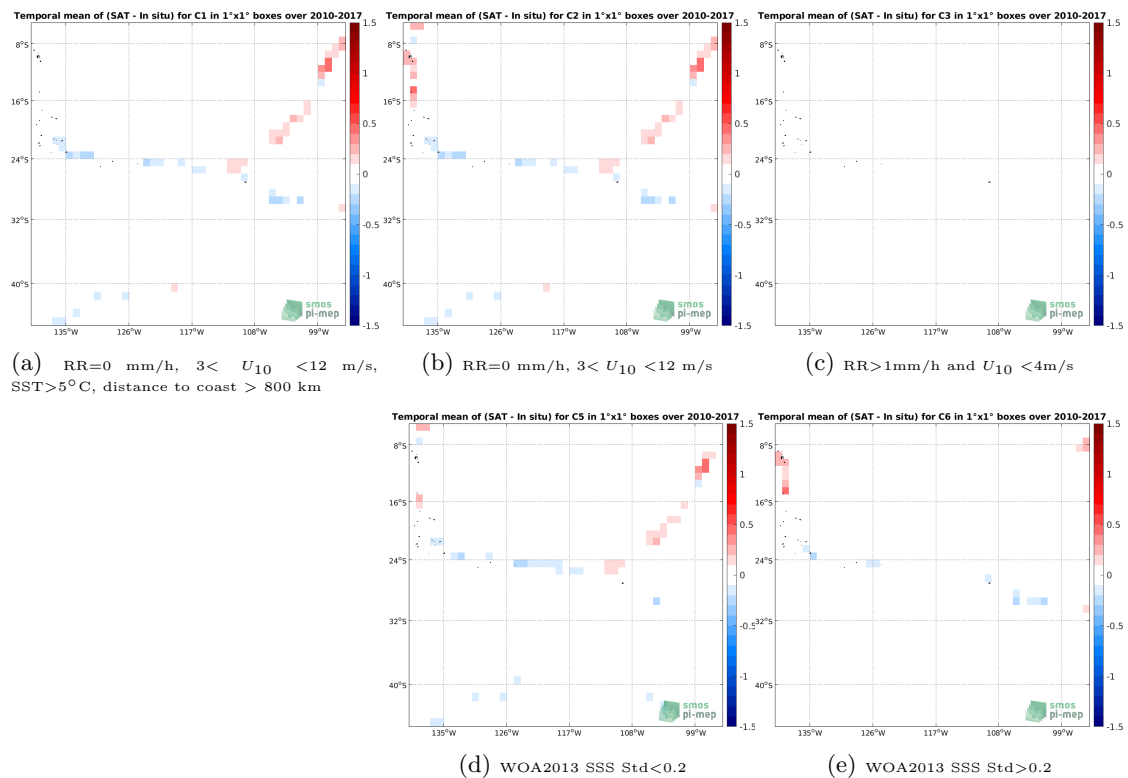
Figure 12: Temporal mean gridded over spatial boxes of size 1^\circ \times 1^\circ of \Delta SSS (CCI SSS L4 Merged-OI v2.31 - 30-day running (ESA) - TSG (GOSUD-Sailing-ship)) for 5 different subdatasets corresponding to:RR=0 mm/h, 3 < U_{10} < 12 m/s, SST >5^\circ\text{C} , distance to coast > 800 km (a), RR=0 mm/h, 3 < U_{10} < 12 m/s (b), RR >1 mm/h and U_{10} < 4 m/s (c), WOA2013 SSS Std <0.2 (d), WOA2013 SSS Std >0.2 (e).
