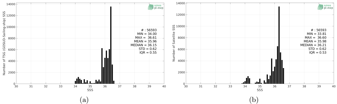
Figure 2: Histograms of SSS from TSG (GOSUD-Sailing-ship) (a) and CCI SSS L4 Merged-OI v2.31 - 30-day running (ESA) (b) considering all match-up pairs per bins of 0.1 over the OTT zone Pi-MEP region and for the full satellite product period.
