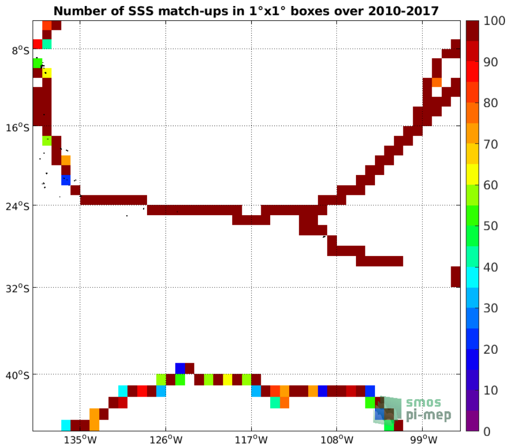
Figure 4: Number of SSS match-ups between TSG (GOSUD-Sailing-ship) SSS and the CCI SSS L4 Merged-OI v2.31 - 30-day running (ESA) SSS product for the OTT zone Pi-MEP region over 1°x1° boxes and for the full satellite product period.
