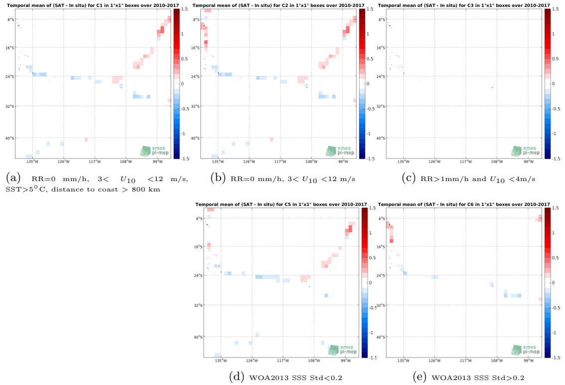
Figure 12: Temporal mean gridded over spatial boxes of size 1^\circ \times 1^\circ of \Delta SSS (CCI SSS L4 Merged-OI v2.31 - 30-day running (ESA) - TSG (GOSUD-Sailing-ship)) for 5 different subdatasets corresponding to: RR=0 mm/h, 3 < U_{10} < 12 m/s, SST > 5^\circ C , distance to coast > 800 km (a), RR=0 mm/h, 3 < U_{10} < 12 m/s (b), RR > 1 mm/h and U_{10} < 4 m/s (c), WOA2013 SSS Std < 0.2 (d), WOA2013 SSS Std > 0.2 (e).
