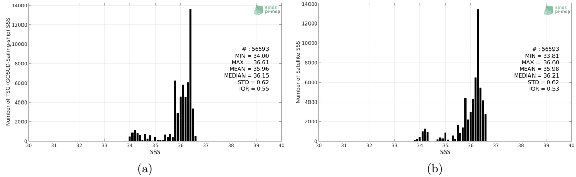
Figure 2: Histograms of SSS from TSG (GOSUD-Sailing-ship) (a) and CCI SSS L4 Merged-OI v2.31 - 30-day running (ESA) (b) considering all match-up pairs per bins of 0.1 over the OTT zone Pi-MEP region and for the full satellite product period.
