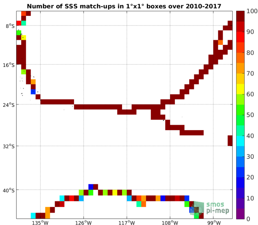
Figure 4: Number of SSS match-ups between TSG (GOSUD-Sailing-ship) SSS and the CCI L4 Merged-OI v2.31 - 30-day running (ESA) SSS product for the OTT zone Pi-MEP region over 1°x1° boxes and for the full satellite product period.
