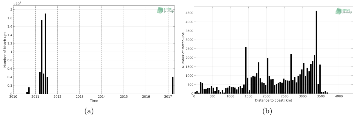
Figure 1: Number of match-ups between TSG (GOSUD-Sailing-ship) and CCI L4 Merged-OI v2.31 - 30-day running (ESA) SSS as a function of time (a) and as function of the distance to coast (b) over the OTT zone Pi-MEP region and for the full satellite product period.
