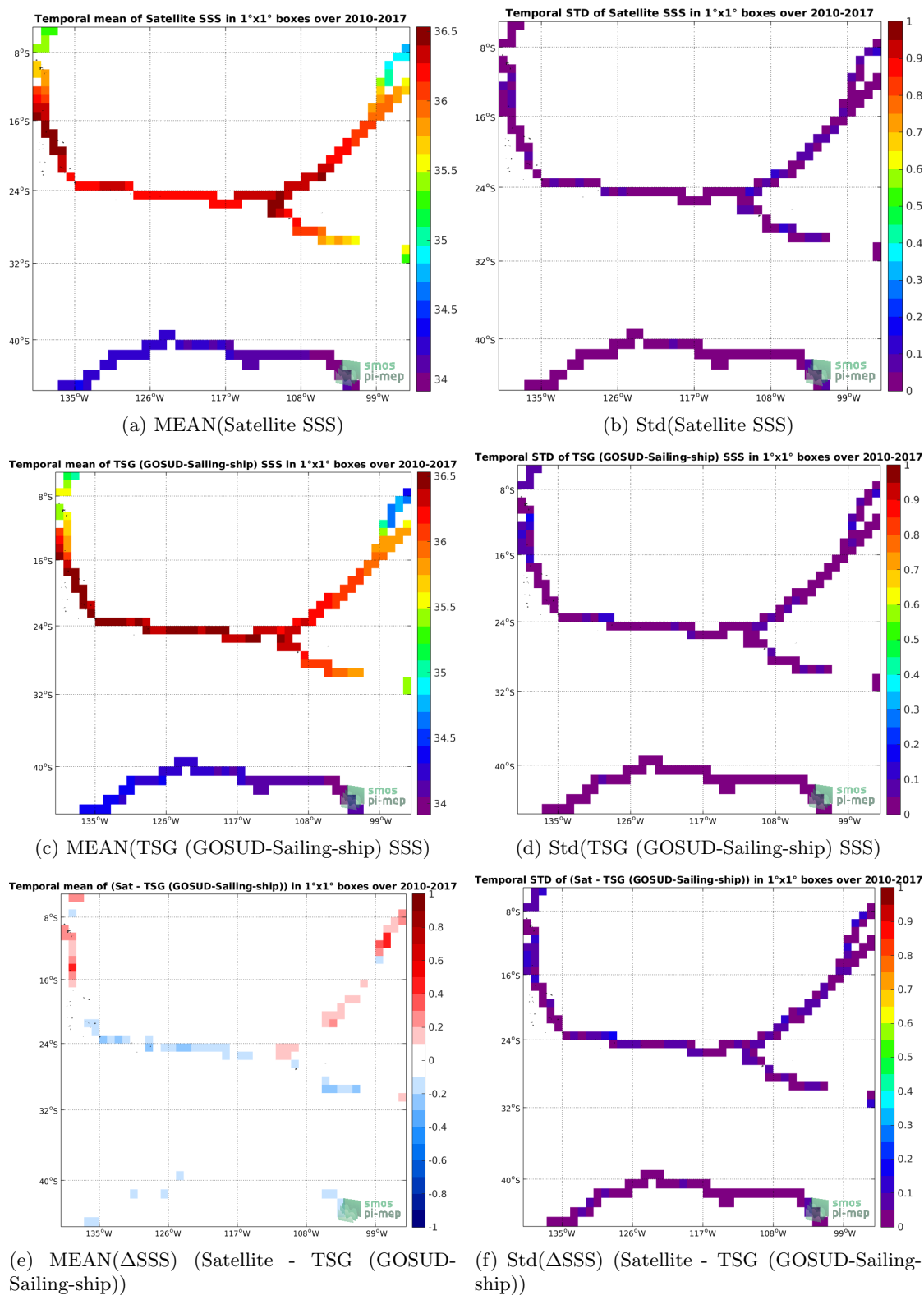
Figure 6: Temporal mean (left) and Std (right) of SSS from CCI L4 Merged-OI v2.31 - 30-day running (ESA) (top), TSG (GOSUD-Sailing-ship) (middle), and of \Delta SSS (Satellite - TSG (GOSUD-Sailing-ship)). Only match-up pairs are used to generate these maps.
