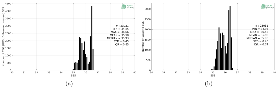
Figure 2: Histograms of SSS from TSG (GOSUD-Research-vessel) (a) and CCI SSS L4 Merged-OI v2.31 - 30-day running (ESA) (b) considering all match-up pairs per bins of 0.1 over the OTT zone Pi-MEP region and for the full satellite product period.
