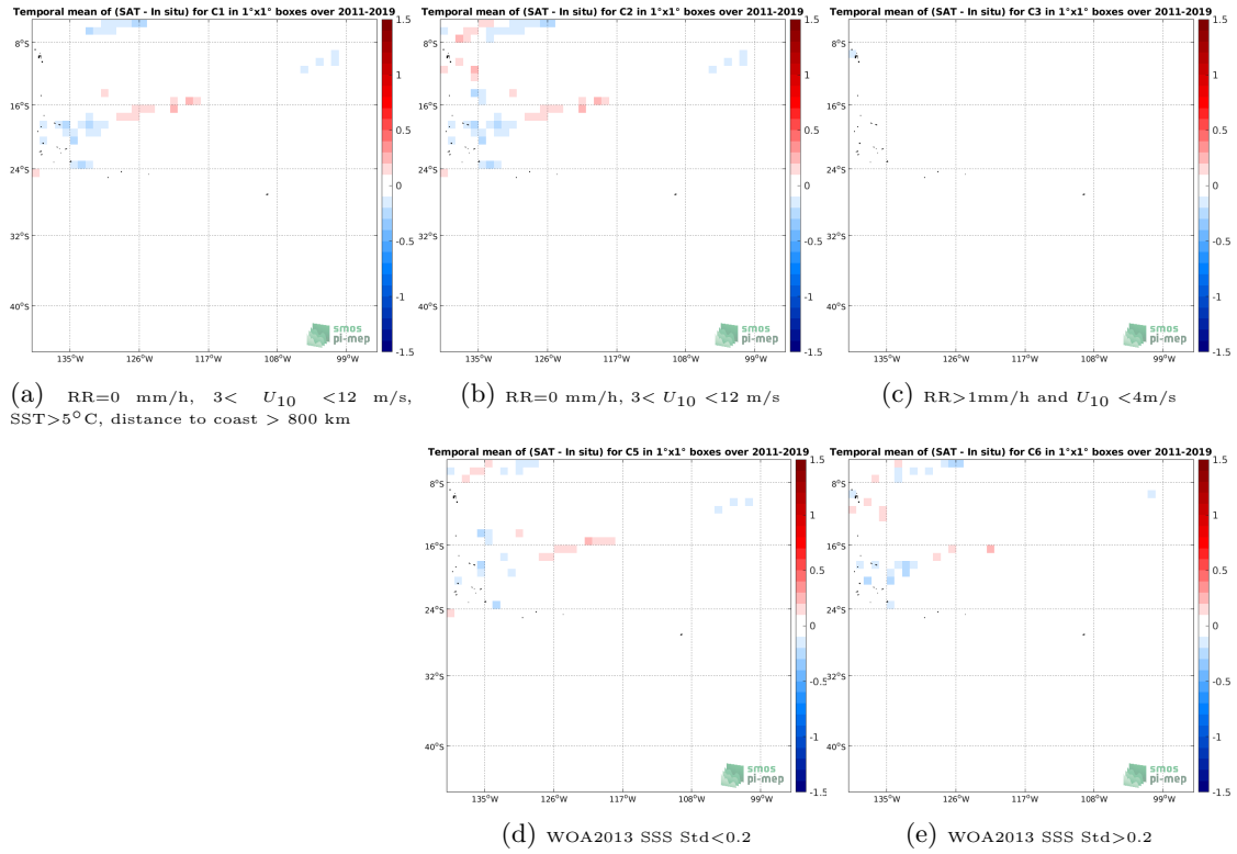
Figure 12: Temporal mean gridded over spatial boxes of size 1°x1° of \Delta SSS (CCI SSS L4 Merged-OI v2.31 - 30-day running (ESA) - TSG (GOSUD-Research-vessel)) for 5 different subdatasets corresponding to:RR=0 mm/h, 3 < U_{10} < 12 m/s, SST>5°C, distance to coast > 800 km (a), RR=0 mm/h, 3 < U_{10} < 12 m/s (b), RR>1mm/h and U_{10} < 4 m/s (c), WOA2013 SSS Std<0.2 (d), WOA2013 SSS Std>0.2 (e).
