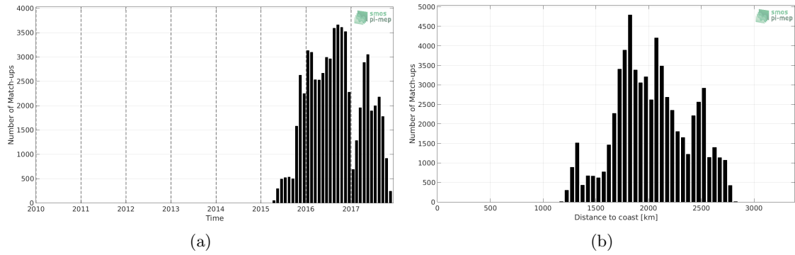
Figure 1: Number of match-ups between Surface drifters and CCI L4 Merged-OI v2.31 - 30-day running (ESA) SSS as a function of time (a) and as function of the distance to coast (b) over the OTT zone Pi-MEP region and for the full satellite product period.
