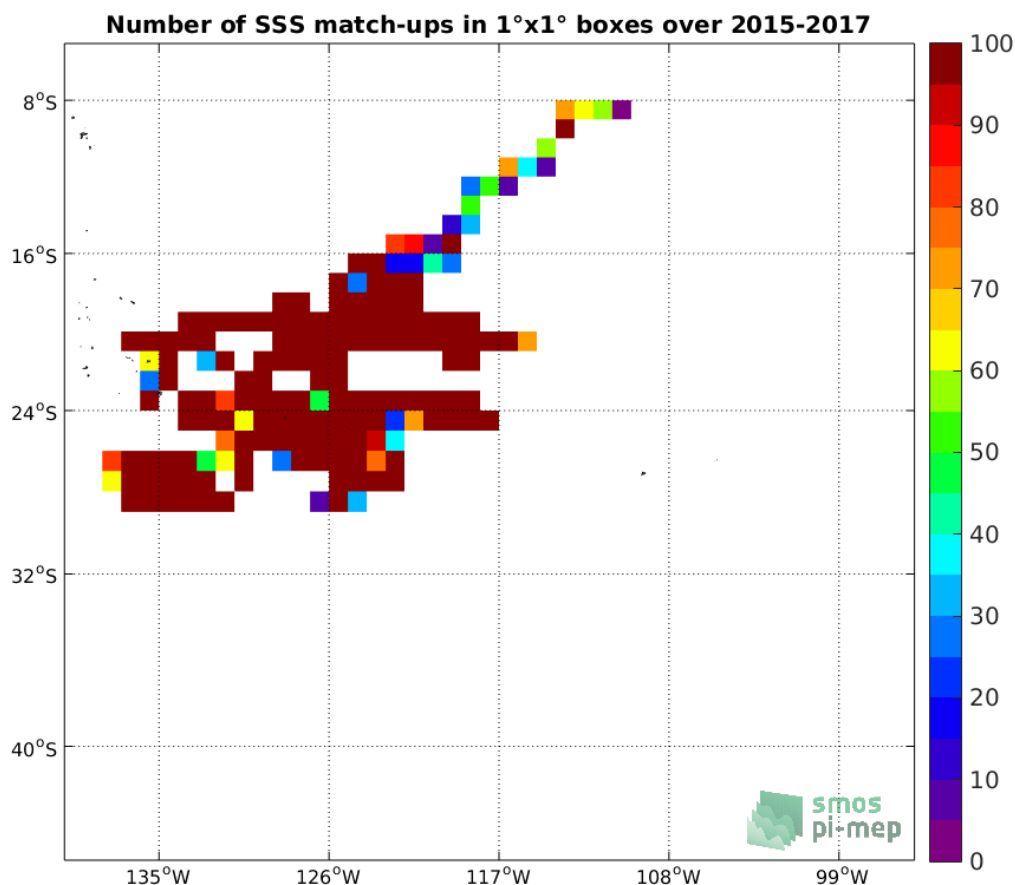
Figure 3: Number of SSS match-ups between Surface drifters SSS and the CCI L4 Merged-OI v2.31 - 30-day running (ESA) SSS product for the OTT zone Pi-MEP region over 1°x1° boxes and for the full satellite product period.
