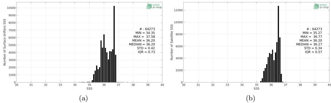
Figure 2: Histograms of SSS from Surface drifters (a) and CCI L4 Merged-OI v2.31 - 30-day running (ESA) (b) considering all match-up pairs per bins of 0.1 over the OTT zone Pi-MEP region and for the full satellite product period.
