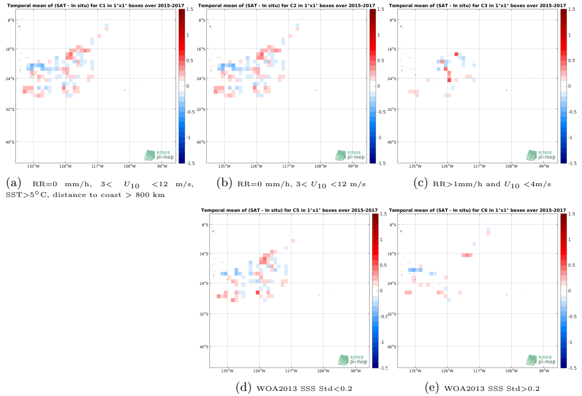
Figure 11: Temporal mean gridded over spatial boxes of size 1^\circ \times 1^\circ of \Delta SSS (CCI L4 Merged-OI v2.31 - 30-day running (ESA) - Surface drifters) for 5 different subdatasets corresponding to: RR=0 mm/h, 3 < U_{10} < 12 m/s, SST >5^\circ C, distance to coast > 800 km (a), RR=0 mm/h, 3 < U_{10} < 12 m/s (b), RR >1 mm/h and U_{10} < 4 m/s (c), WOA2013 SSS Std <0.2 (d), WOA2013 SSS Std >0.2 (e).
