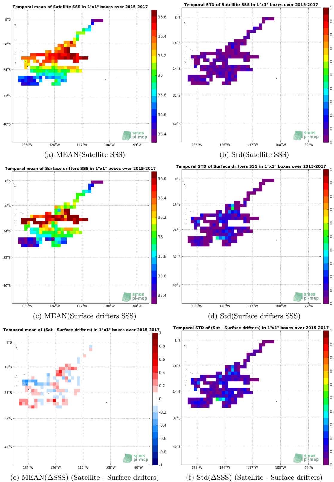
Figure 5: Temporal mean (left) and Std (right) of SSS from CCI L4 Merged-OI v2.31 - 30-day running (ESA) (top), Surface drifters (middle), and of \Delta SSS (Satellite - Surface drifters). Only match-up pairs are used to generate these maps.
