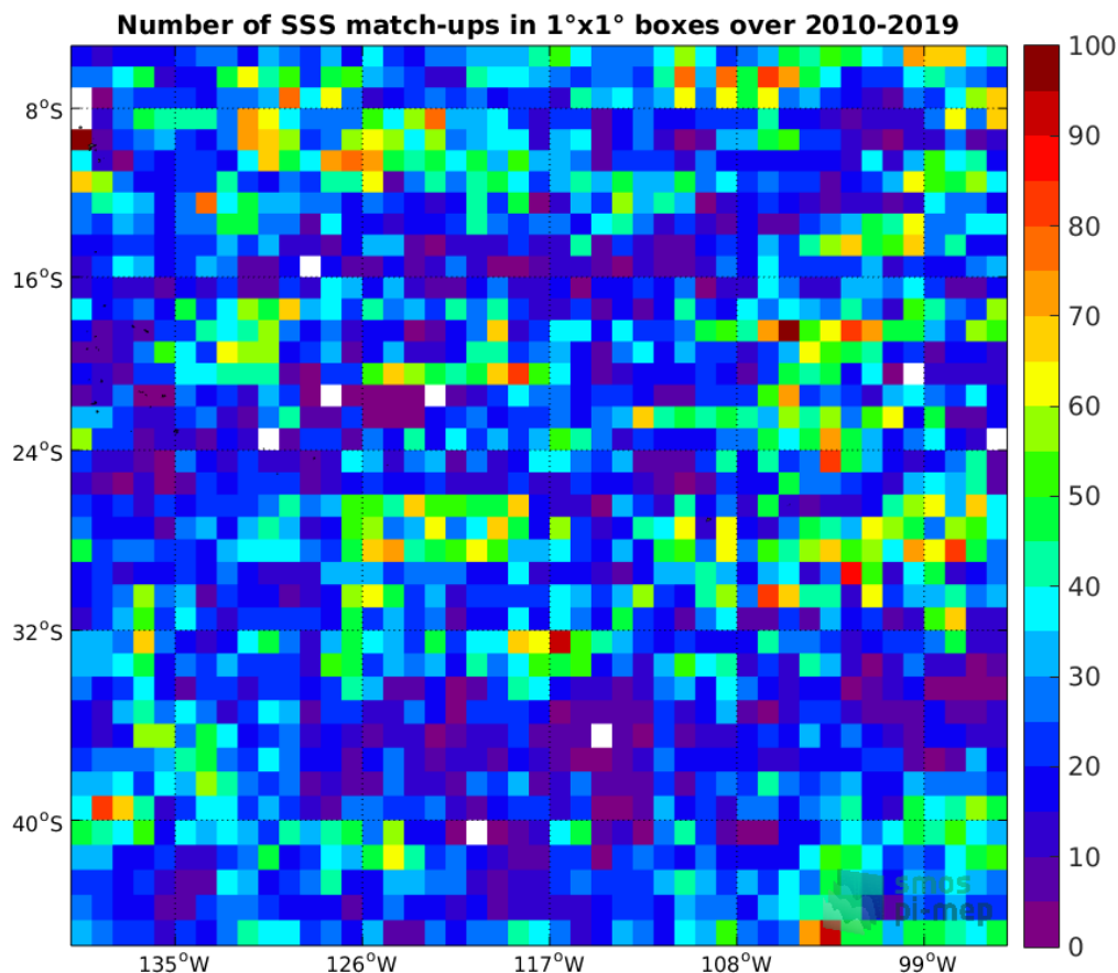
Figure 4: Number of SSS match-ups between Argo SSS and the CCI L4 Merged-OI v2.31 - 30-day running (ESA) SSS product for the OTT zone Pi-MEP region over 1°x1° boxes and for the full satellite product period.
