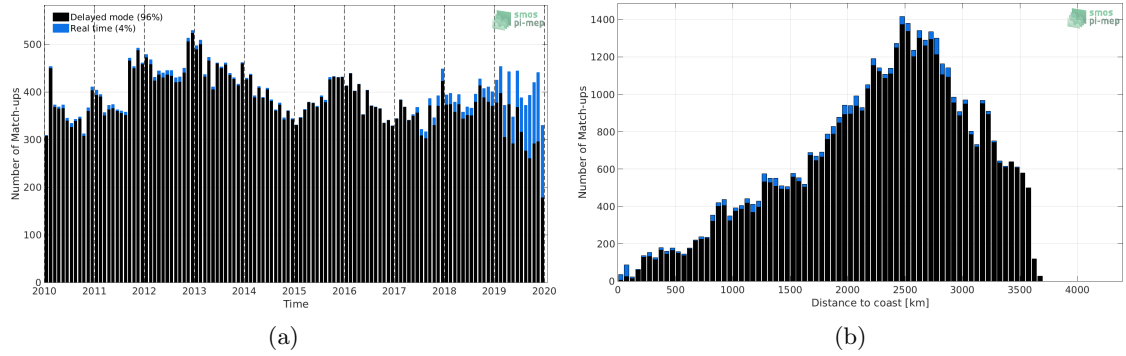
Figure 1: Number of match-ups between Argo and CCI L4 Merged-OI v2.31 - 30-day running (ESA) SSS as a function of time (a) and as function of the distance to coast (b) over the OTT zone Pi-MEP region and for the full satellite product period.
