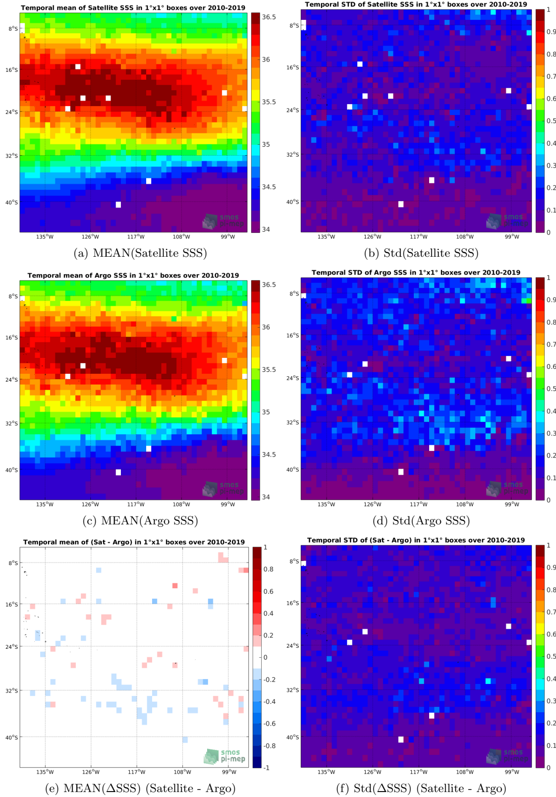
Figure 6: Temporal mean (left) and Std (right) of SSS from CCI L4 Merged-OI v2.31 - 30-day running (ESA) (top), Argo (middle), and of \Delta SSS (Satellite - Argo). Only match-up pairs are used to generate these maps.
