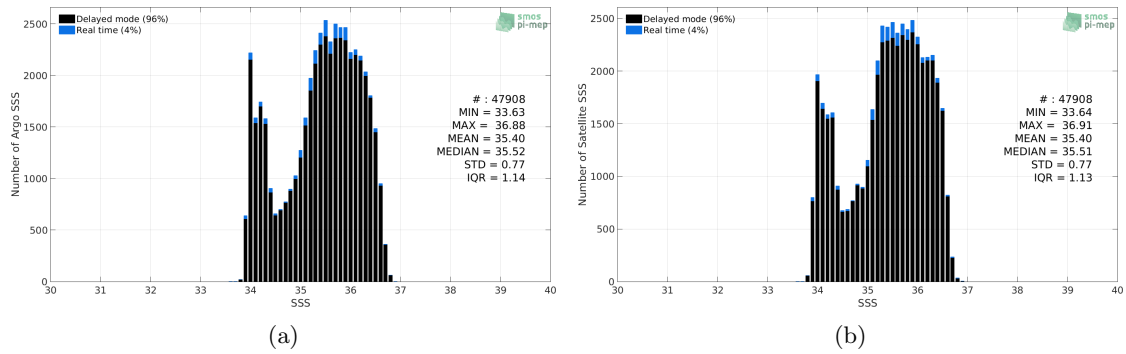
Figure 2: Histograms of SSS from Argo (a) and CCI L4 Merged-OI v2.31 - 30-day running (ESA) (b) considering all match-up pairs per bins of 0.1 over the OTT zone Pi-MEP region and for the full satellite product period.
