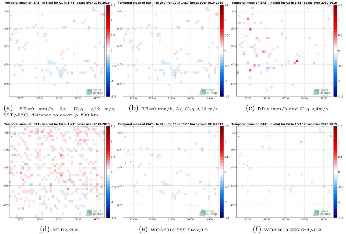
Figure 12: Temporal mean gridded over spatial boxes of size 1^\circ \times 1^\circ of \Delta SSS (CCI L4 Merged-OI v2.31 - 30-day running (ESA) - Argo) for 6 different subdatasets corresponding to: RR=0 mm/h, 3 < U_{10} < 12 m/s, SST > 5^\circ C , distance to coast > 800 km (a), RR=0 mm/h, 3 < U_{10} < 12 m/s (b), RR > 1 mm/h and U_{10} < 4 m/s (c), MLD < 20 m (d), WOA2013 SSS Std < 0.2 (e), WOA2013 SSS Std > 0.2 (f).
