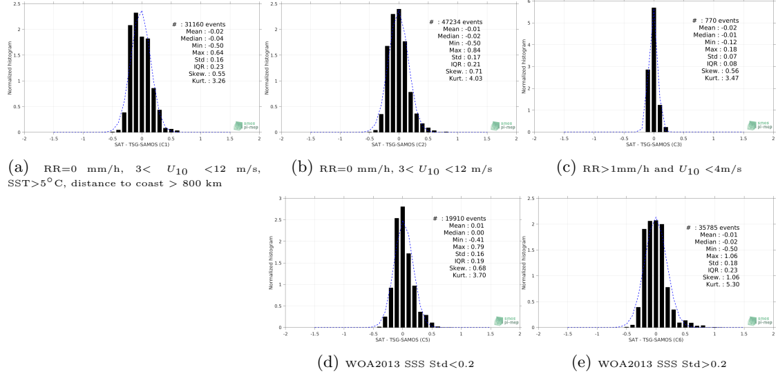
Figure 13: Normalized histogram of \Delta SSS (CCI-L4-ESA-MERGED-OI-V1.8-7DAY-RUNNING - TSG-SAMOS) for 5 different subdatasets corresponding to: RR=0 mm/h, 3 < U_{10} < 12 m/s, SST>5°C, distance to coast > 800 km (a), RR=0 mm/h, 3 < U_{10} < 12 m/s (b), RR>1mm/h and U_{10} < 4 m/s (c), WOA2013 SSS Std<0.2 (d), WOA2013 SSS Std>0.2 (e).
