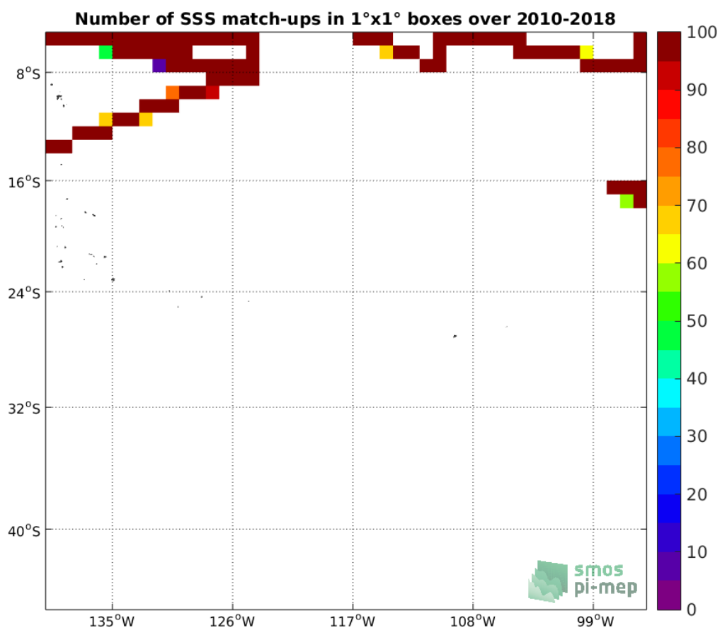
Figure 4: Number of SSS match-ups between TSG-SAMOS SSS and the CCI-L4-ESA-MERGED-OI-V1.8-7DAY-RUNNING SSS product for the OTT zone Pi-MEP region over 1°x1° boxes and for the full satellite product period.
