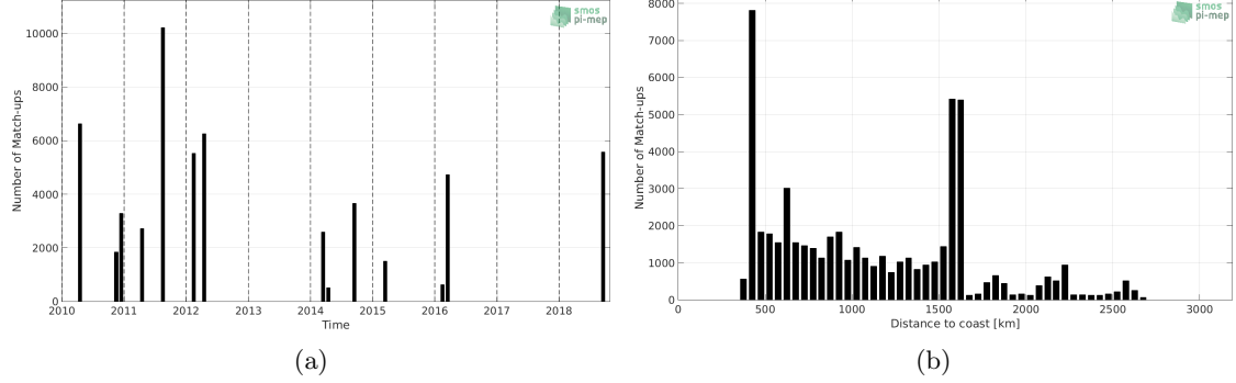
Figure 1: Number of match-ups between TSG-SAMOS and CCI-L4-ESA-MERGED-OI-V1.8-7DAY-RUNNING SSS as a function of time (a) and as function of the distance to coast (b) over the OTT zone Pi-MEP region and for the full satellite product period.
