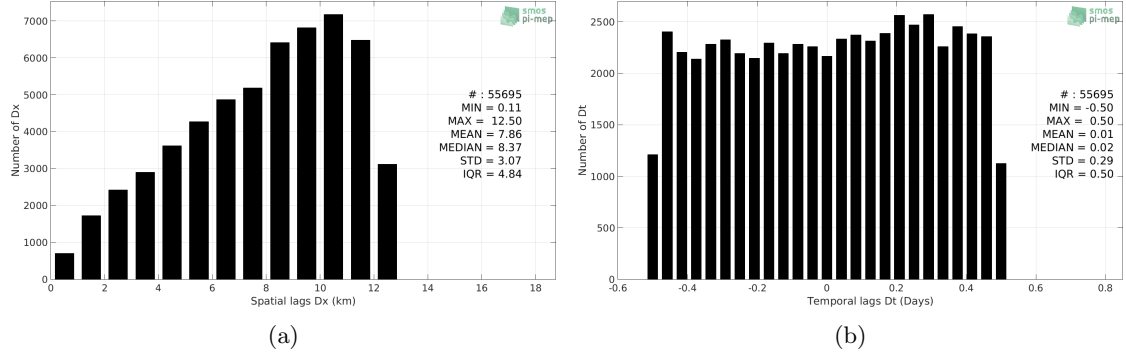
Figure 5: Histograms of the spatial (a) and temporal (b) lags between the time of the TSG-SAMOS measurements and the date of the corresponding CCI-L4-ESA-MERGED-OI-V1.8-7DAY-RUNNING SSS product.
