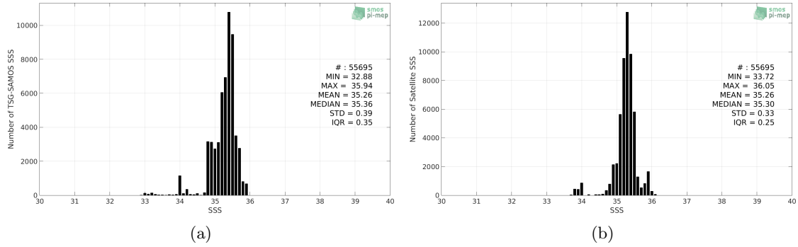
Figure 2: Histograms of SSS from TSG-SAMOS (a) and CCI-L4-ESA-MERGED-OI-V1.8-7DAY-RUNNING (b) considering all match-up pairs per bins of 0.1 over the OTT zone Pi-MEP region and for the full satellite product period.
