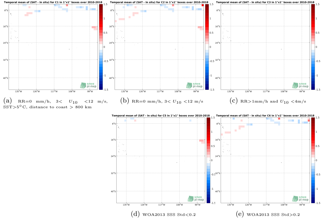
Figure 12: Temporal mean gridded over spatial boxes of size 1^\circ \times 1^\circ of \Delta SSS (CCI-L4-ESA-MERGED-OI-V1.8-7DAY-RUNNING - TSG-SAMOS) for 5 different subdatasets corresponding to: RR=0 mm/h, 3 < U_{10} < 12 m/s, SST >5^\circ\text{C} , distance to coast > 800 km (a), RR=0 mm/h, 3 < U_{10} < 12 m/s (b), RR >1 mm/h and U_{10} < 4 m/s (c), WOA2013 SSS Std <0.2 (d), WOA2013 SSS Std >0.2 (e).
