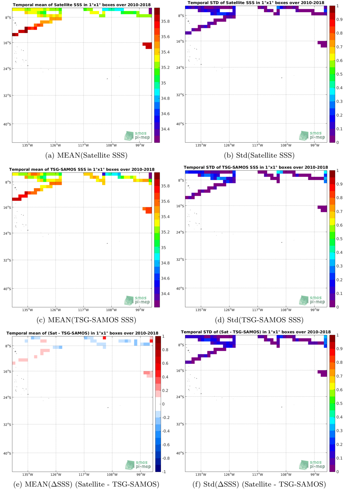
Figure 6: Temporal mean (left) and Std (right) of SSS from CCI-L4-ESA-MERGED-OI-V1.8-7DAY-RUNNING (top), TSG-SAMOS (middle), and of \Delta SSS (Satellite - TSG-SAMOS). Only match-up pairs are used to generate these maps.
