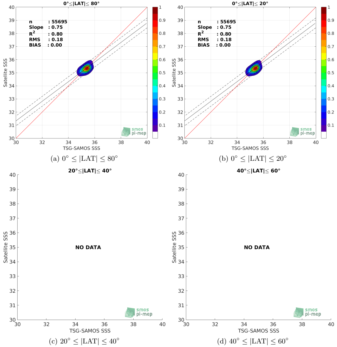
Figure 9: Contour maps of the concentration of CCI-L4-ESA-MERGED-OI-V1.8-7DAY-RUNNING SSS (y-axis) versus TSG-SAMOS SSS (x-axis) at match-up pairs for different latitude bands. For each plot, the red line shows x=y . The black thin and dashed lines indicate a linear fit through the data cloud and the \pm 95\% confidence levels, respectively. The number match-up pairs n , the slope and R^2 coefficient of the linear fit, the root mean square (RMS) and the mean bias between satellite and in situ data are indicated for each latitude band in each plots.
