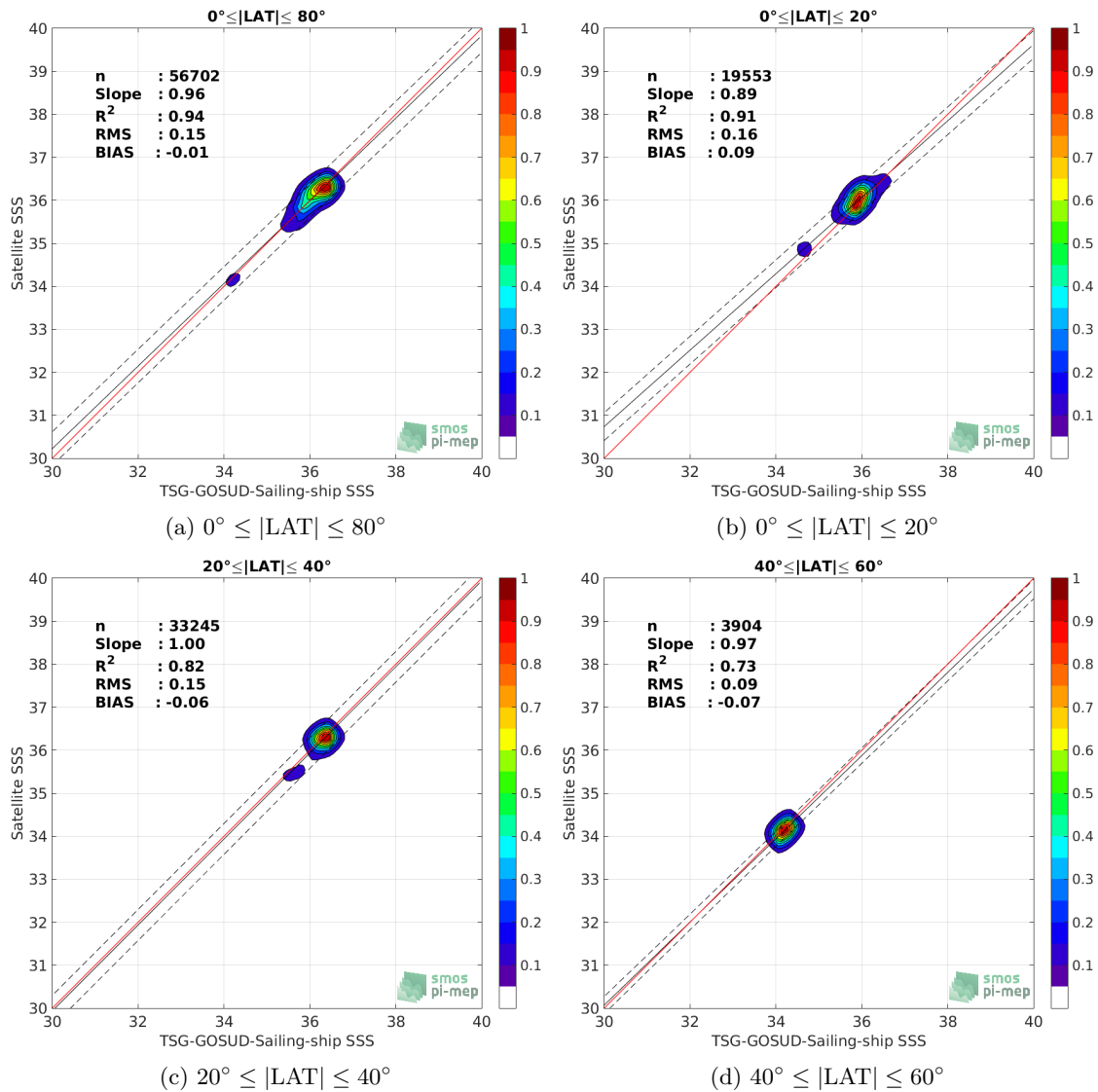
Figure 9: Contour maps of the concentration of CCI L4 Merged-OI v1.8 - 7-day running (ESA) SSS (y-axis) versus TSG-GOSUD-Sailing-ship SSS (x-axis) at match-up pairs for different latitude bands. For each plot, the red line shows x=y . The black thin and dashed lines indicate a linear fit through the data cloud and the \pm 95\% confidence levels, respectively. The number match-up pairs n , the slope and R^2 coefficient of the linear fit, the root mean square (RMS) and the mean bias between satellite and in situ data are indicated for each latitude band in each plots.
