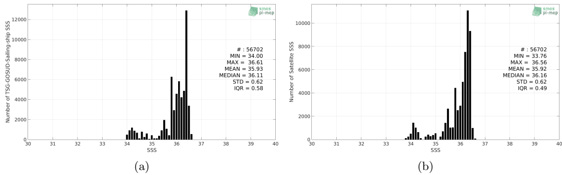
Figure 2: Histograms of SSS from TSG-GOSUD-Sailing-ship (a) and CCI L4 Merged-OI v1.8 - 7-day running (ESA) (b) considering all match-up pairs per bins of 0.1 over the OTT zone Pi-MEP region and for the full satellite product period.
