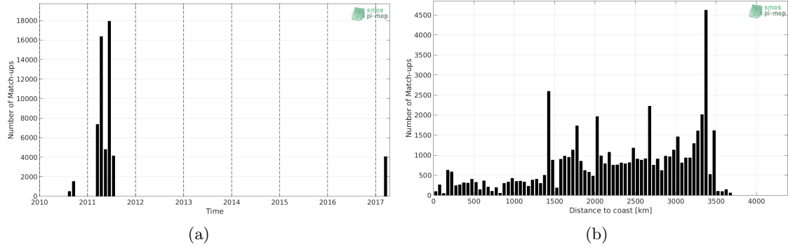
Figure 1: Number of match-ups between TSG-GOSUD-Sailing-ship and CCI L4 Merged-OI v1.8 - 7-day running (ESA) SSS as a function of time (a) and as function of the distance to coast (b) over the OTT zone Pi-MEP region and for the full satellite product period.
