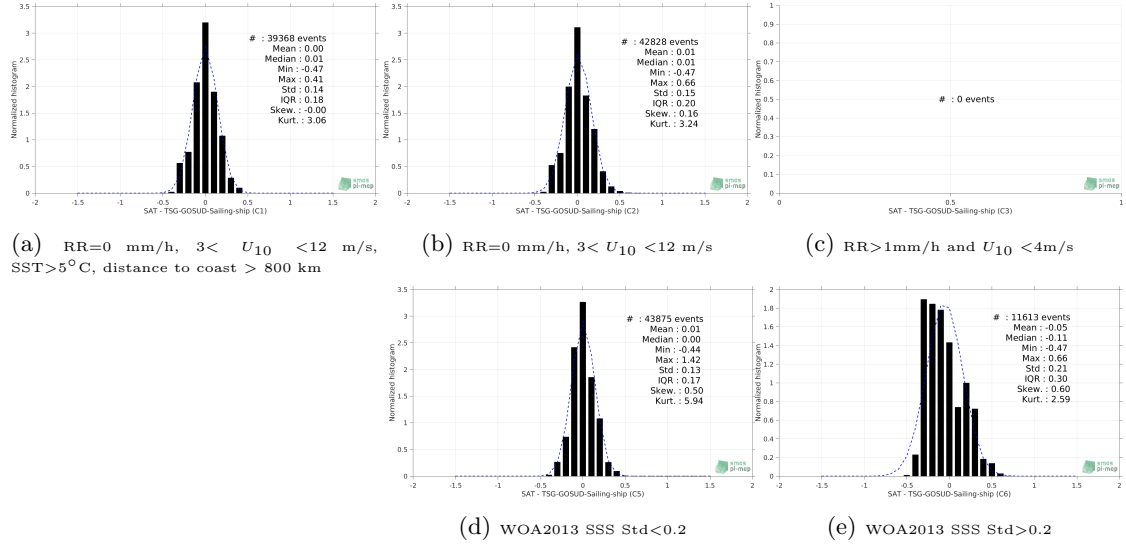
Figure 13: Normalized histogram of \Delta SSS (CCI L4 Merged-OI v1.8 - 7-day running (ESA) - TSG-GOSUD-Sailing-ship) for 5 different subdatasets corresponding to: RR=0 mm/h, 3 < U_{10} < 12 m/s, SST > 5°C, distance to coast > 800 km (a), RR=0 mm/h, 3 < U_{10} < 12 m/s (b), RR > 1mm/h and U_{10} < 4 m/s (c), WOA2013 SSS Std < 0.2 (d), WOA2013 SSS Std > 0.2 (e).
