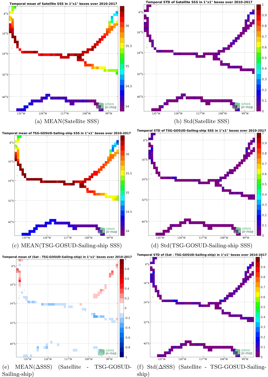
Figure 6: Temporal mean (left) and Std (right) of SSS from CCI L4 Merged-OI v1.8 - 7-day running (ESA) (top), TSG-GOSUD-Sailing-ship (middle), and of \Delta SSS (Satellite - TSG-GOSUD-Sailing-ship). Only match-up pairs are used to generate these maps.
