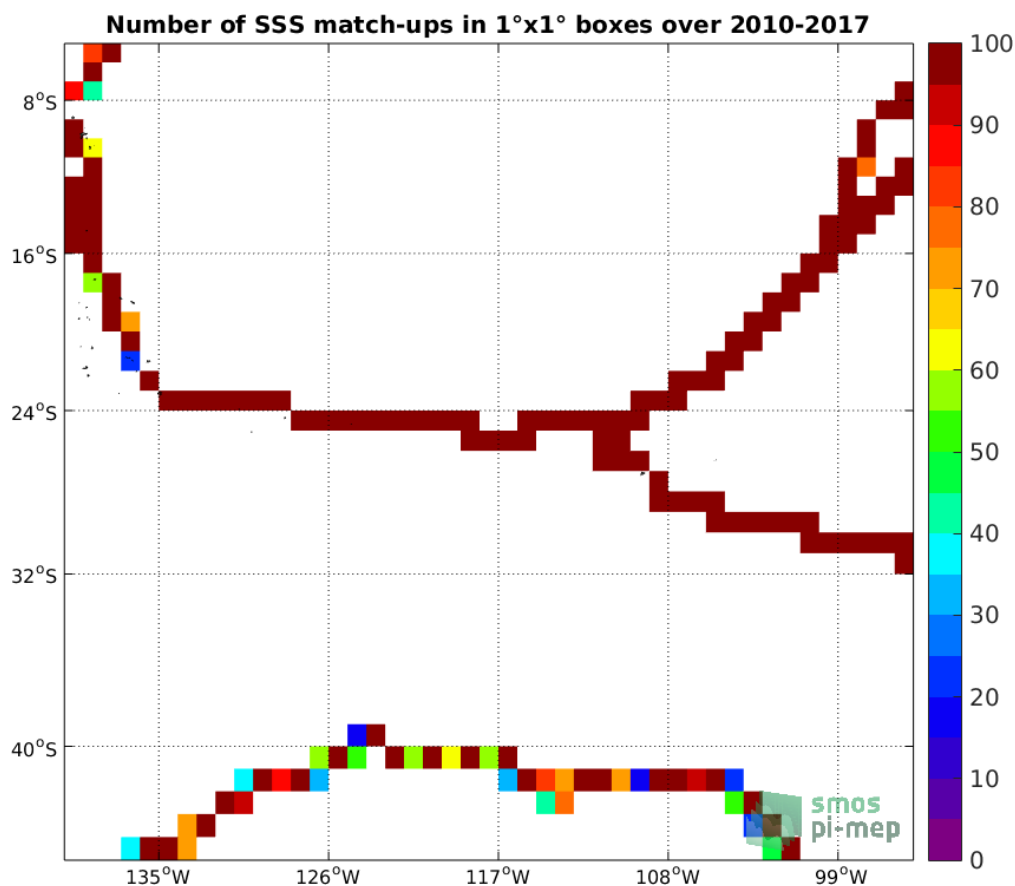
Figure 4: Number of SSS match-ups between TSG-GOSUD-Sailing-ship SSS and the CCI L4 Merged-OI v1.8 - 7-day running (ESA) SSS product for the OTT zone Pi-MEP region over 1°x1° boxes and for the full satellite product period.
