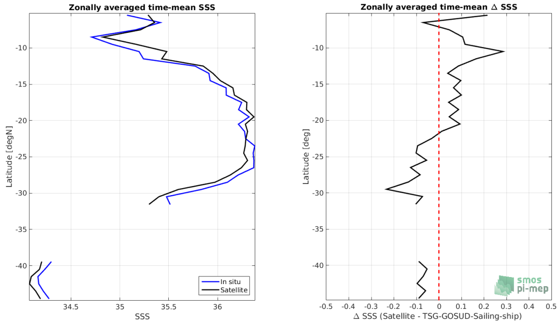
Figure 8: Left panel: Zonal mean SSS from CCI L4 Merged-OI v1.8 - 7-day running (ESA) satellite product (black) and from TSG-GOSUD-Sailing-ship (blue). Right panel: Zonal mean of \Delta SSS (Satellite - TSG-GOSUD-Sailing-ship) for all the collected Pi-MEP match-up pairs estimated over the full satellite product period.
