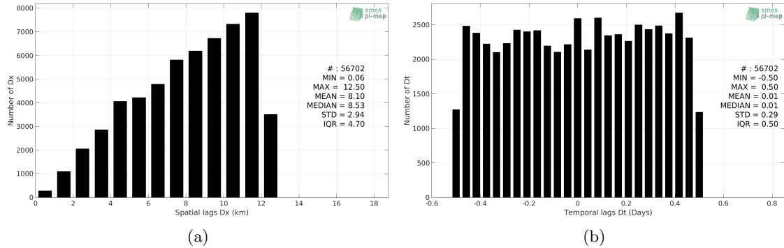
Figure 5: Histograms of the spatial (a) and temporal (b) lags between the time of the TSG-GOSUD-Sailing-ship measurements and the date of the corresponding CCI L4 Merged-OI v1.8 - 7-day running (ESA) SSS product.
