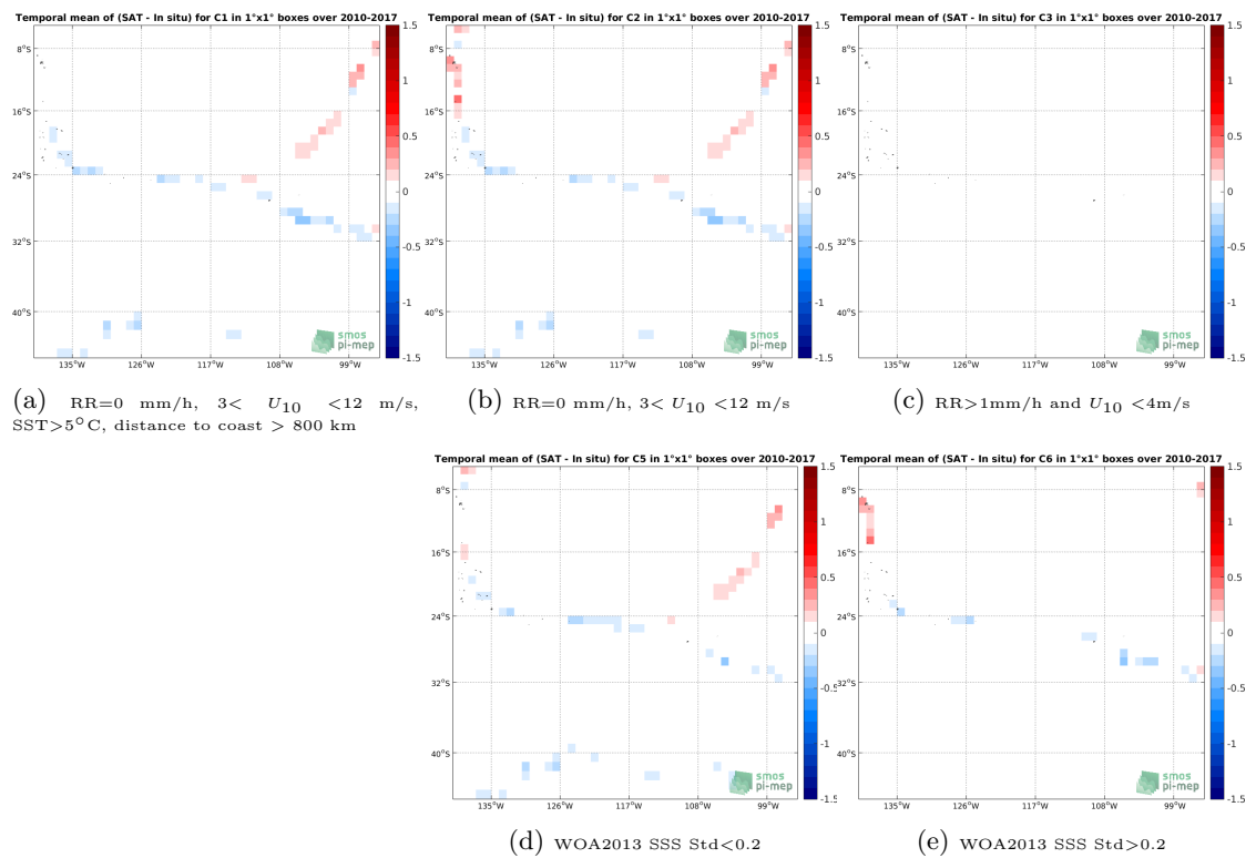
Figure 12: Temporal mean gridded over spatial boxes of size 1^\circ \times 1^\circ of \Delta SSS (CCI L4 Merged-OI v1.8 - 7-day running (ESA) - TSG-GOSUD-Sailing-ship) for 5 different subdatasets corresponding to: RR=0 mm/h, 3 < U_{10} < 12 m/s, SST > 5^\circ C , distance to coast > 800 km (a), RR=0 mm/h, 3 < U_{10} < 12 m/s (b), RR > 1 mm/h and U_{10} < 4 m/s (c), WOA2013 SSS Std < 0.2 (d), WOA2013 SSS Std > 0.2 (e).
