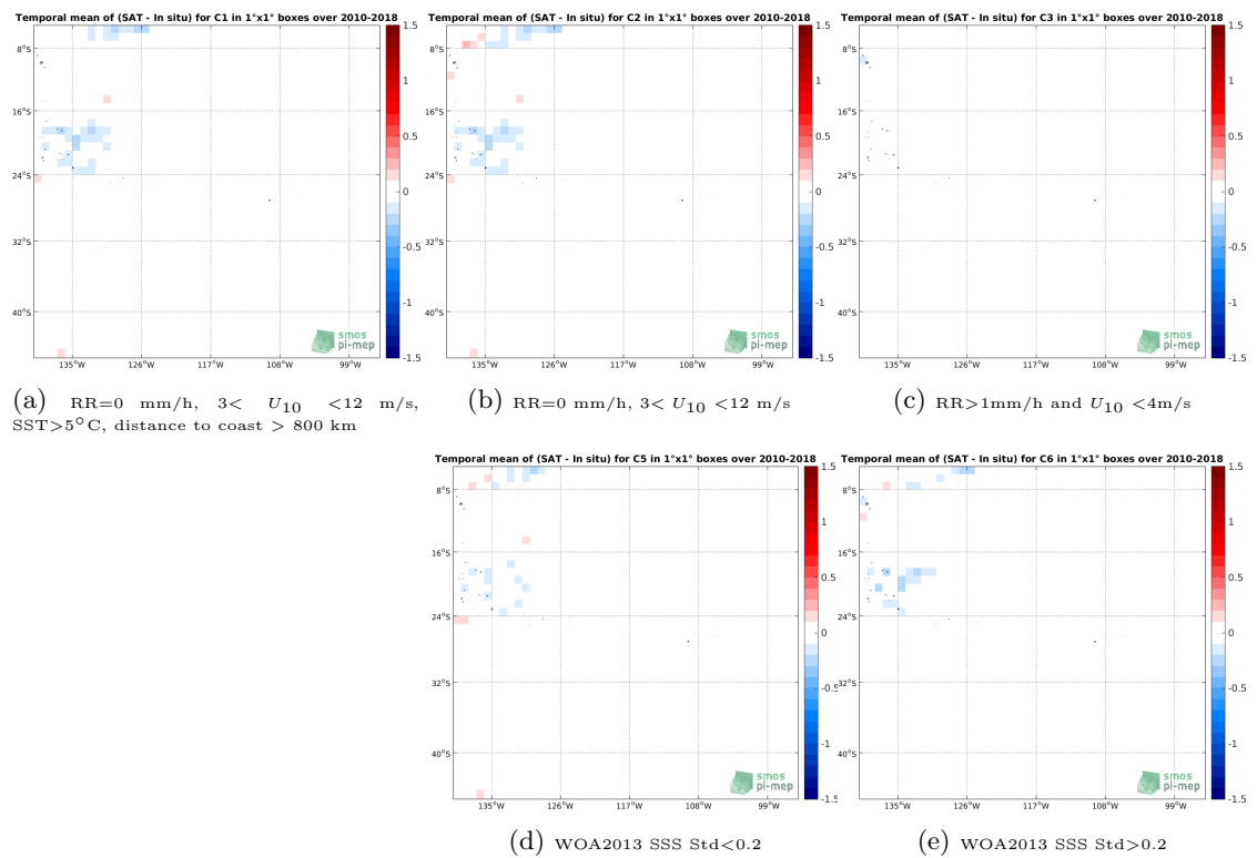
Figure 12: Temporal mean gridded over spatial boxes of size 1^\circ \times 1^\circ of \Delta SSS (CCI-L4-ESA-MERGED-OI-V1.8-7DAY-RUNNING - TSG-GOSUD-Research-vessel) for 5 different sub-datasets corresponding to:RR=0 mm/h, 3 < U_{10} < 12 m/s, SST >5^\circ\text{C} , distance to coast > 800 km (a), RR=0 mm/h, 3 < U_{10} < 12 m/s (b), RR >1 mm/h and U_{10} < 4 m/s (c), WOA2013 SSS Std <0.2 (d), WOA2013 SSS Std >0.2 (e).
