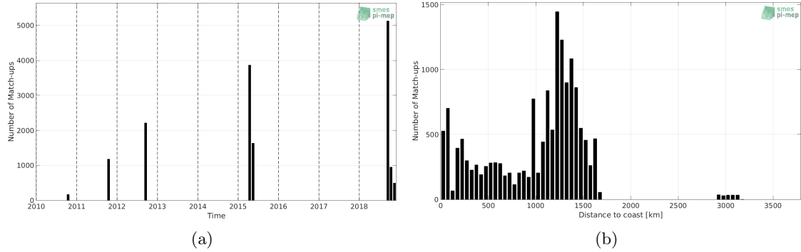
Figure 1: Number of match-ups between TSG-GOSUD-Research-vessel and CCI-L4-ESA-MERGED-OI-V1.8-7DAY-RUNNING SSS as a function of time (a) and as function of the distance to coast (b) over the OTT zone Pi-MEP region and for the full satellite product period.
