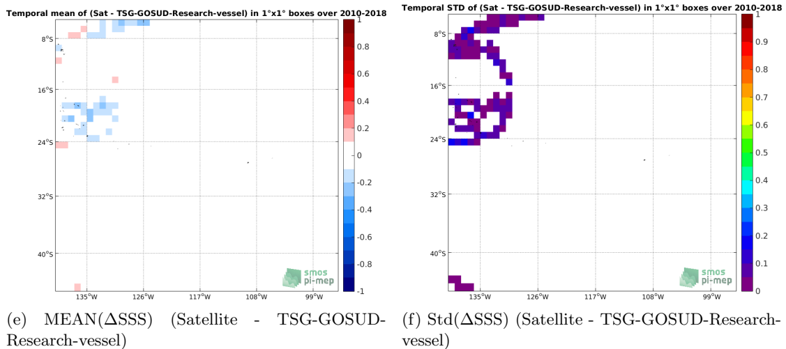
Figure 6: Temporal mean (left) and Std (right) of SSS from CCI-L4-ESA-MERGED-OI-V1.8-7DAY-RUNNING (top), TSG-GOSUD-Research-vessel (middle), and of \Delta SSS (Satellite - TSG-GOSUD-Research-vessel). Only match-up pairs are used to generate these maps.
