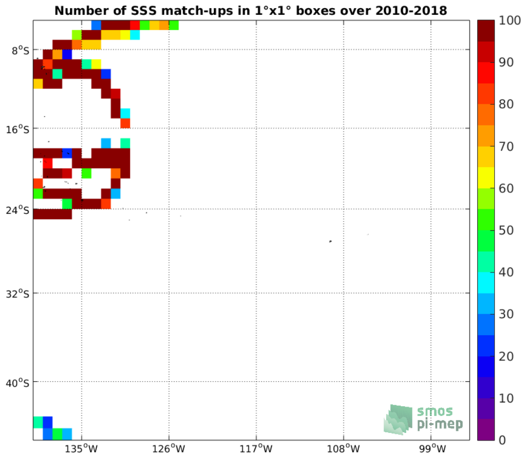
Figure 4: Number of SSS match-ups between TSG-GOSUD-Research-vessel SSS and the CCI-L4-ESA-MERGED-OI-V1.8-7DAY-RUNNING SSS product for the OTT zone Pi-MEP region over 1°x1° boxes and for the full satellite product period.
