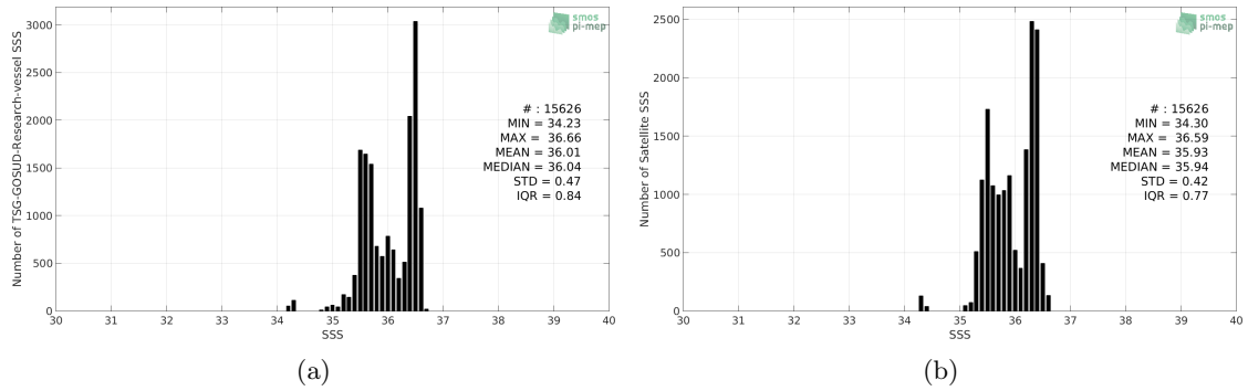
Figure 2: Histograms of SSS from TSG-GOSUD-Research-vessel (a) and CCI-L4-ESA-MERGED-OI-V1.8-7DAY-RUNNING (b) considering all match-up pairs per bins of 0.1 over the OTT zone Pi-MEP region and for the full satellite product period.
