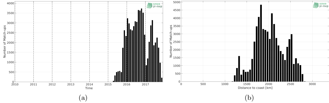
Figure 1: Number of match-ups between Surface drifters and CCI L4 Merged-OI v1.8 - 7-day running (ESA) SSS as a function of time (a) and as function of the distance to coast (b) over the OTT zone Pi-MEP region and for the full satellite product period.
