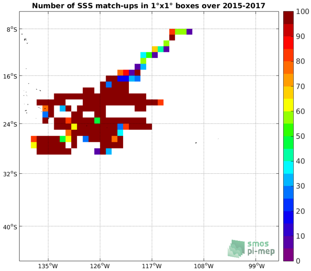
Figure 3: Number of SSS match-ups between Surface drifters SSS and the CCI L4 Merged-OI v1.8 - 7-day running (ESA) SSS product for the OTT zone Pi-MEP region over 1°x1° boxes and for the full satellite product period.
