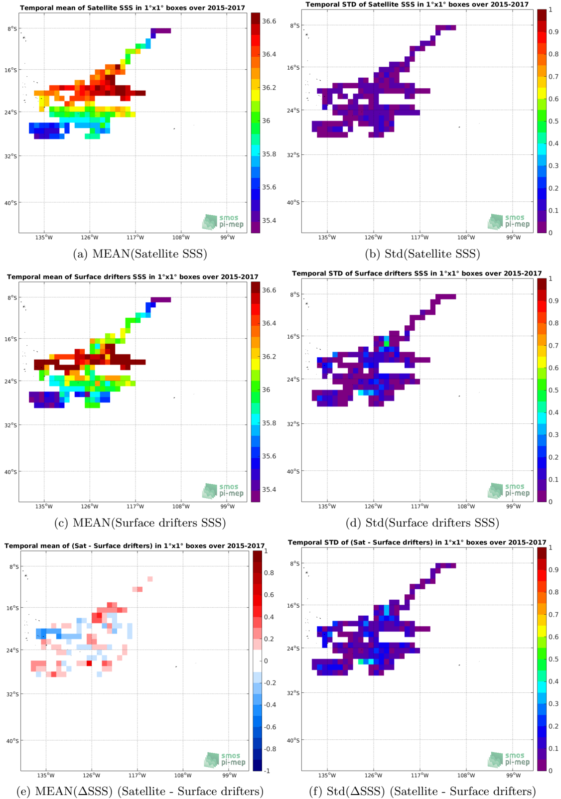
Figure 5: Temporal mean (left) and Std (right) of SSS from CCI L4 Merged-OI v1.8 - 7-day running (ESA) (top), Surface drifters (middle), 20 and of \Delta SSS (Satellite - Surface drifters). Only match-up pairs are used to generate these maps.
