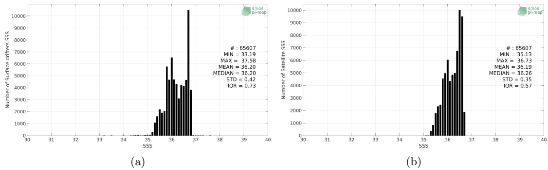
Figure 2: Histograms of SSS from Surface drifters (a) and CCI L4 Merged-OI v1.8 - 7-day running (ESA) (b) considering all match-up pairs per bins of 0.1 over the OTT zone Pi-MEP region and for the full satellite product period.
