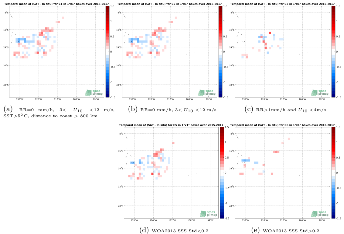
Figure 11: Temporal mean gridded over spatial boxes of size 1^\circ \times 1^\circ of \Delta SSS (CCI L4 Merged-OI v1.8 - 7-day running (ESA) - Surface drifters) for 5 different subdatasets corresponding to:RR=0 mm/h, 3 < U_{10} < 12 m/s, SST > 5^\circ\text{C} , distance to coast > 800 km (a), RR=0 mm/h, 3 < U_{10} < 12 m/s (b), RR > 1 mm/h and U_{10} < 4 m/s (c), WOA2013 SSS Std < 0.2 (d), WOA2013 SSS Std > 0.2 (e).
