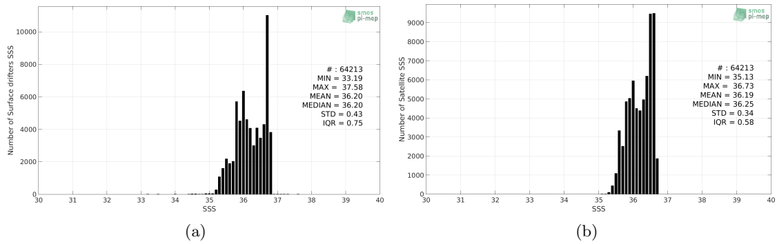
Figure 2: Histograms of SSS from Surface drifters (a) and CCI-L4-ESA-MERGED-OI-V1.8-7DAY-RUNNING (b) considering all match-up pairs per bins of 0.1 over the OTT zone Pi-MEP region and for the full satellite product period.
