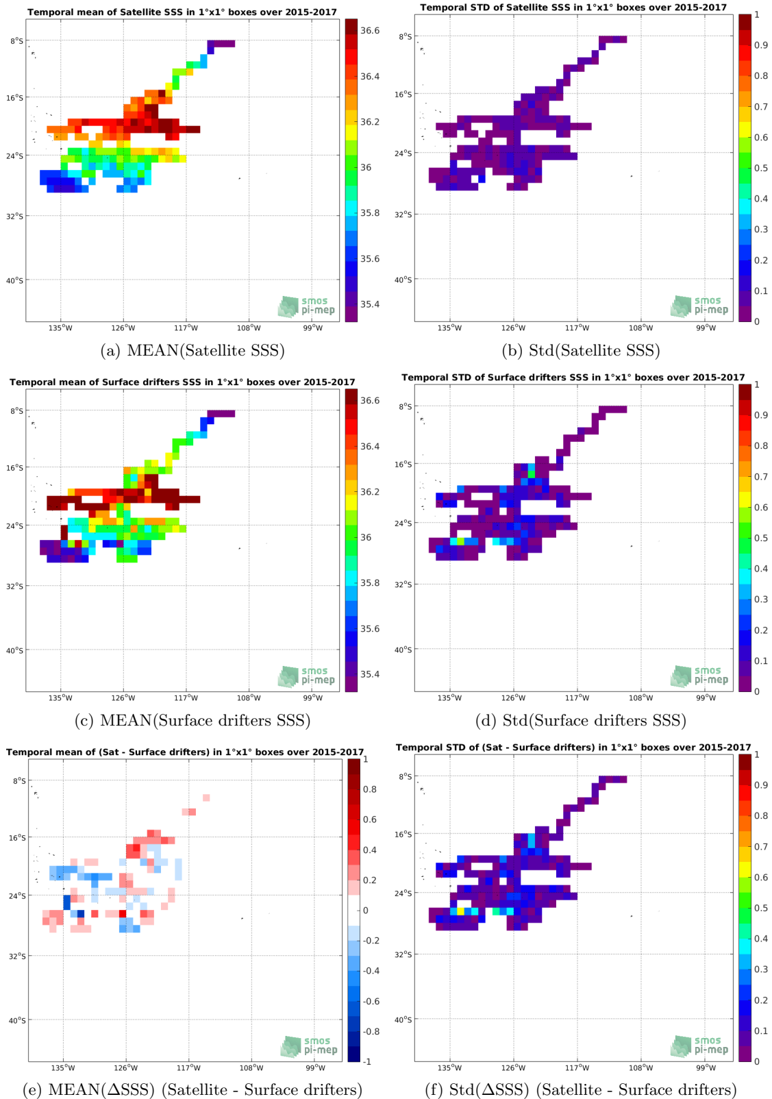
Figure 5: Temporal mean (left) and Std (right) of SSS from CCI-L4-ESA-MERGED-OI-V1.8-7DAY-RUNNING (top), Surface drifters (middle), and of \Delta SSS (Satellite - Surface drifters). Only match-up pairs are used to generate these maps.
