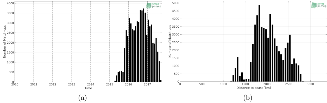
Figure 1: Number of match-ups between Surface drifters and CCI-L4-ESA-MERGED-OI-V1.8-7DAY-RUNNING SSS as a function of time (a) and as function of the distance to coast (b) over the OTT zone Pi-MEP region and for the full satellite product period.
