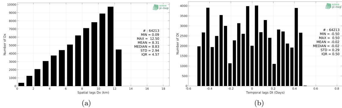
Figure 4: Histograms of the spatial (a) and temporal (b) lags between the time of the Surface drifters measurements and the date of the corresponding CCI-L4-ESA-MERGED-OI-V1.8-7DAY-RUNNING SSS product.
