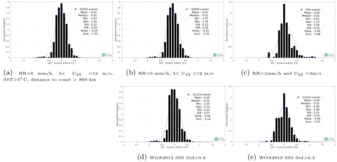
Figure 12: Normalized histogram of \Delta SSS (CCI-L4-ESA-MERGED-OI-V1.8-7DAY-RUNNING - Surface drifters) for 5 different subdatasets corresponding to: RR=0 mm/h, 3 < U_{10} < 12 m/s, SST > 5°C, distance to coast > 800 km (a), RR=0 mm/h, 3 < U_{10} < 12 m/s (b), RR > 1mm/h and U_{10} < 4 m/s (c), WOA2013 SSS Std < 0.2 (d), WOA2013 SSS Std > 0.2 (e).
