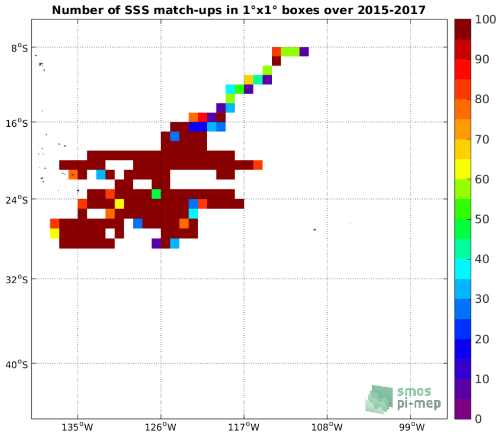
Figure 3: Number of SSS match-ups between Surface drifters SSS and the CCI-L4-ESA-MERGED-OI-V1.8-7DAY-RUNNING SSS product for the OTT zone Pi-MEP region over 1°x1° boxes and for the full satellite product period.
