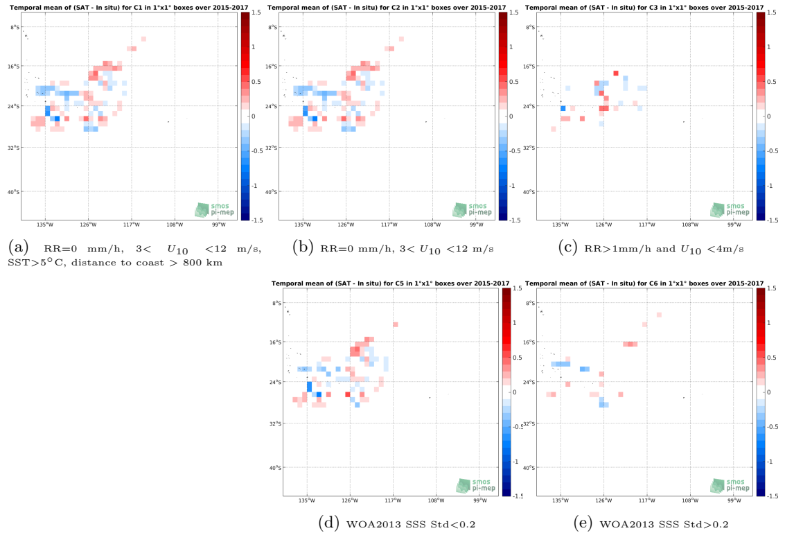
Figure 11: Temporal mean gridded over spatial boxes of size 1^\circ \times 1^\circ of \Delta SSS (CCI-L4-ESAMERGED-OI-V1.8-7DAY-RUNNING - Surface drifters) for 5 different subdatasets corresponding to:RR=0 mm/h, 3 < U_{10} < 12 m/s, SST >5^\circ C, distance to coast > 800 km (a), RR=0 mm/h, 3 < U_{10} < 12 m/s (b), RR >1 mm/h and U_{10} < 4 m/s (c), WOA2013 SSS Std <0.2 (d), WOA2013 SSS Std >0.2 (e).
