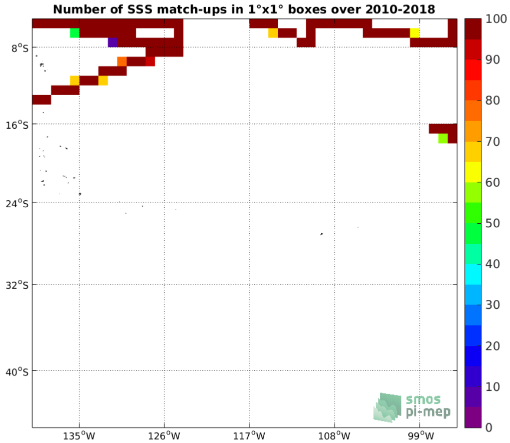
Figure 4: Number of SSS match-ups between TSG-SAMOS SSS and the CCI-L4-ESA-MERGED-OI-V1.8-30DAY-RUNNING SSS product for the OTT zone Pi-MEP region over 1°x1° boxes and for the full satellite product period.
