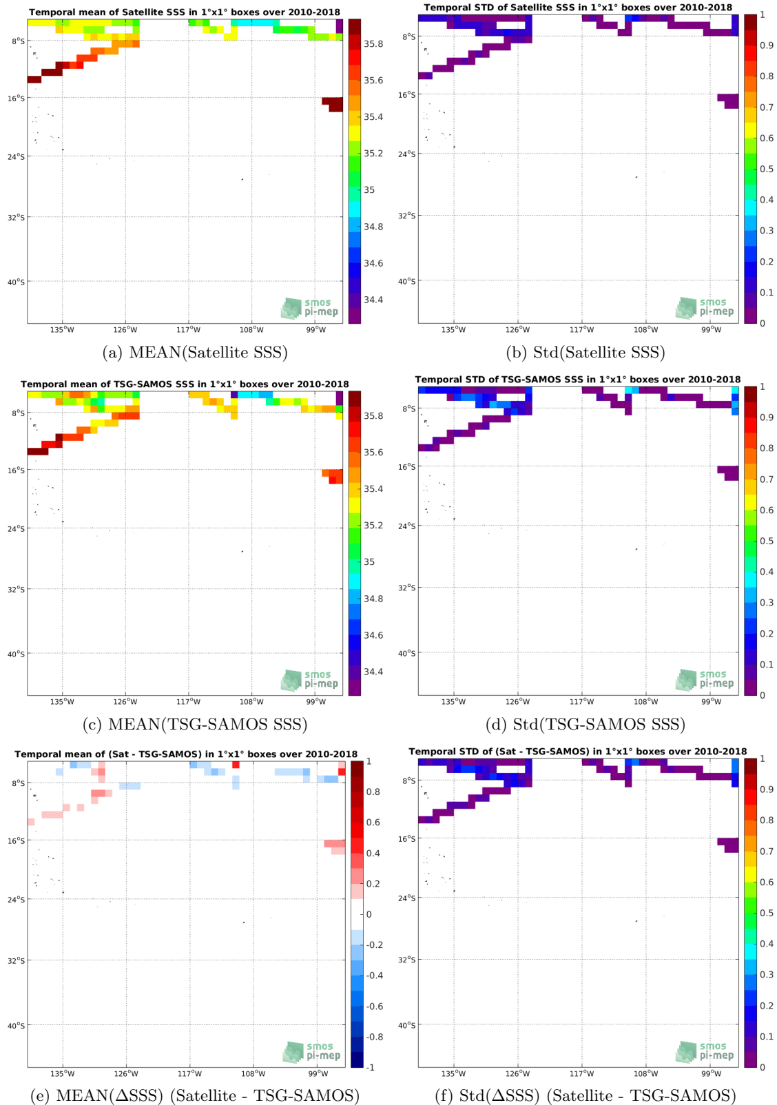
Figure 6: Temporal mean (left) and Std (right) of SSS from CCI-L4-ESA-MERGED-OI-V1.8-30DAY-RUNNING (top), TSG-SAMOS (middle), and of \Delta SSS (Satellite - TSG-SAMOS). Only match-up pairs are used to generate these maps.
