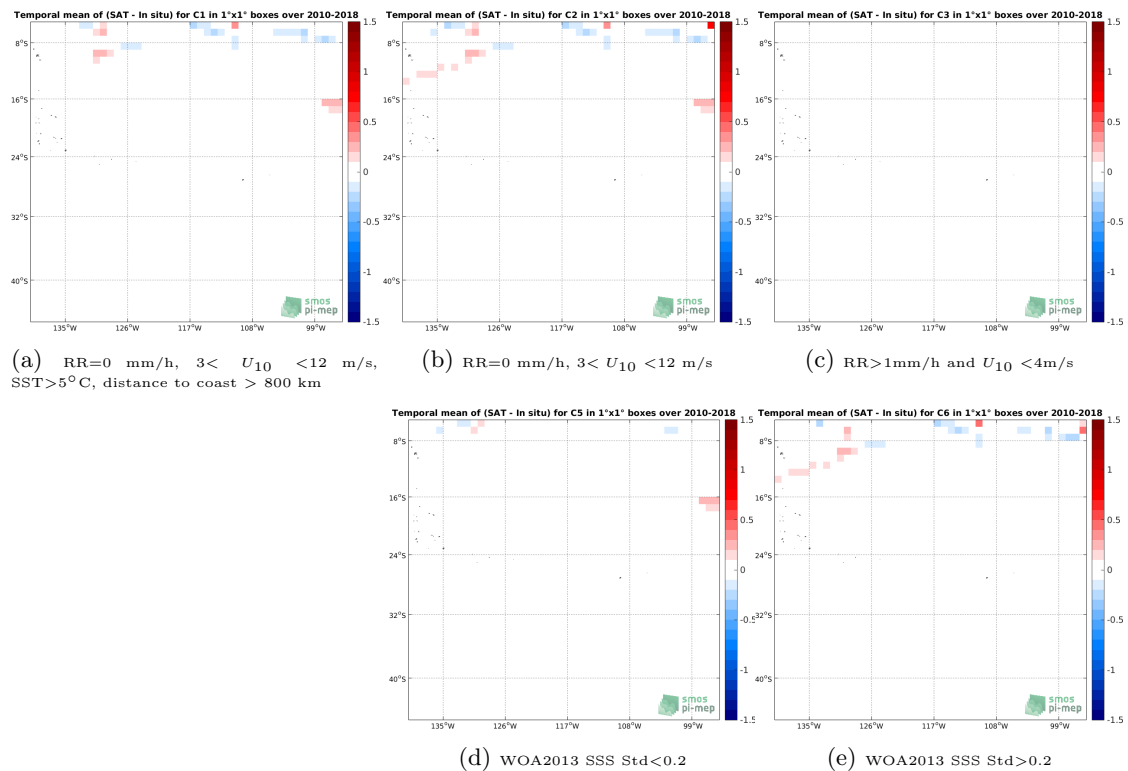
Figure 12: Temporal mean gridded over spatial boxes of size 1^\circ \times 1^\circ of \Delta SSS (CCI-L4-ESA-MERGED-OI-V1.8-30DAY-RUNNING - TSG-SAMOS) for 5 different subdatasets corresponding to:RR=0 mm/h, 3 < U_{10} < 12 m/s, SST >5^\circ C, distance to coast > 800 km (a), RR=0 mm/h, 3 < U_{10} < 12 m/s (b), RR >1 mm/h and U_{10} < 4 m/s (c), WOA2013 SSS Std <0.2 (d), WOA2013 SSS Std >0.2 (e).
