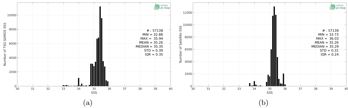
Figure 2: Histograms of SSS from TSG-SAMOS (a) and CCI-L4-ESA-MERGED-OI-V1.8-30DAY-RUNNING (b) considering all match-up pairs per bins of 0.1 over the OTT zone Pi-MEP region and for the full satellite product period.
