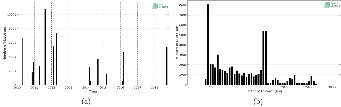
Figure 1: Number of match-ups between TSG-SAMOS and CCI-L4-ESA-MERGED-OI-V1.8-30DAY-RUNNING SSS as a function of time (a) and as function of the distance to coast (b) over the OTT zone Pi-MEP region and for the full satellite product period.
