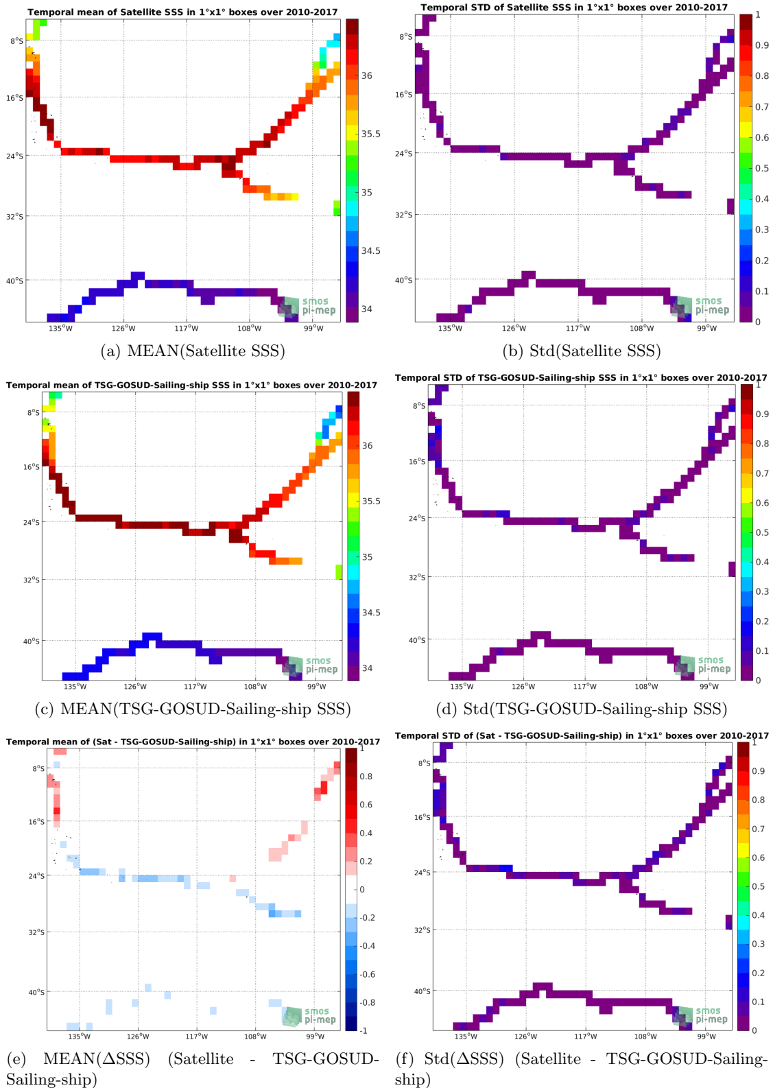
Figure 6: Temporal mean (left) and Std (right) of SSS from CCI-L4-ESA-MERGED-OI-V1.8-30DAY-RUNNING (top), TSG-GOSUD-Sailing-ship (middle), and of \Delta SSS (Satellite - TSG-GOSUD-Sailing-ship). Only match-up pairs are used to generate these maps.
