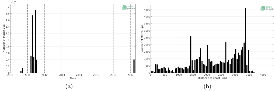
Figure 1: Number of match-ups between TSG-GOSUD-Sailing-ship and CCI-L4-ESA-MERGED-OI-V1.8-30DAY-RUNNING SSS as a function of time (a) and as function of the distance to coast (b) over the OTT zone Pi-MEP region and for the full satellite product period.
