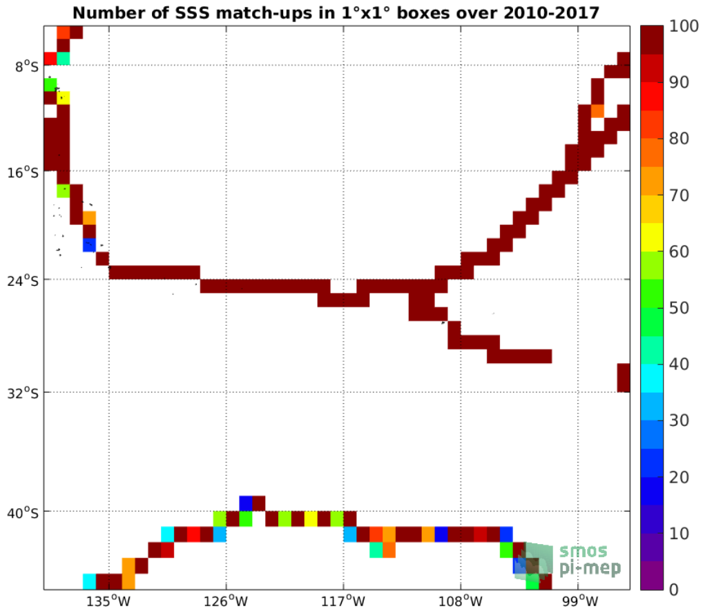
Figure 4: Number of SSS match-ups between TSG-GOSUD-Sailing-ship SSS and the CCI-L4-ESA-MERGED-OI-V1.8-30DAY-RUNNING SSS product for the OTT zone Pi-MEP region over 1°x1° boxes and for the full satellite product period.
