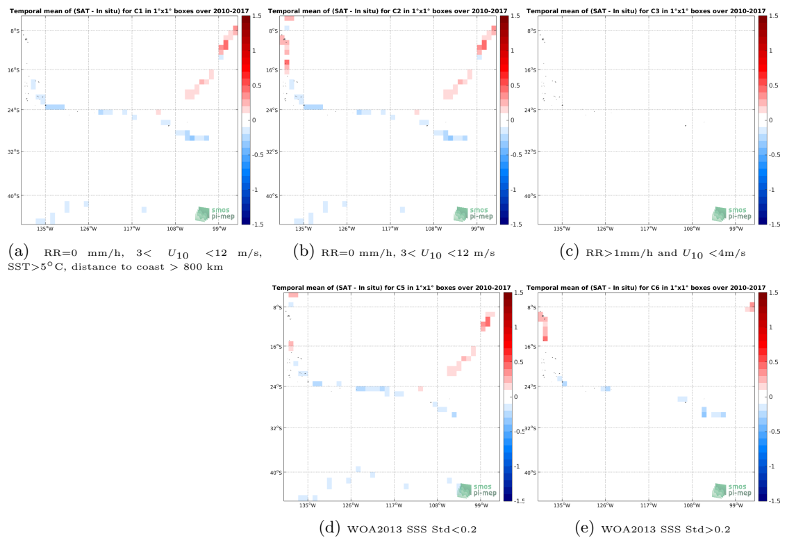
Figure 12: Temporal mean gridded over spatial boxes of size 1^\circ \times 1^\circ of \Delta SSS (CCI-L4-ESA-MERGED-OI-V1.8-30DAY-RUNNING - TSG-GOSUD-Sailing-ship) for 5 different subdatasets corresponding to:RR=0 mm/h, 3 < U_{10} < 12 m/s, SST >5^\circ\text{C} , distance to coast > 800 km (a), RR=0 mm/h, 3 < U_{10} < 12 m/s (b), RR >1 mm/h and U_{10} < 4 m/s (c), WOA2013 SSS Std <0.2 (d), WOA2013 SSS Std >0.2 (e).
