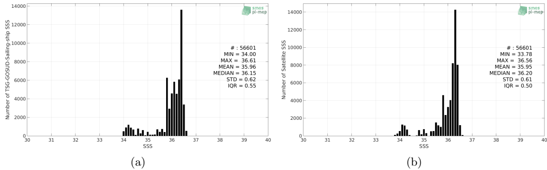
Figure 2: Histograms of SSS from TSG-GOSUD-Sailing-ship (a) and CCI-L4-ESA-MERGED-OI-V1.8-30DAY-RUNNING (b) considering all match-up pairs per bins of 0.1 over the OTT zone Pi-MEP region and for the full satellite product period.
