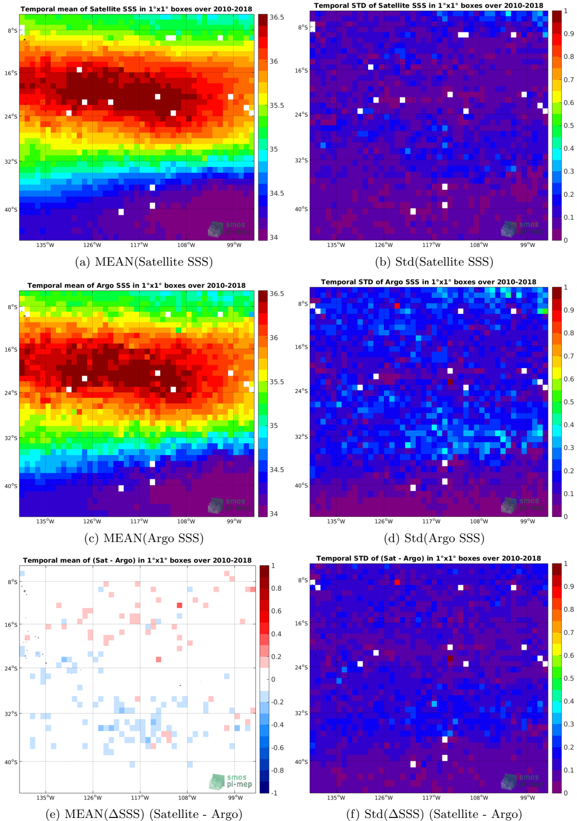
Figure 6: Temporal mean (left) and Std (right) of SSS from CCI-L4-ESA-MERGED-OI-V1.8-30DAY-RUNNING (top), Argo (middle), and of \Delta SSS (Satellite - Argo). Only match-up pairs are used to generate these maps.
