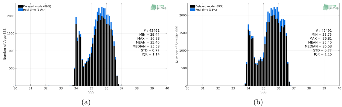
Figure 2: Histograms of SSS from Argo (a) and CCI-L4-ESA-MERGED-OI-V1.8-30DAY-RUNNING (b) considering all match-up pairs per bins of 0.1 over the OTT zone Pi-MEP region and for the full satellite product period.
