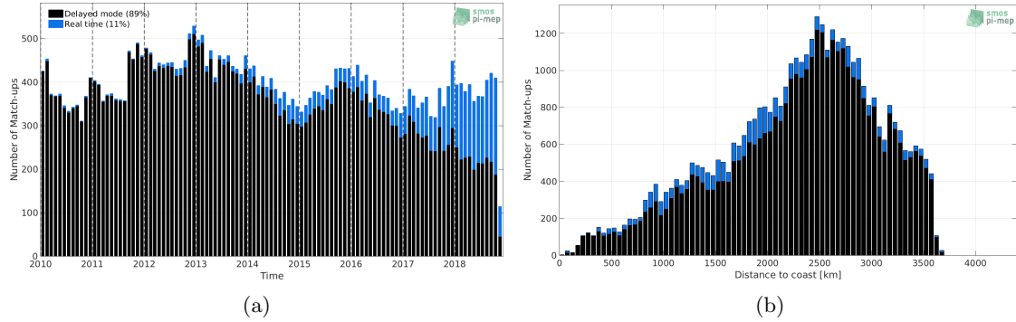
Figure 1: Number of match-ups between Argo and CCI-L4-ESA-MERGED-OI-V1.8-30DAY-RUNNING SSS as a function of time (a) and as function of the distance to coast (b) over the OTT zone Pi-MEP region and for the full satellite product period.
