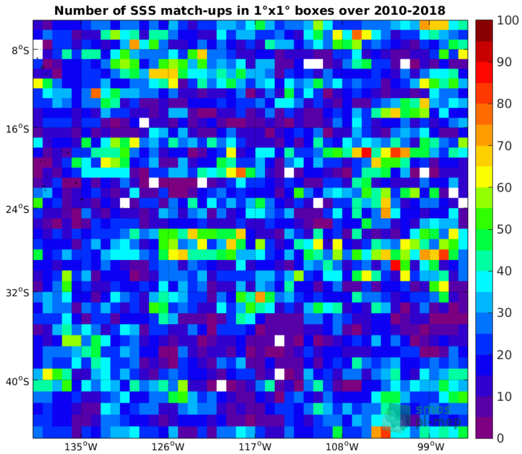
Figure 4: Number of SSS match-ups between Argo SSS and the CCI-L4-ESA-MERGED-OI-V1.8-30DAY-RUNNING SSS product for the OTT zone Pi-MEP region over 1°x1° boxes and for the full satellite product period.
