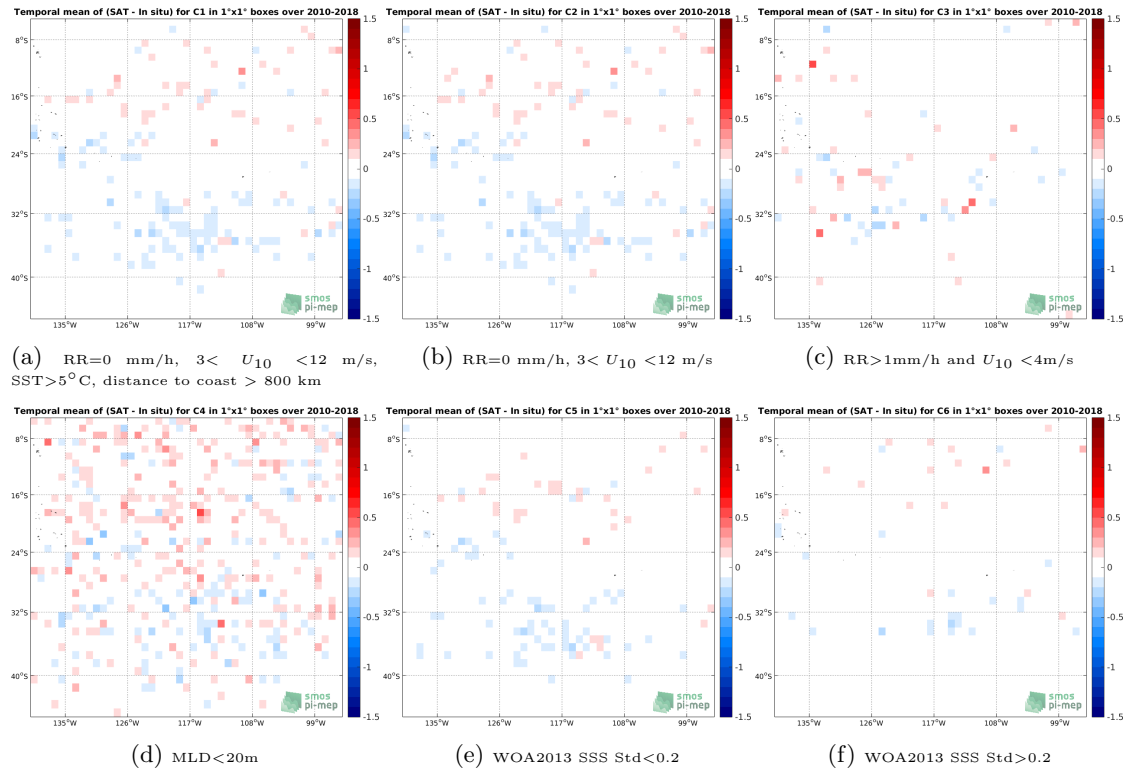
Figure 12: Temporal mean gridded over spatial boxes of size 1^\circ \times 1^\circ of \Delta SSS (CCI-L4-ESA-MERGED-OI-V1.8-30DAY-RUNNING - Argo) for 6 different subdatasets corresponding to:RR=0 mm/h, 3 < U_{10} < 12 m/s, SST >5^\circ C, distance to coast > 800 km (a), RR=0 mm/h, 3 < U_{10} < 12 m/s (b), RR >1 mm/h and U_{10} < 4 m/s (c),MLD <20 m (d),WOA2013 SSS Std <0.2 (e),WOA2013 SSS Std >0.2 (f).
