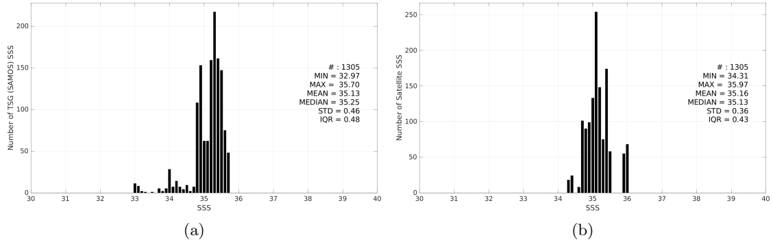
Figure 3: Histograms of SSS from TSG (SAMOS) (a) and Aquarius SSS L4 OI v5 - Weekly (IPRC) (b) considering all match-up pairs per bins of 0.1 over the OTT zone Pi-MEP region and for the full satellite product period.
