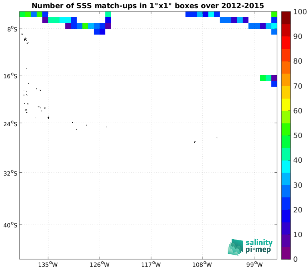
Figure 5: Number of SSS match-ups between TSG (SAMOS) SSS and the Aquarius SSS L4 OI v5 - Weekly (IPRC) SSS product for the OTT zone Pi-MEP region over 1^\circ \times 1^\circ boxes and for the full satellite product period.
