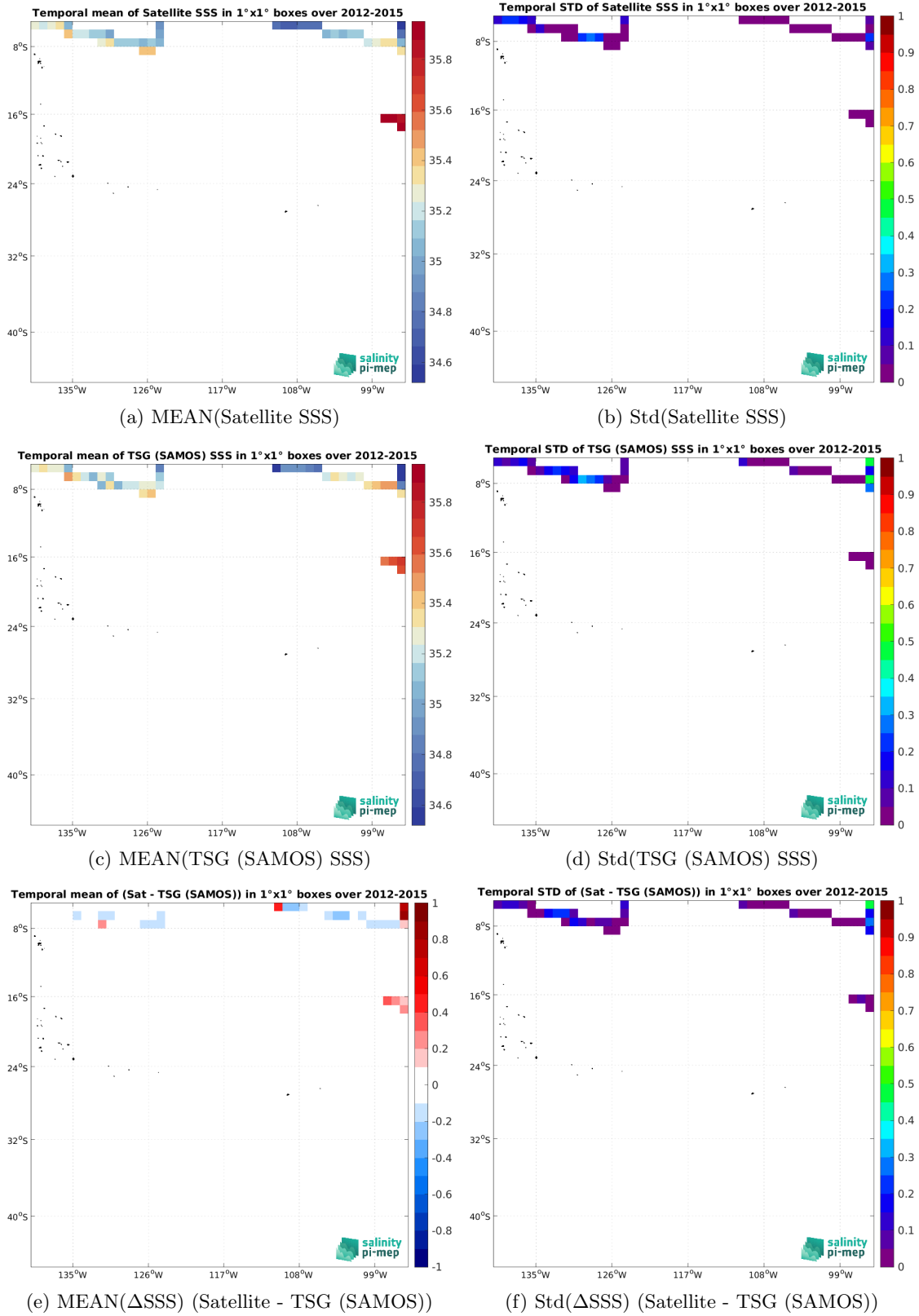
Figure 7: Temporal mean (left) and Std (right) of SSS from Aquarius SSS L4 OI v5 - Weekly (IPRC) (top), TSG (SAMOS) (middle), and of \Delta SSS (Satellite - TSG (SAMOS)). Only match-up pairs are used to generate these maps.
