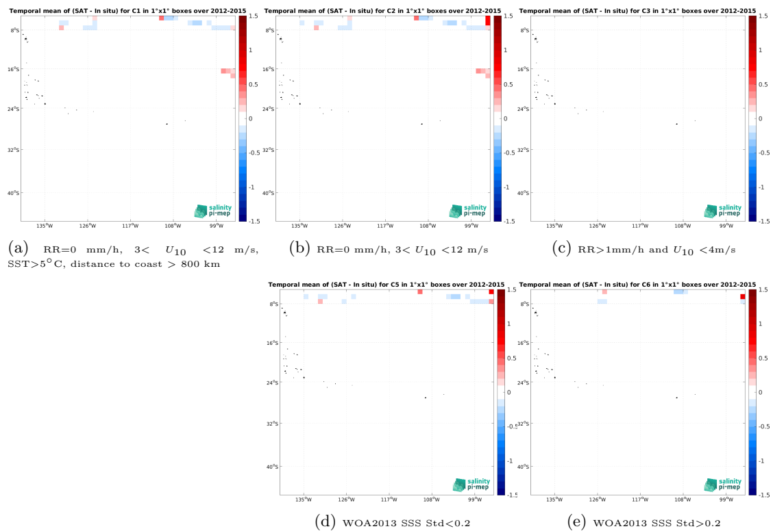
Figure 14: Temporal mean gridded over spatial boxes of size 1^\circ \times 1^\circ of \Delta SSS (Aquarius SSS L4 OI v5 - Weekly (IPRC) - TSG (SAMOS)) for 5 different subdatasets corresponding to: RR=0 mm/h, 3 < U_{10} < 12 m/s, SST > 5^\circ C , distance to coast > 800 km (a), RR=0 mm/h, 3 < U_{10} < 12 m/s (b), RR > 1 mm/h and U_{10} < 4 m/s (c), WOA2013 SSS Std < 0.2 (d), WOA2013 SSS Std > 0.2 (e).
