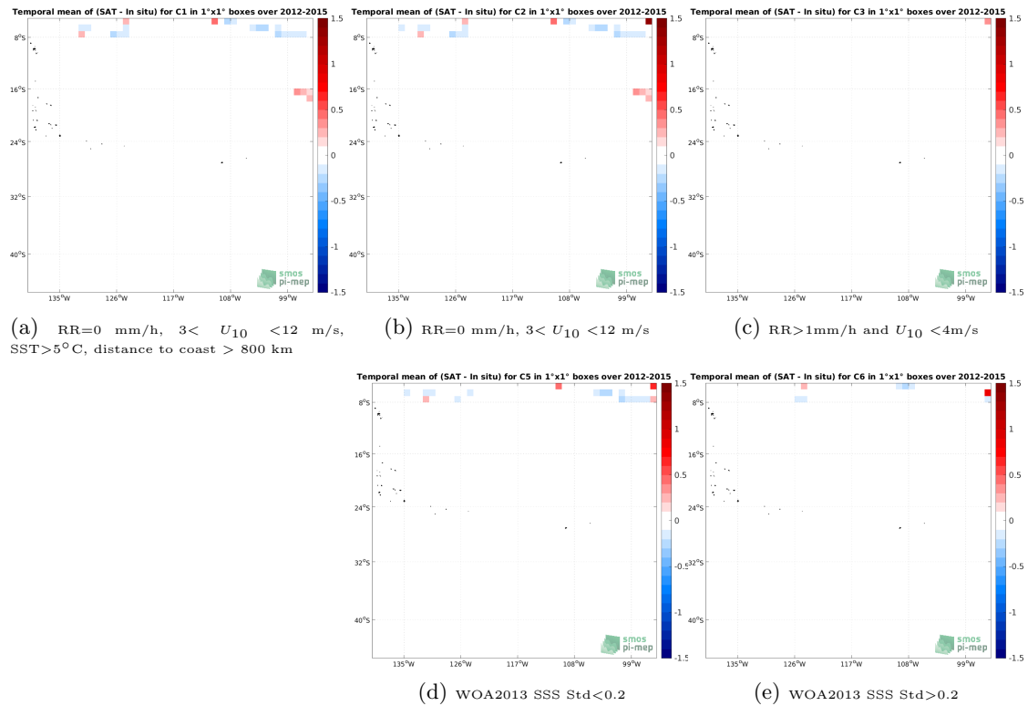
Figure 12: Temporal mean gridded over spatial boxes of size 1^\circ \times 1^\circ of \Delta SSS (Aquarius SSS L4 OI v5 - Weekly (IPRC) - TSG (SAMOS)) for 5 different subdatasets corresponding to:RR=0 mm/h, 3 < U_{10} < 12 m/s, SST >5^\circ C, distance to coast > 800 km (a), RR=0 mm/h, 3 < U_{10} < 12 m/s (b), RR >1 mm/h and U_{10} < 4 m/s (c), WOA2013 SSS Std <0.2 (d), WOA2013 SSS Std >0.2 (e).
