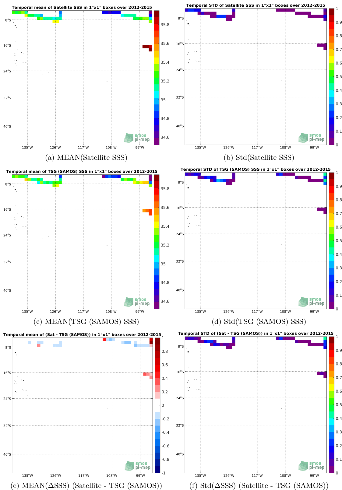
Figure 6: Temporal mean (left) and Std (right) of SSS from Aquarius SSS L4 OI v5 - Weekly (IPRC) (top), TSG (SAMOS) (middle), and of \Delta SSS (Satellite - TSG (SAMOS)). Only match-up pairs are used to generate these maps.
