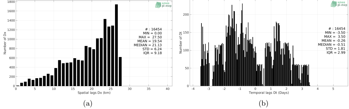
Figure 5: Histograms of the spatial (a) and temporal (b) lags between the time of the TSG (SAMOS) measurements and the date of the corresponding Aquarius SSS L4 OI v5 - Weekly (IPRC) SSS product.
