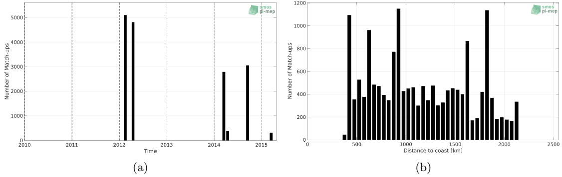
Figure 1: Number of match-ups between TSG (SAMOS) and Aquarius SSS L4 OI v5 - Weekly (IPRC) SSS as a function of time (a) and as function of the distance to coast (b) over the OTT zone Pi-MEP region and for the full satellite product period.
