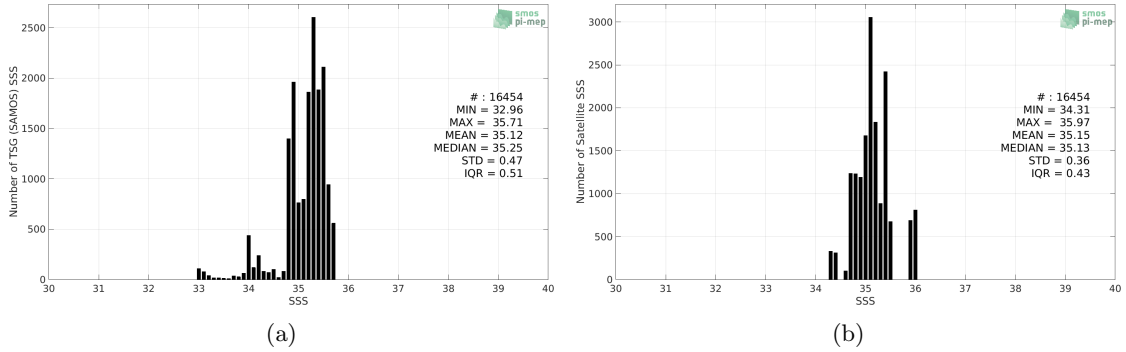
Figure 2: Histograms of SSS from TSG (SAMOS) (a) and Aquarius SSS L4 OI v5 - Weekly (IPRC) (b) considering all match-up pairs per bins of 0.1 over the OTT zone Pi-MEP region and for the full satellite product period.
