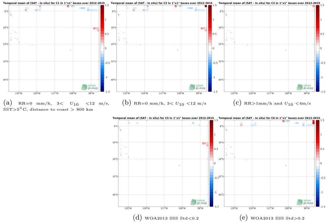
Figure 12: Temporal mean gridded over spatial boxes of size 1^\circ \times 1^\circ of \Delta SSS (Aquarius SSS L4 OI v5 - Weekly (IPRC) - TSG (SAMOS)) for 5 different subdatasets corresponding to: RR=0 mm/h, 3 < U_{10} < 12 m/s, SST>5°C, distance to coast > 800 km (a), RR=0 mm/h, 3 < U_{10} < 12 m/s (b), RR>1mm/h and U_{10} < 4 m/s (c), WOA2013 SSS Std<0.2 (d), WOA2013 SSS Std>0.2 (e).
