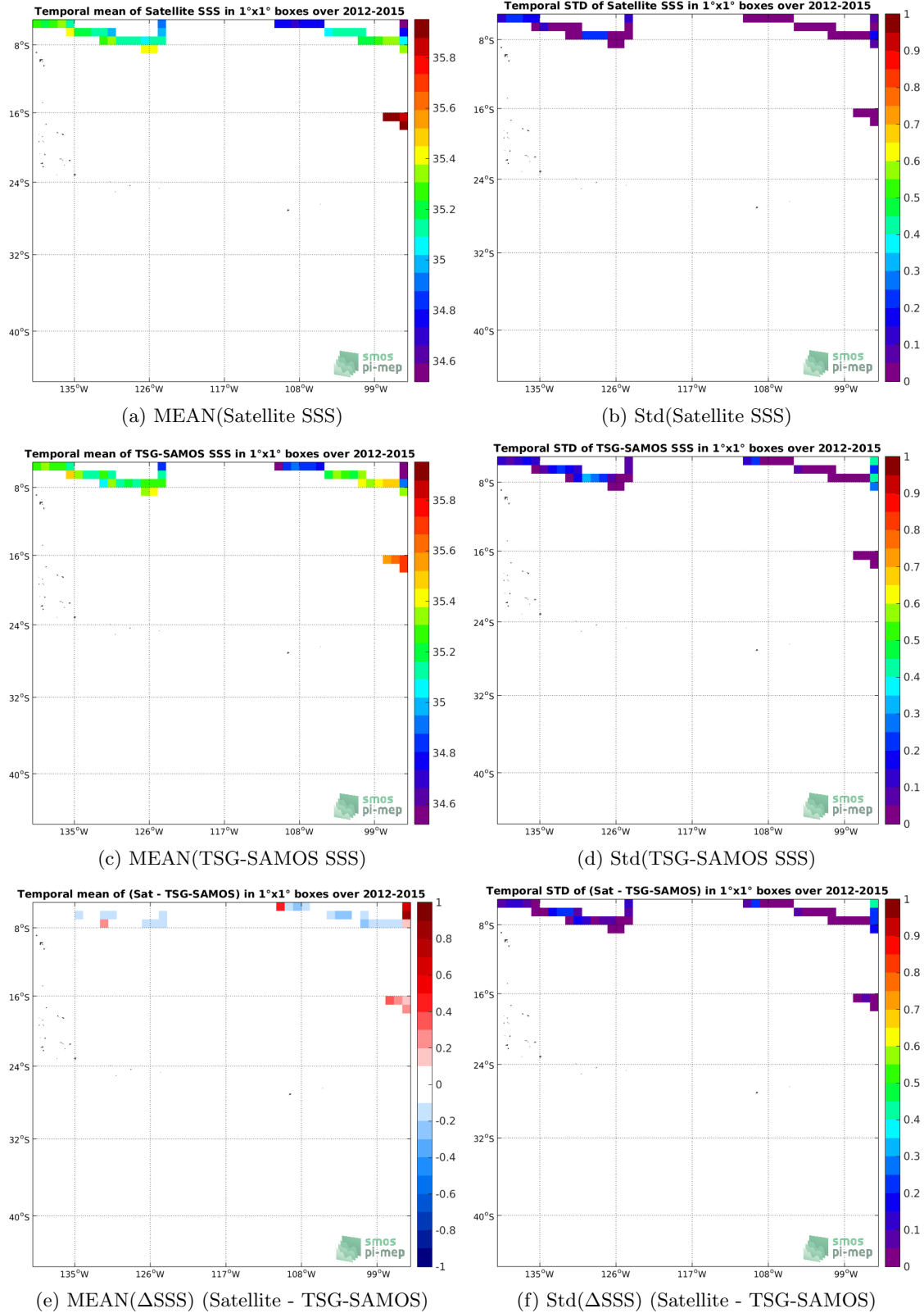
Figure 6: Temporal mean (left) and Std (right) of SSS from Aquarius-L4-IPRC-V5-WEEKLY (top), TSG-SAMOS (middle), and of \Delta SSS (Satellite - TSG-SAMOS). Only match-up pairs are used to generate these maps.
