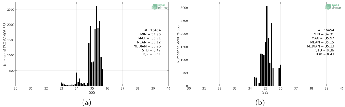
Figure 2: Histograms of SSS from TSG-SAMOS (a) and Aquarius-L4-IPRC-V5-WEEKLY (b) considering all match-up pairs per bins of 0.1 over the OTT zone Pi-MEP region and for the full satellite product period.
