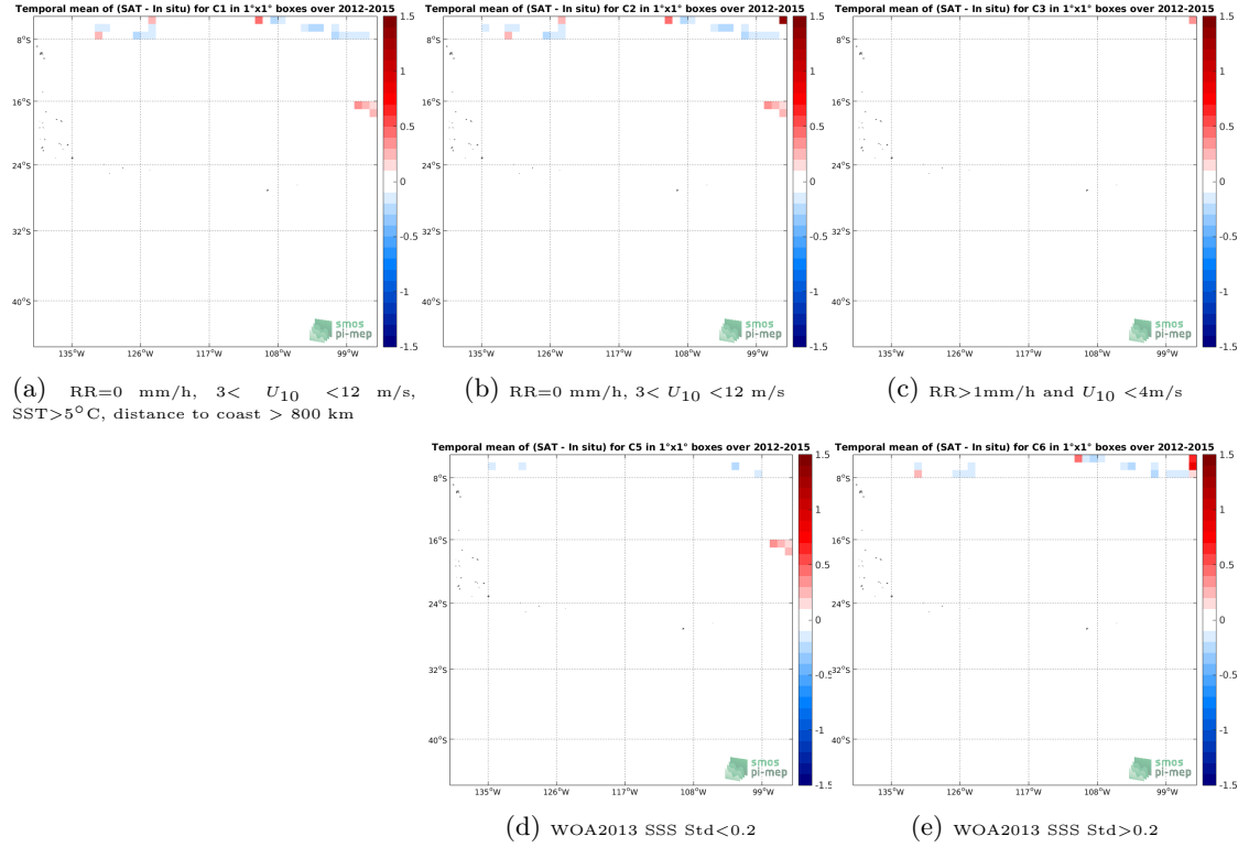
Figure 12: Temporal mean gridded over spatial boxes of size 1^\circ \times 1^\circ of \Delta SSS (Aquarius-L4-IPRC-V5-WEEKLY - TSG-SAMOS) for 5 different subdatasets corresponding to:RR=0 mm/h, 3 < U_{10} < 12 m/s, SST >5^\circ\text{C} , distance to coast > 800 km (a), RR=0 mm/h, 3 < U_{10} < 12 m/s (b), RR >1 mm/h and U_{10} < 4 m/s (c), WOA2013 SSS Std <0.2 (d), WOA2013 SSS Std >0.2 (e).
