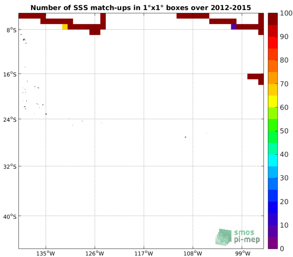
Figure 4: Number of SSS match-ups between TSG-SAMOS SSS and the Aquarius-L4-IPRC-V5-WEEKLY SSS product for the OTT zone Pi-MEP region over 1°x1° boxes and for the full satellite product period.
