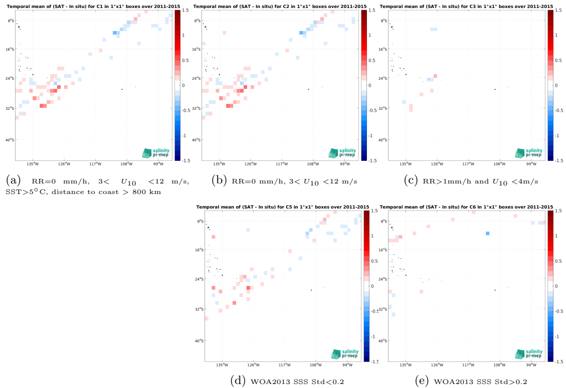
Figure 12: Temporal mean gridded over spatial boxes of size 1^\circ \times 1^\circ of \Delta SSS (Aquarius SSS L4 OI v5 - Weekly (IPRC) - TSG (LEGOS-DM)) for 5 different subdatasets corresponding to: RR=0 mm/h, 3 < U_{10} < 12 m/s, SST > 5^\circ C , distance to coast > 800 km (a), RR=0 mm/h, 3 < U_{10} < 12 m/s (b), RR > 1 mm/h and U_{10} < 4 m/s (c), WOA2013 SSS Std < 0.2 (d), WOA2013 SSS Std > 0.2 (e).
