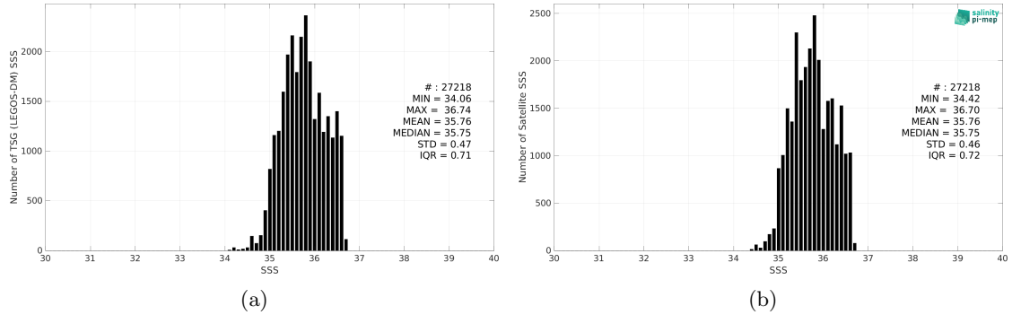
Figure 2: Histograms of SSS from TSG (LEGOS-DM) (a) and Aquarius SSS L4 OI v5 - Weekly (IPRC) (b) considering all match-up pairs per bins of 0.1 over the OTT zone Pi-MEP region and for the full satellite product period.
