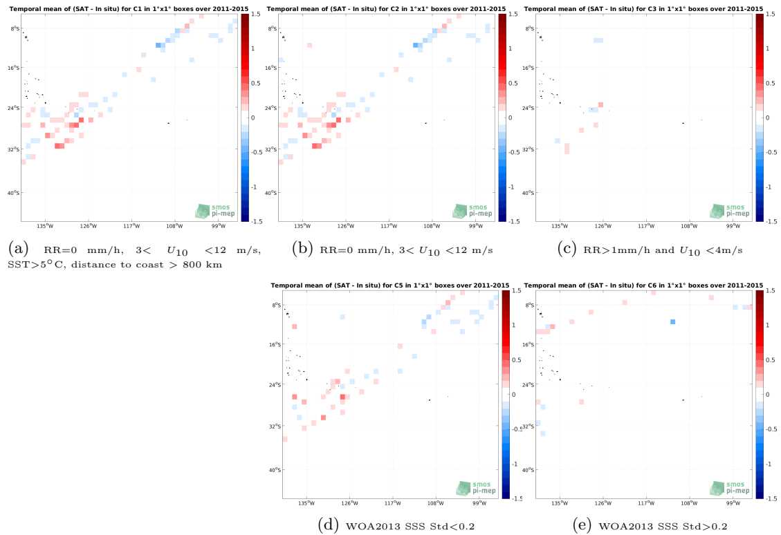
Figure 12: Temporal mean gridded over spatial boxes of size 1^\circ \times 1^\circ of \Delta SSS (Aquarius SSS L4 OI v5 - Weekly (IPRC) - TSG (LEGOS-DM)) for 5 different subdatasets corresponding to:RR=0 mm/h, 3 < U_{10} < 12 m/s, SST >5^\circ C, distance to coast > 800 km (a), RR=0 mm/h, 3 < U_{10} < 12 m/s (b), RR >1 mm/h and U_{10} < 4 m/s (c), WOA2013 SSS Std <0.2 (d), WOA2013 SSS Std >0.2 (e).
