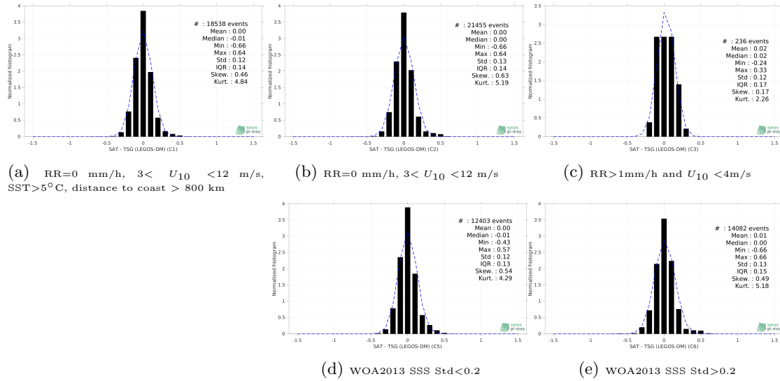
Figure 13: Normalized histogram of \Delta SSS (Aquarius SSS L4 OI v5 - Weekly (IPRC) - TSG (LEGOS-DM)) for 5 different subdatasets corresponding to: RR=0 mm/h, 3 < U_{10} < 12 m/s, SST >5^{\circ}\text{C} , distance to coast > 800 km (a), RR=0 mm/h, 3 < U_{10} < 12 m/s (b), RR >1 mm/h and U_{10} < 4 m/s (c), WOA2013 SSS Std <0.2 (d), WOA2013 SSS Std >0.2 (e).
