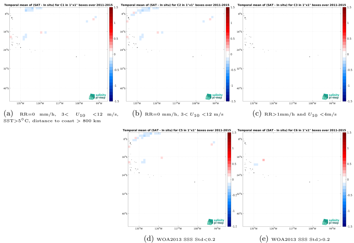
Figure 14: Temporal mean gridded over spatial boxes of size 1^\circ \times 1^\circ of \Delta\text{SSS} (Aquarius SSS L4 OI v5 - Weekly (IPRC) - TSG (GOSUD-Research-vessel)) for 5 different subdatasets corresponding to:RR=0 mm/h, 3 < U_{10} < 12 m/s, SST >5^\circ\text{C} , distance to coast > 800 km (a), RR=0 mm/h, 3 < U_{10} < 12 m/s (b), RR >1 mm/h and U_{10} < 4 m/s (c), WOA2013 SSS Std <0.2 (d), WOA2013 SSS Std >0.2 (e).
