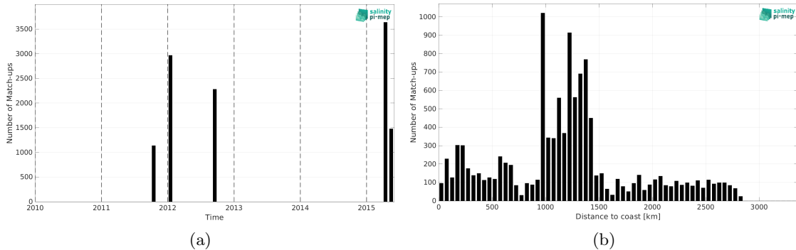
Figure 2: Number of match-ups between TSG (GOSUD-Research-vessel) and Aquarius SSS L4 OI v5 - Weekly (IPRC) SSS as a function of time (a) and as function of the distance to coast (b) over the OTT zone Pi-MEP region and for the full satellite product period.
