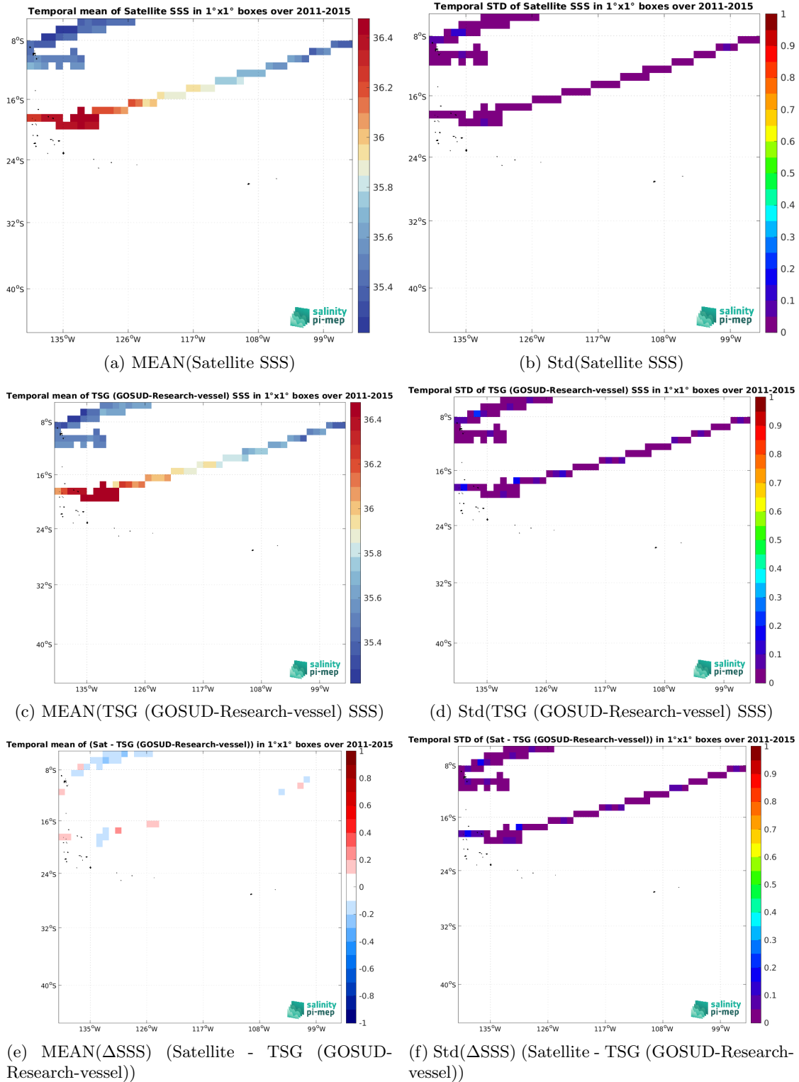
Figure 7: Temporal mean (left) and Std (right) of SSS from Aquarius SSS L4 OI v5 - Weekly (IPRC) (top), TSG (GOSUD-Research-vessel) (middle), and of \Delta SSS (Satellite - TSG (GOSUD-Research-vessel)). Only match-up pairs are used to generate these maps.
