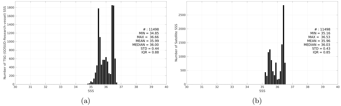
Figure 3: Histograms of SSS from TSG (GOSUD-Research-vessel) (a) and Aquarius SSS L4 OI v5 - Weekly (IPRC) (b) considering all match-up pairs per bins of 0.1 over the OTT zone Pi-MEP region and for the full satellite product period.
