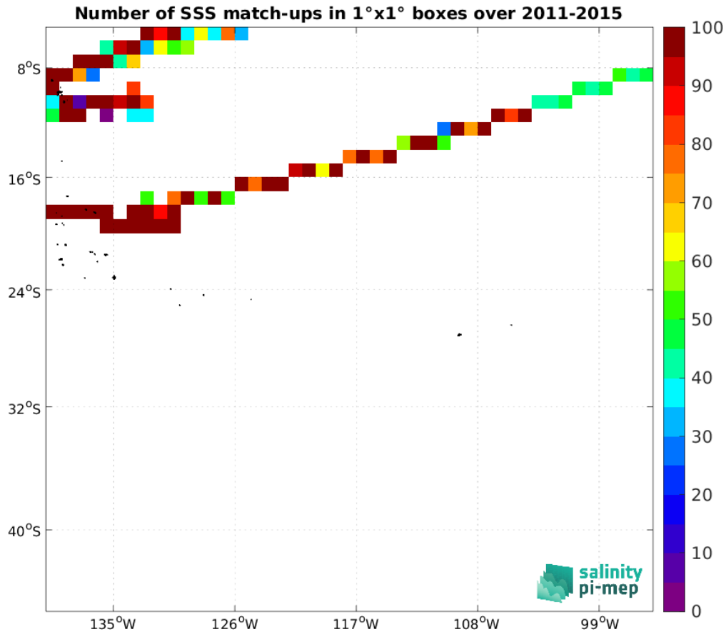
Figure 5: Number of SSS match-ups between TSG (GOSUD-Research-vessel) SSS and the Aquarius SSS L4 OI v5 - Weekly (IPRC) SSS product for the OTT zone Pi-MEP region over 1^\circ \times 1^\circ boxes and for the full satellite product period.
