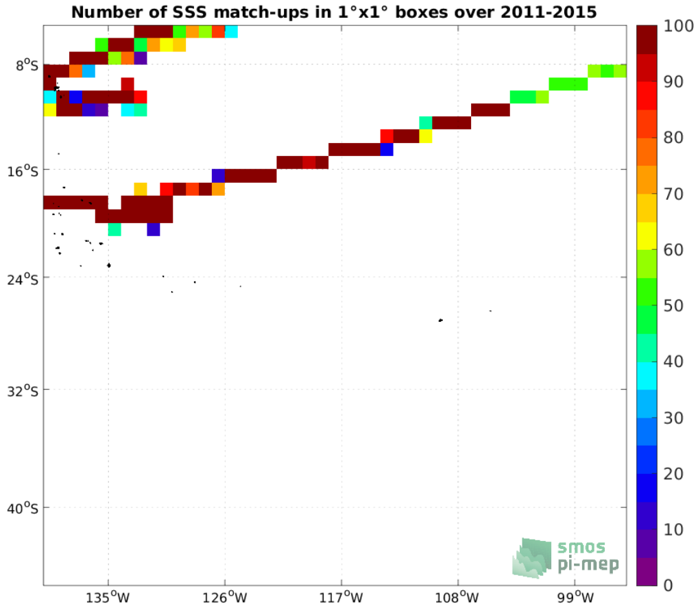
Figure 4: Number of SSS match-ups between TSG (GOSUD-Research-vessel) SSS and the Aquarius SSS L4 OI v5 - Weekly (IPRC) SSS product for the OTT zone Pi-MEP region over 1^\circ \times 1^\circ boxes and for the full satellite product period.
