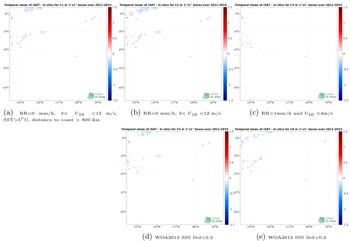
Figure 12: Temporal mean gridded over spatial boxes of size 1^\circ \times 1^\circ of \Delta SSS (Aquarius SSS L4 OI v5 - Weekly (IPRC) - TSG (GOSUD-Research-vessel)) for 5 different subdatasets corresponding to:RR=0 mm/h, 3 < U_{10} < 12 m/s, SST>5°C, distance to coast > 800 km (a), RR=0 mm/h, 3 < U_{10} < 12 m/s (b), RR>1mm/h and U_{10} < 4 m/s (c), WOA2013 SSS Std<0.2 (d), WOA2013 SSS Std>0.2 (e).
