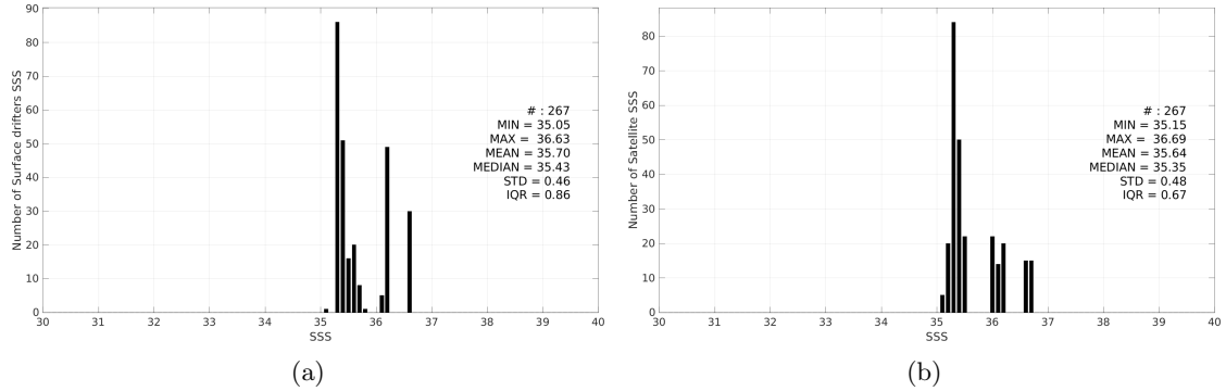
Figure 3: Histograms of SSS from Surface drifters (a) and Aquarius SSS L4 OI v5 - Weekly (IPRC) (b) considering all match-up pairs per bins of 0.1 over the OTT zone Pi-MEP region and for the full satellite product period.
