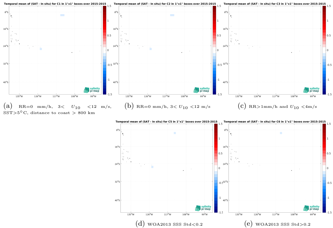
Figure 13: Temporal mean gridded over spatial boxes of size 1^\circ \times 1^\circ of \Delta SSS (Aquarius SSS L4 OI v5 - Weekly (IPRC) - Surface drifters) for 5 different subdatasets corresponding to:RR=0 mm/h, 3 < U_{10} < 12 m/s, SST >5^\circ C, distance to coast > 800 km (a), RR=0 mm/h, 3 < U_{10} < 12 m/s (b), RR >1 mm/h and U_{10} < 4 m/s (c), WOA2013 SSS Std <0.2 (d), WOA2013 SSS Std >0.2 (e).
