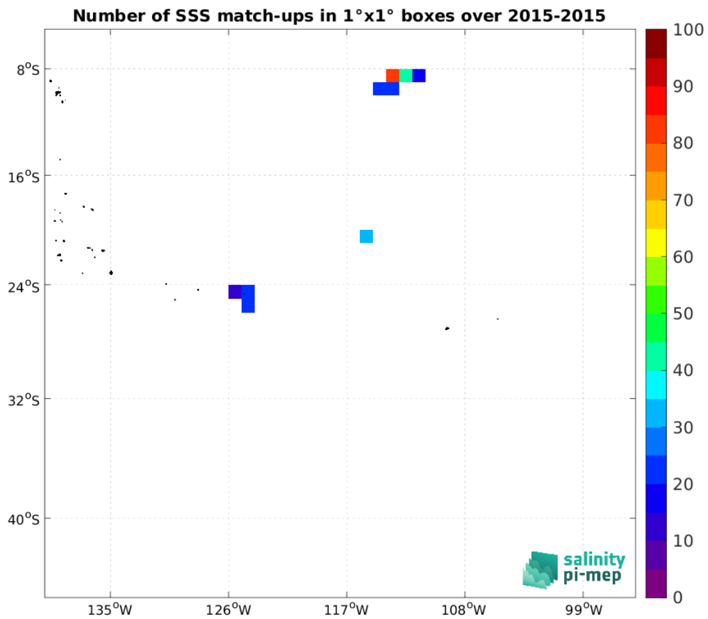
Figure 4: Number of SSS match-ups between Surface drifters SSS and the Aquarius SSS L4 OI v5 - Weekly (IPRC) SSS product for the OTT zone Pi-MEP region over 1°x1° boxes and for the full satellite product period.
