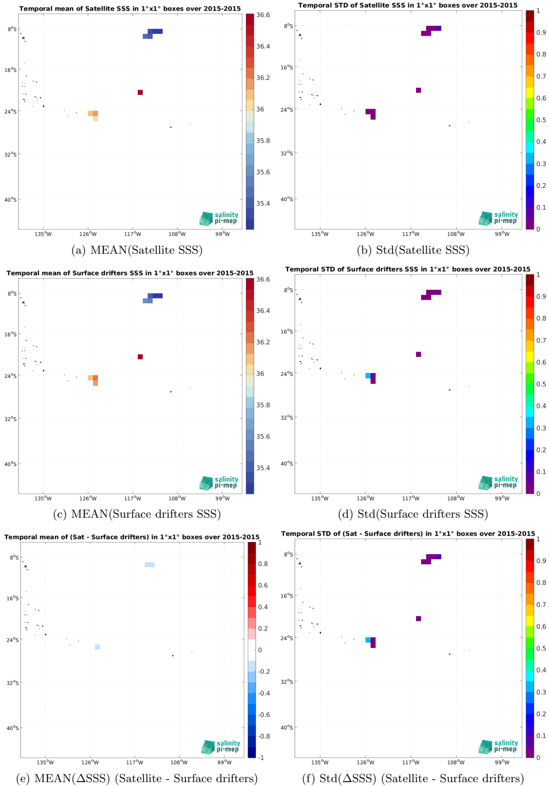
Figure 6: Temporal mean (left) and Std (right) of SSS from Aquarius SSS L4 OI v5 - Weekly (IPRC) (top), Surface drifters (middle), and of \Delta SSS (Satellite - Surface drifters). Only match-up pairs are used to generate these maps.
