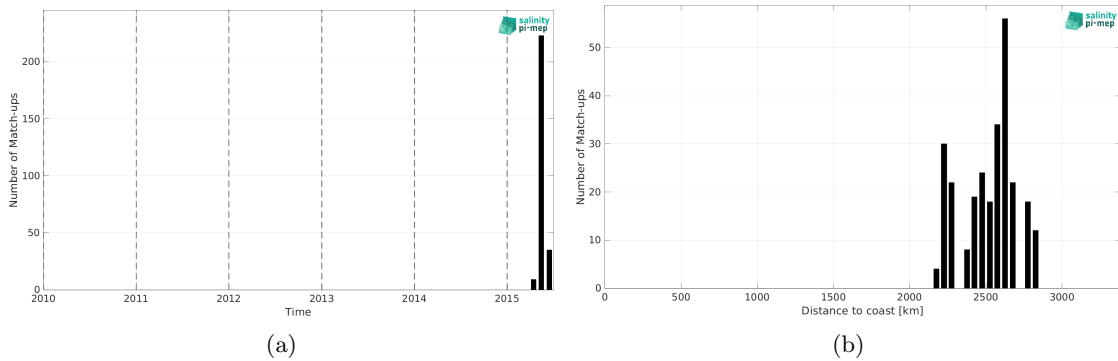
Figure 2: Number of match-ups between Surface drifters and Aquarius SSS L4 OI v5 - Weekly (IPRC) SSS as a function of time (a) and as function of the distance to coast (b) over the OTT zone Pi-MEP region and for the full satellite product period.
